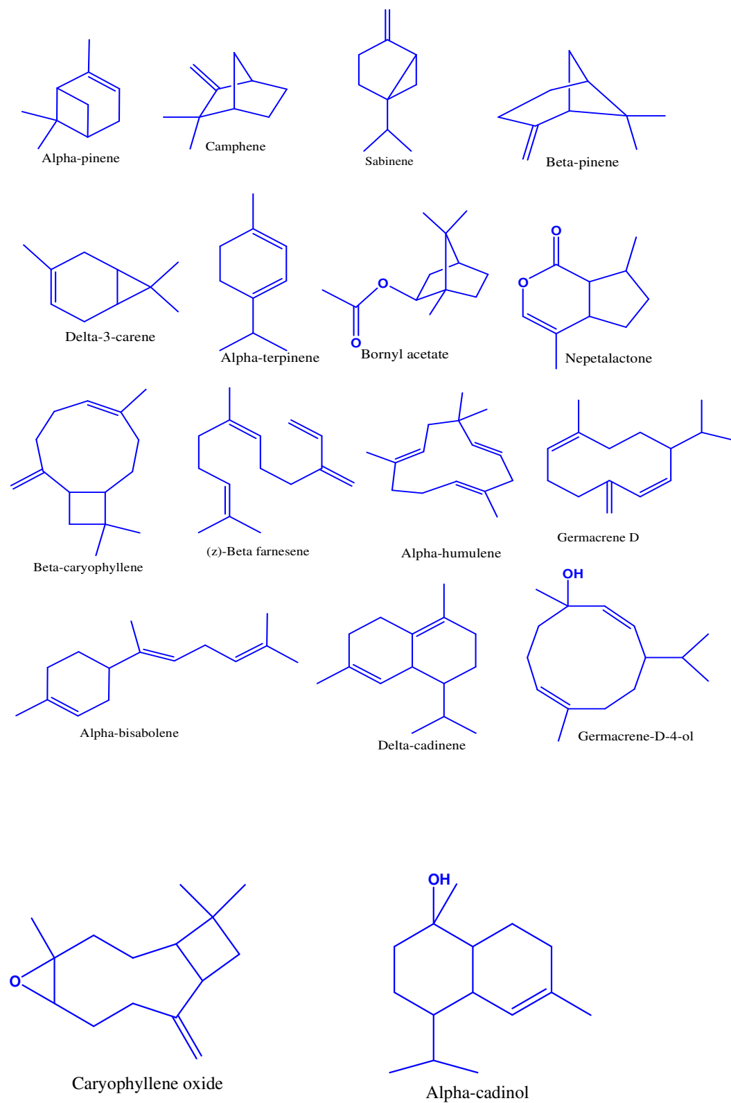
Figure-2: Chemical structures of the mono and sesquiterpene compounds present in the essential oil of Nepeta raphanorhiza
