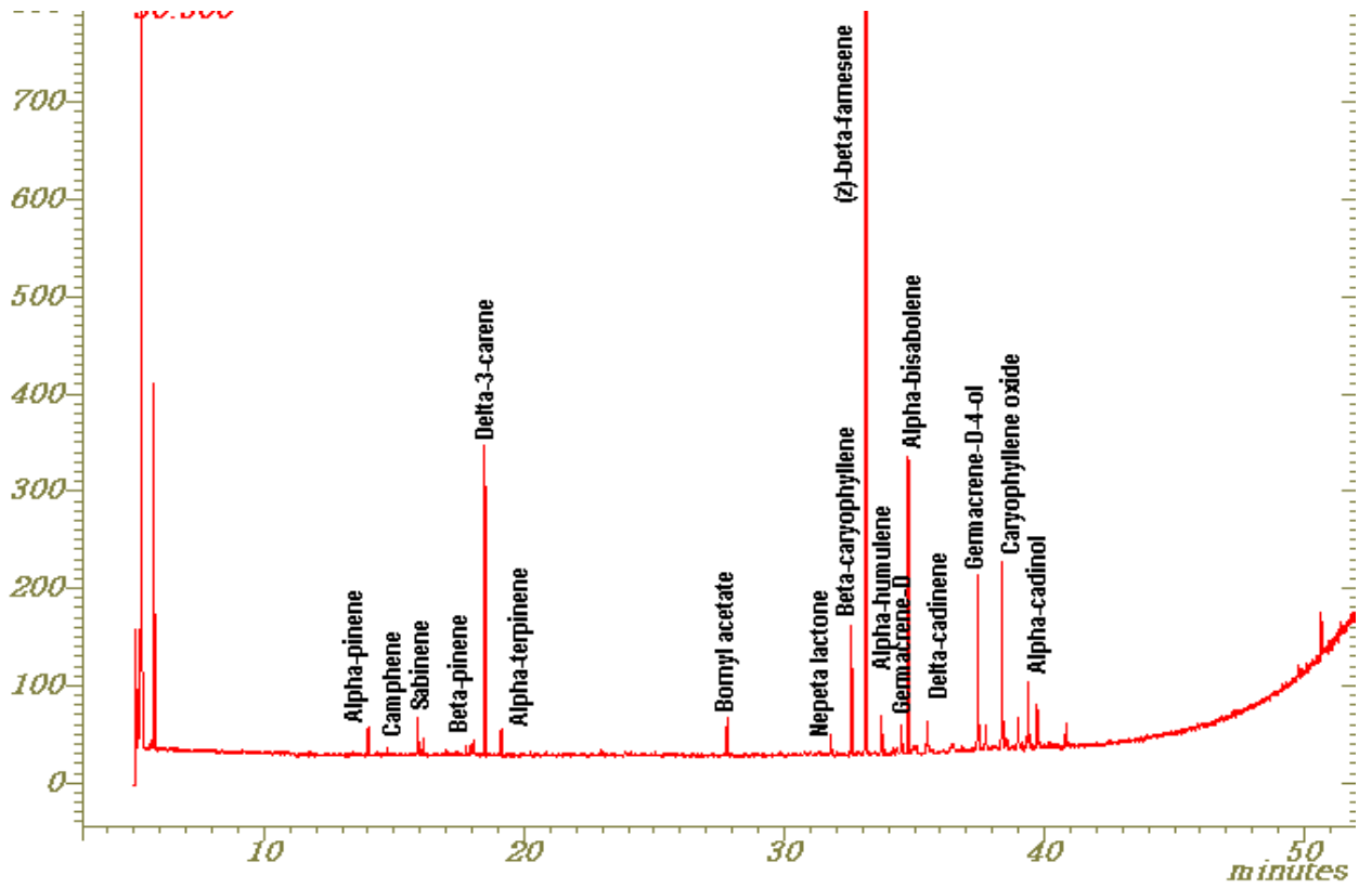
Figure-1: Total ion chromatogram (TIC) of the essential oil of Nepeta raphanorrhiza growing in Kashmir valley.
