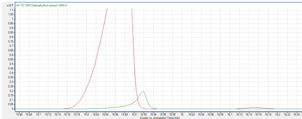
S5: Expansion of the selected ion chromatograms of the ions at m/z 136 - terpinolene (red) and m/z 132 - p -cymenene (green).
