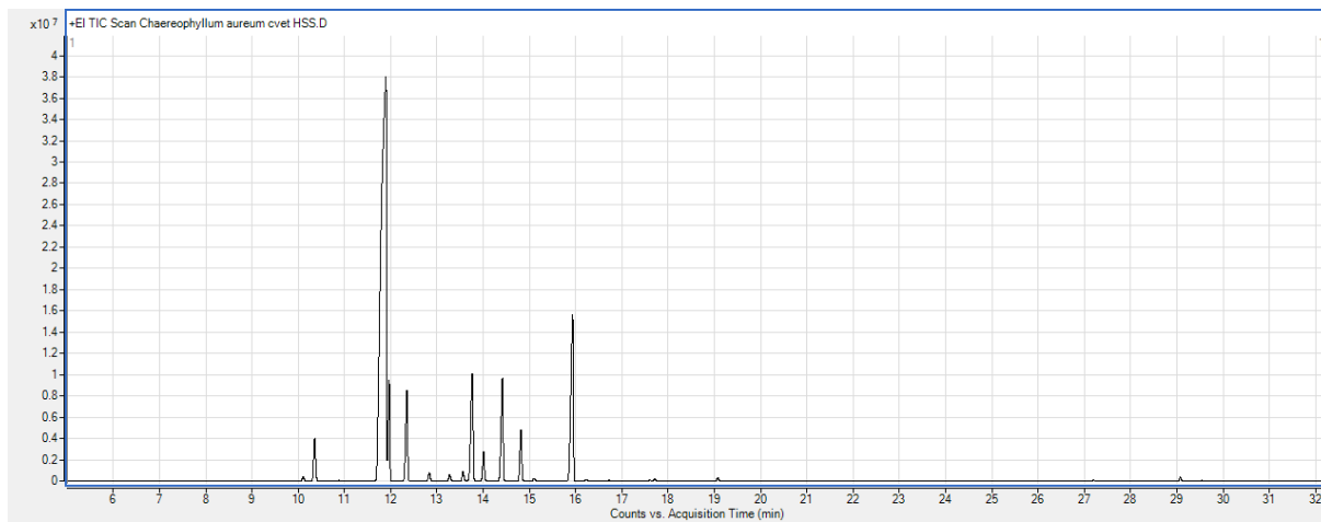
S3: Total ion chromatogram of the Chaerophyllum aureum L. flower headspace volatiles.
