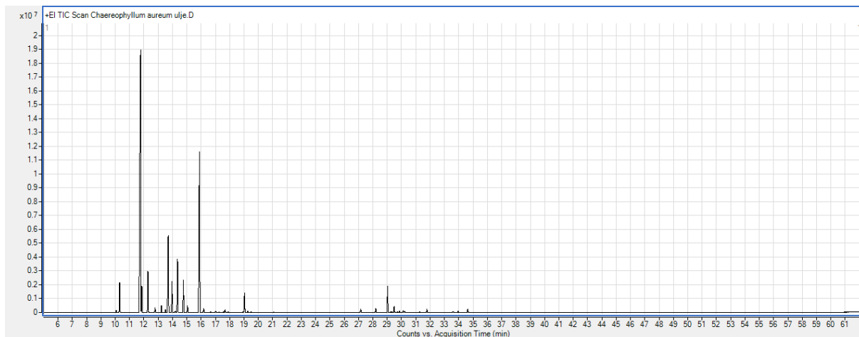
S1: Total ion chromatogram of the Chaerophyllum aureum L. essential oil.
