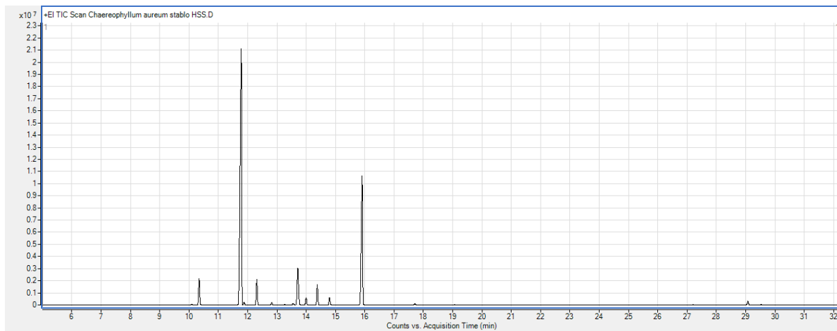
S2: Total ion chromatogram of the Chaerophyllum aureum L. stem headspace volatiles.
