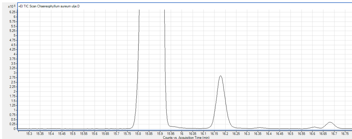
S4: Expansion of the total ion chromatogram of the Chaerophyllum aureum L. essential oil.
