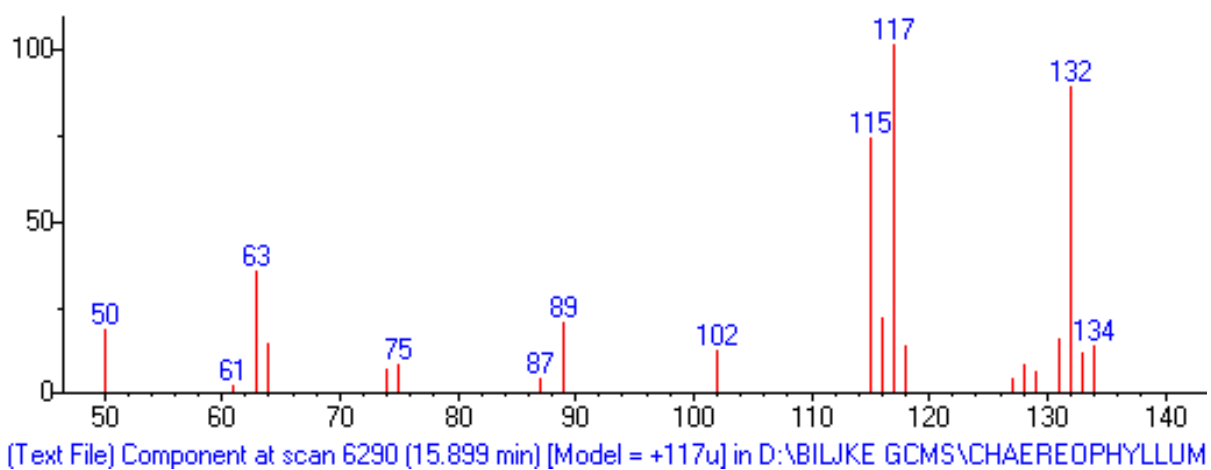
S7: Mass spectrum of p -cymenene obtained by AMDIS software.
