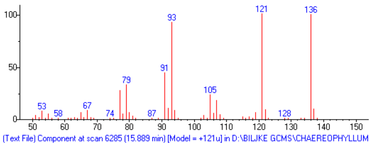
S6: Mass spectrum of terpinolene obtained by AMDIS software.
