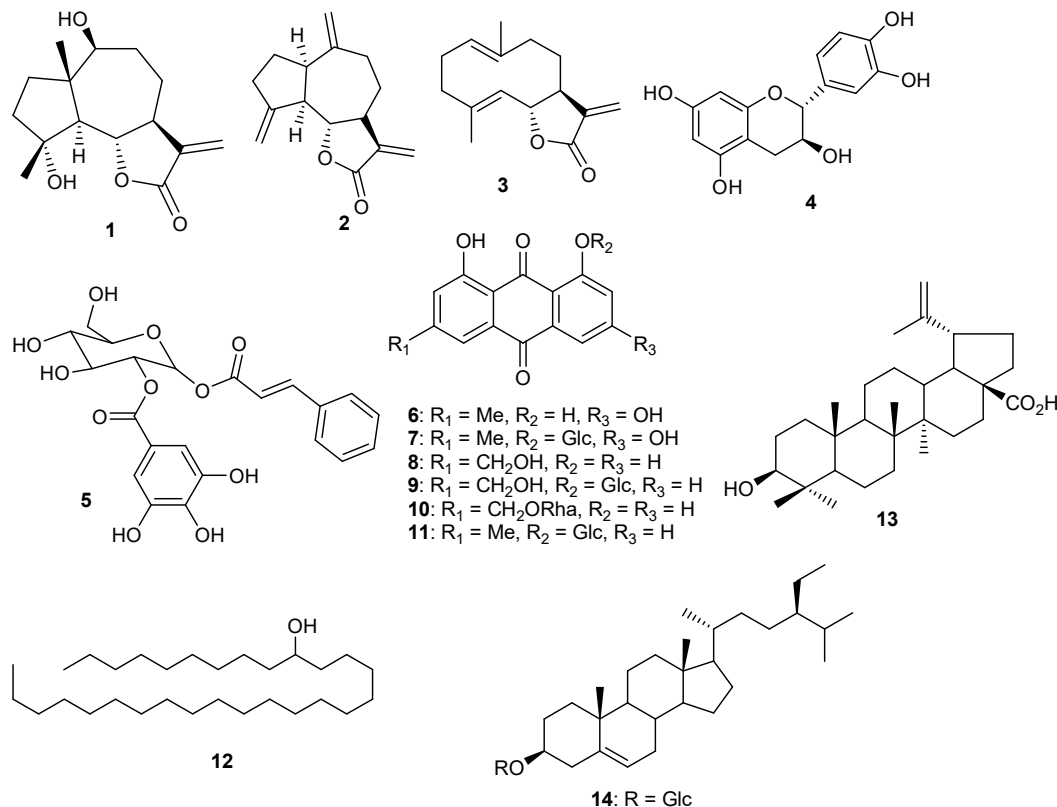
Figure 1. Compounds 1-14 isolated from L. shawii
