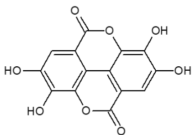
Ellagic acid
