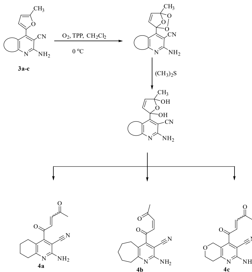
Scheme 2. Photooxygenation of 4-furyl-2-amino-3-cyanopyridine derivatives
