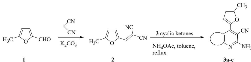
Scheme 1. Synthesis of 4-furyl-2-amino-3-cyanopyridine derivatives ( 3 cyclic ketones: cyclohexanone; cycloheptanone; tetrahydro-4H-pyran-4-one).
