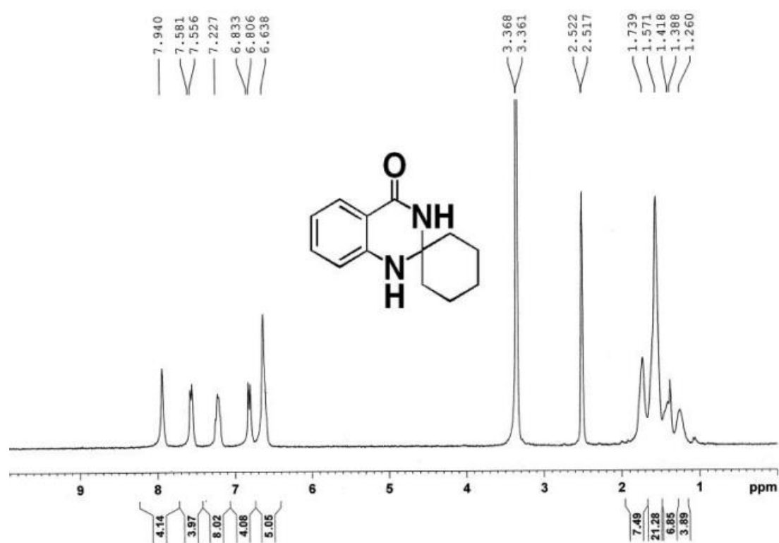
Figure S24: 1 H-NMR (400 MHz, CDCl 3 ) Spectrum of 3l
