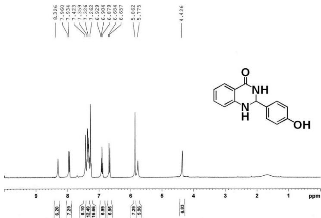
Figure S12: 1 H-NMR (400 MHz, CDCl 3 ) Spectrum of 3e
