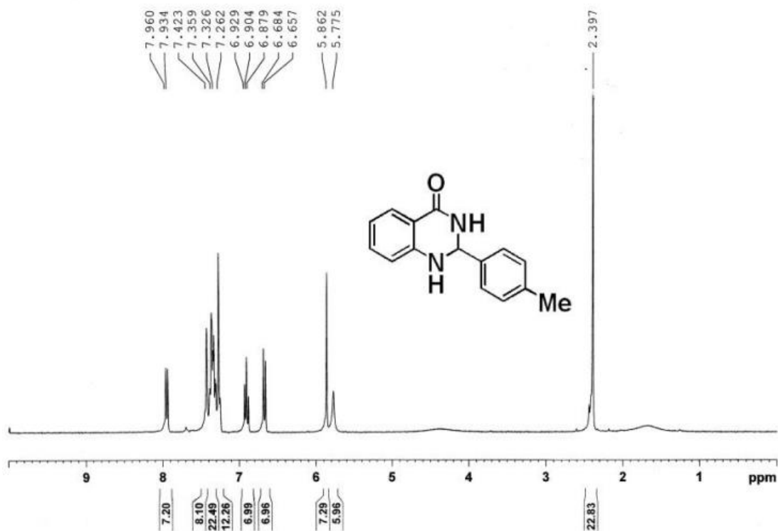
Figure S4: 1 H-NMR (400 MHz, CDCl 3 ) Spectrum of 3b
