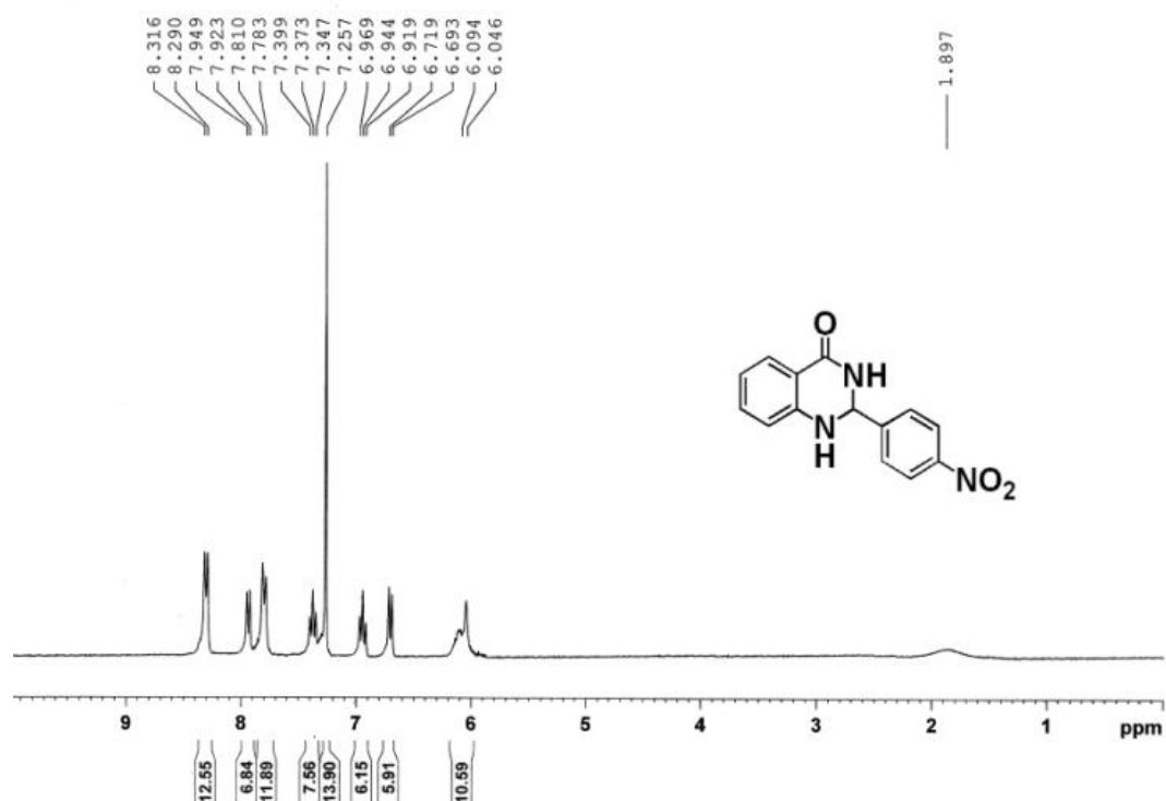
Figure S14: 1 H-NMR (400 MHz, CDCl 3 ) Spectrum of 3f
