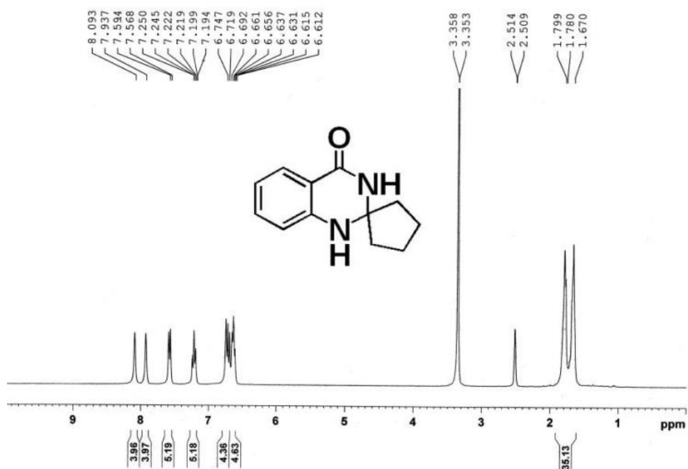
Figure S27: 1 H-NMR (400 MHz, CDCl 3 ) Spectrum of 3m
