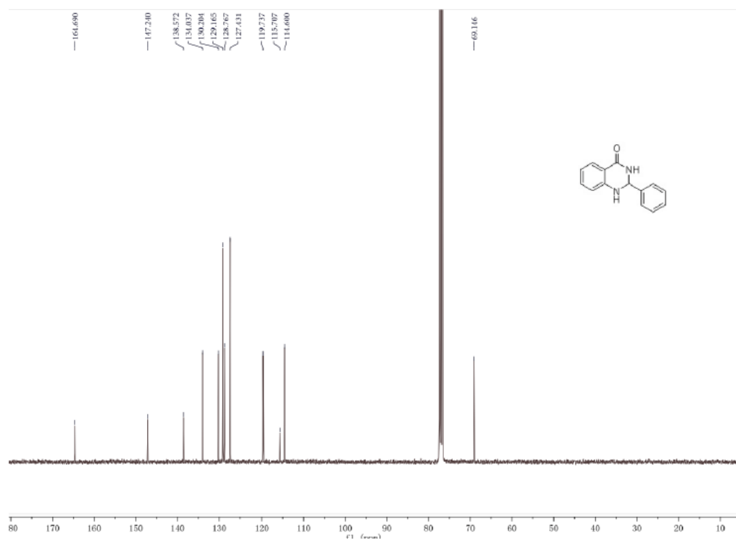
Figure S3: 13 C-NMR (100 MHz, CDCl 3 ) Spectrum of 3a
