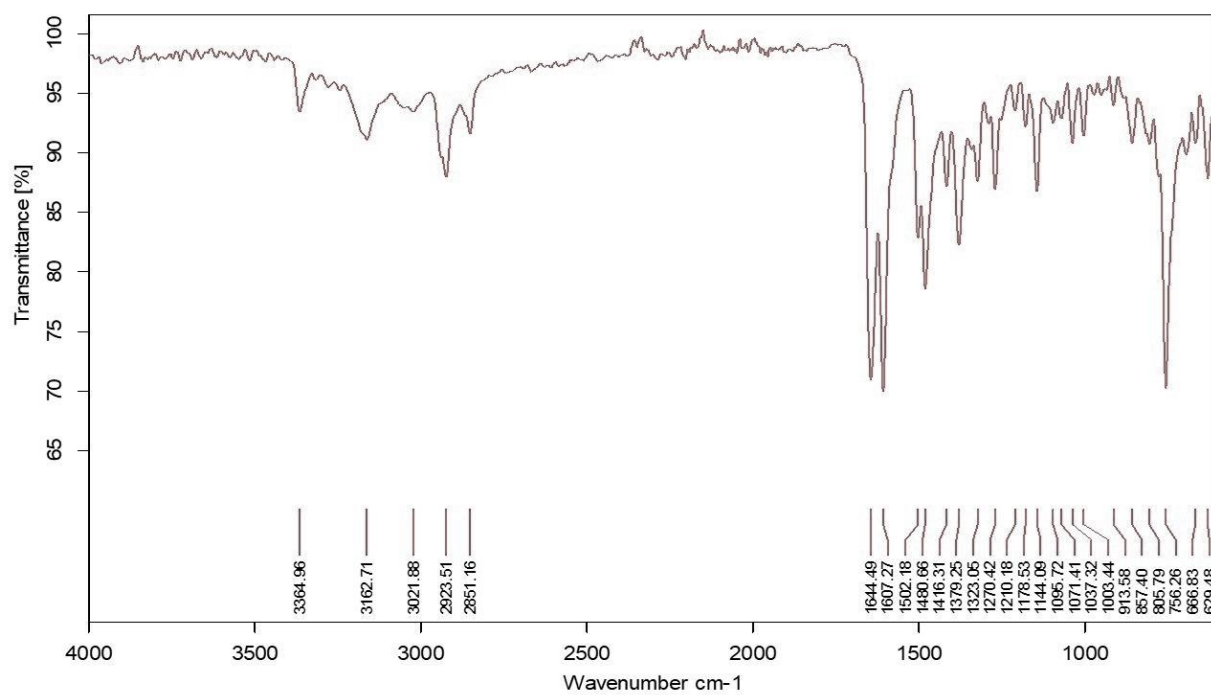
Figure S23: IR Spectrum of 3l
