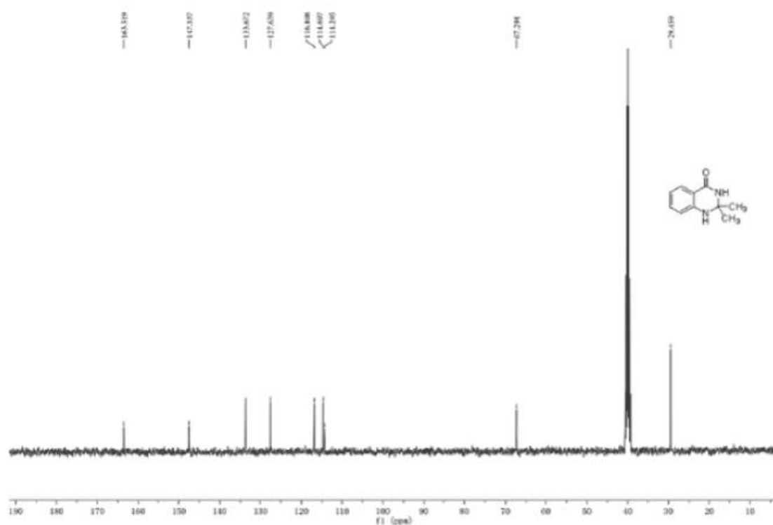
Figure S19: 13 C-NMR (100 MHz, CDCl 3 ) Spectrum of 3i
