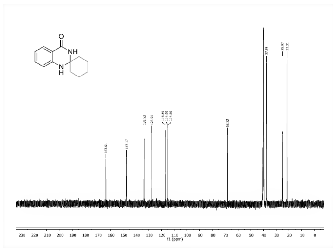
Figure S25: ^{13}\text{C} -NMR (100 MHz, \text{CDCl}_3 ) Spectrum of 3l
