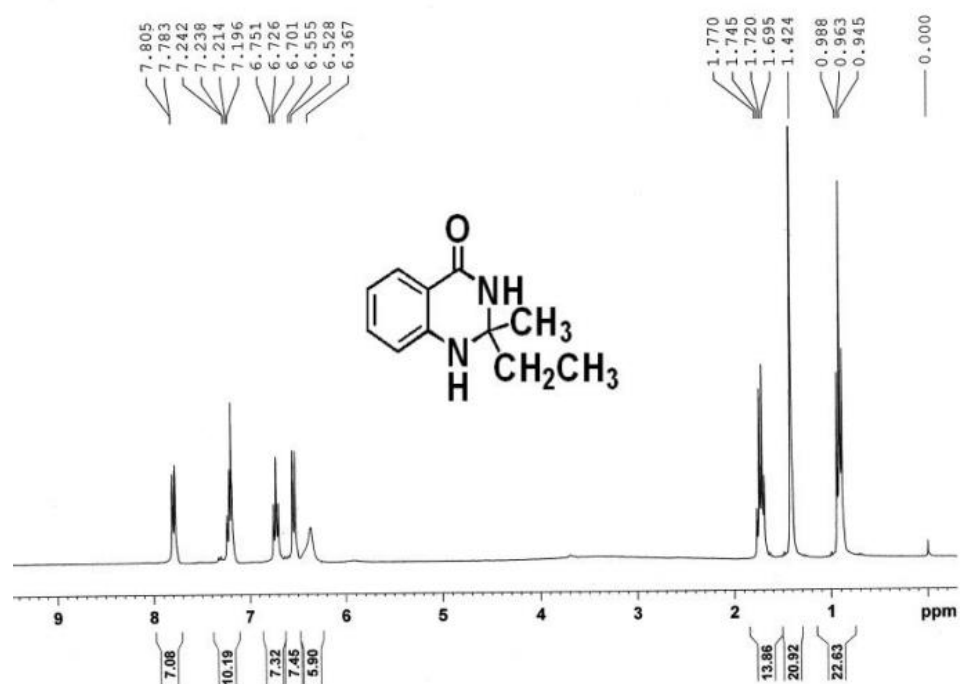
Figure S20: 1 H-NMR (400 MHz, CDCl 3 ) Spectrum of 3j
