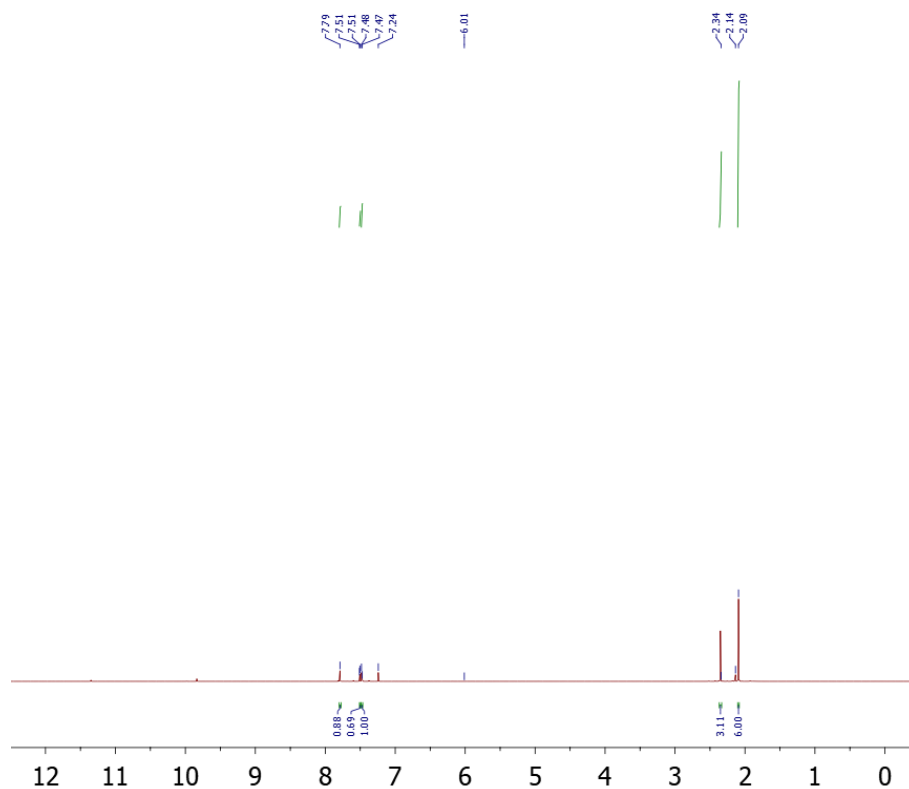
Figure S7 : ^1\text{H} NMR spectrum of compound 15
