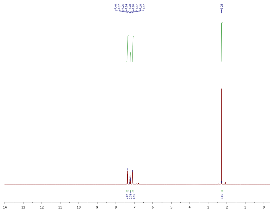
Figure S1: ^1\text{H} NMR spectrum of compound 1
