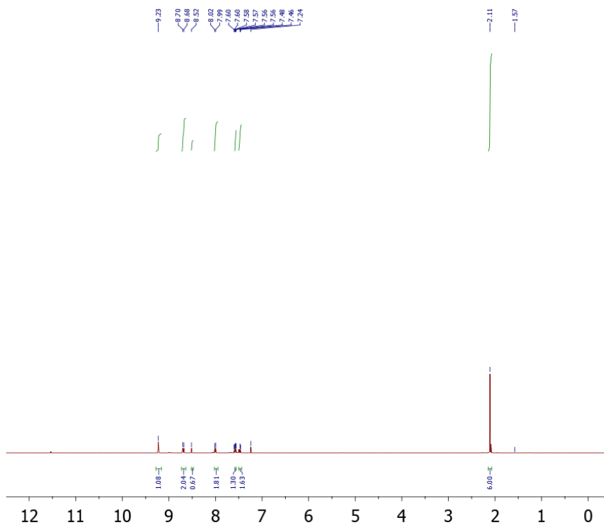
Figure S9 : ^1\text{H} NMR spectrum of compound 17
