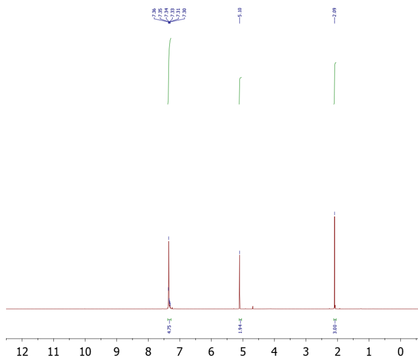
Figure S3 : ^1\text{H} NMR spectrum of compound 5
