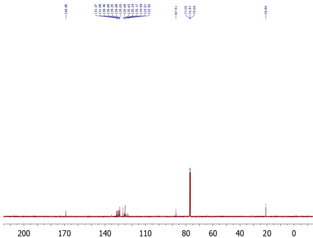
Figure S8 : ^{13}\text{C} NMR spectrum of compound 17
