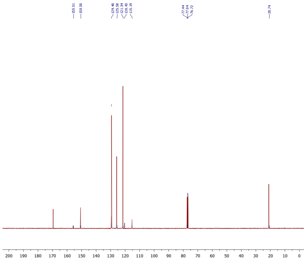
Figure S2 : ^{13}\text{C} NMR spectrum of compound 1
