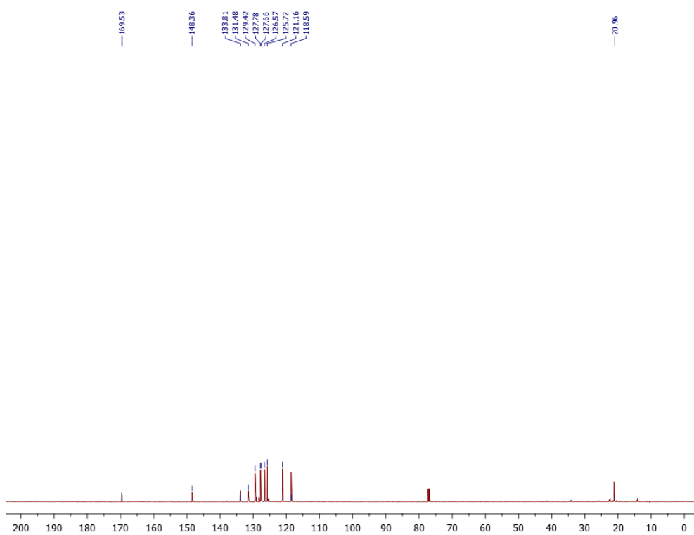
Figure S6 : ^{13}\text{C} NMR spectrum of compound 6
