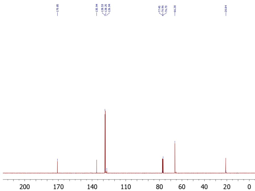
Figure S4 : ^{13}\text{C} NMR spectrum of compound 5
