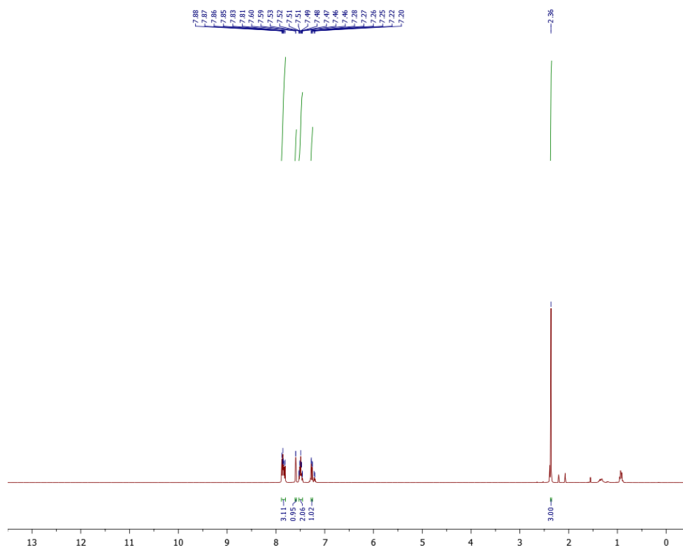
Figure S5 : ^1\text{H} NMR spectrum of compound 6
