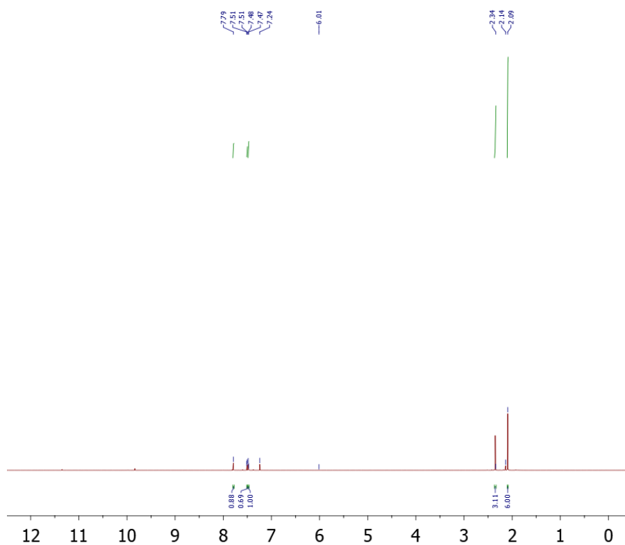
Figure S8 : ^{13}\text{C} NMR spectrum of compound 15
