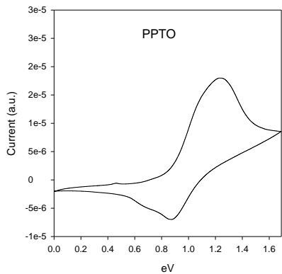
S1: Cyclic voltammograms of polymers.
