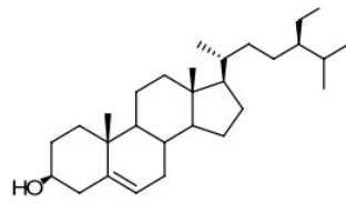
\beta -Sitosterol
