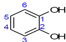
Catechol
