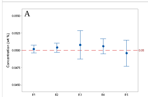
Figure 1. A) Graphical representation of homogeneity study and B) linear regression plots for long-term stability study during 12 months of storage at -20 °C for phenoxyethanol and parabens in cosmetic cream reference material
