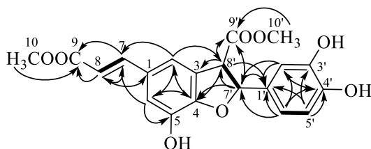
Figure 2. ^1\text{H} - ^1\text{H} COSY (—) correlations and HMBC ( \text{H} \rightarrow \text{C} ) correlations of compound 1
