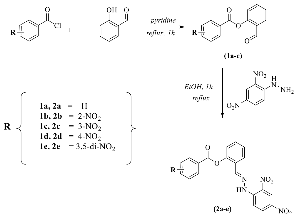
Figure 1. Synthetic route for the preparation of hydrazone derivatives
