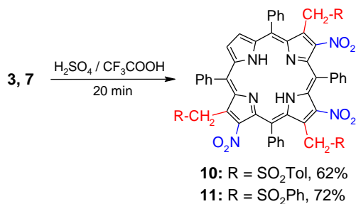
Scheme 4. Demetallation of copper(II)-complexes of hexasubstituted products.
