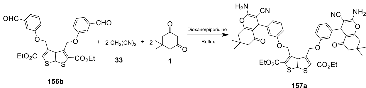
Scheme 58. Synthesis of bis-chromene-3-carbonitrile 157a
