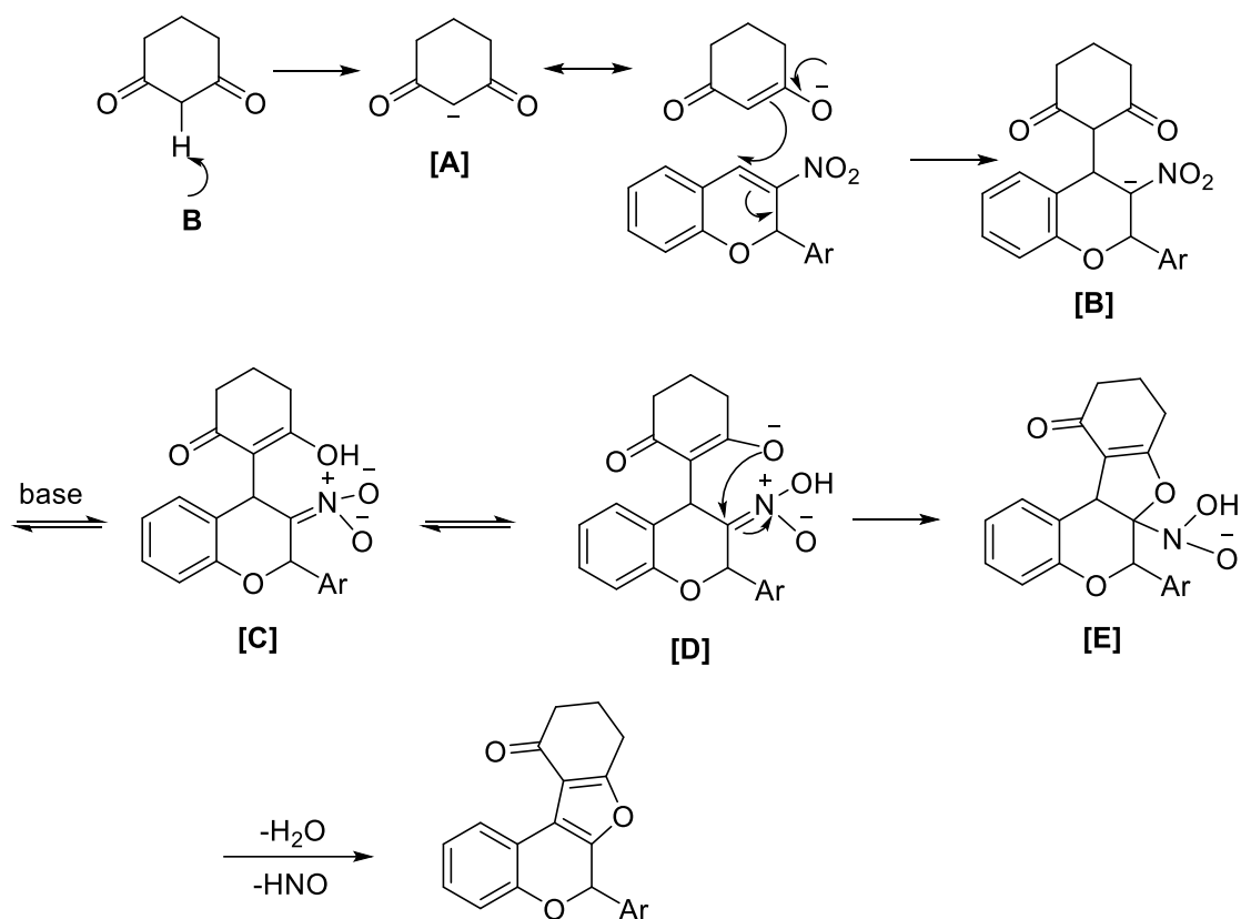
Scheme 19. Tentative reaction mechanism
