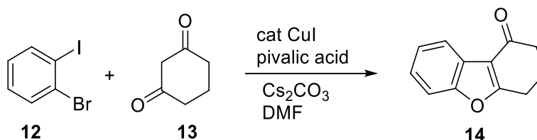
Scheme 8. Synthesis of furans derivative 14
