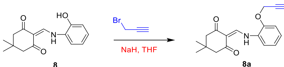
Scheme 5. Synthesis of 2-(((2-hydroxyphenyl)amino)methylene)-dimedone propargyl ether
