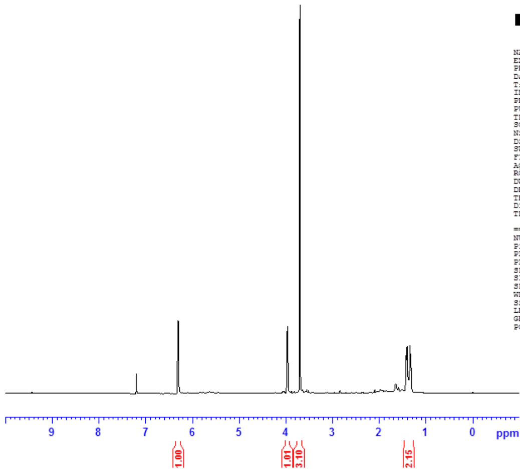
Figure S5. ^1\text{H} NMR spectrum of compound 5
