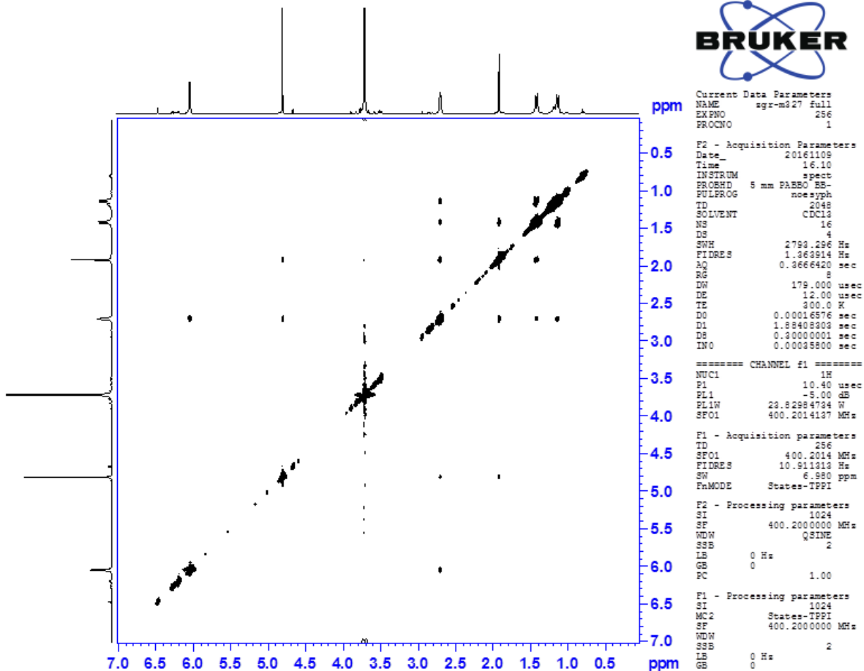
Figure S4. NOESY NMR spectrum of compound 6
