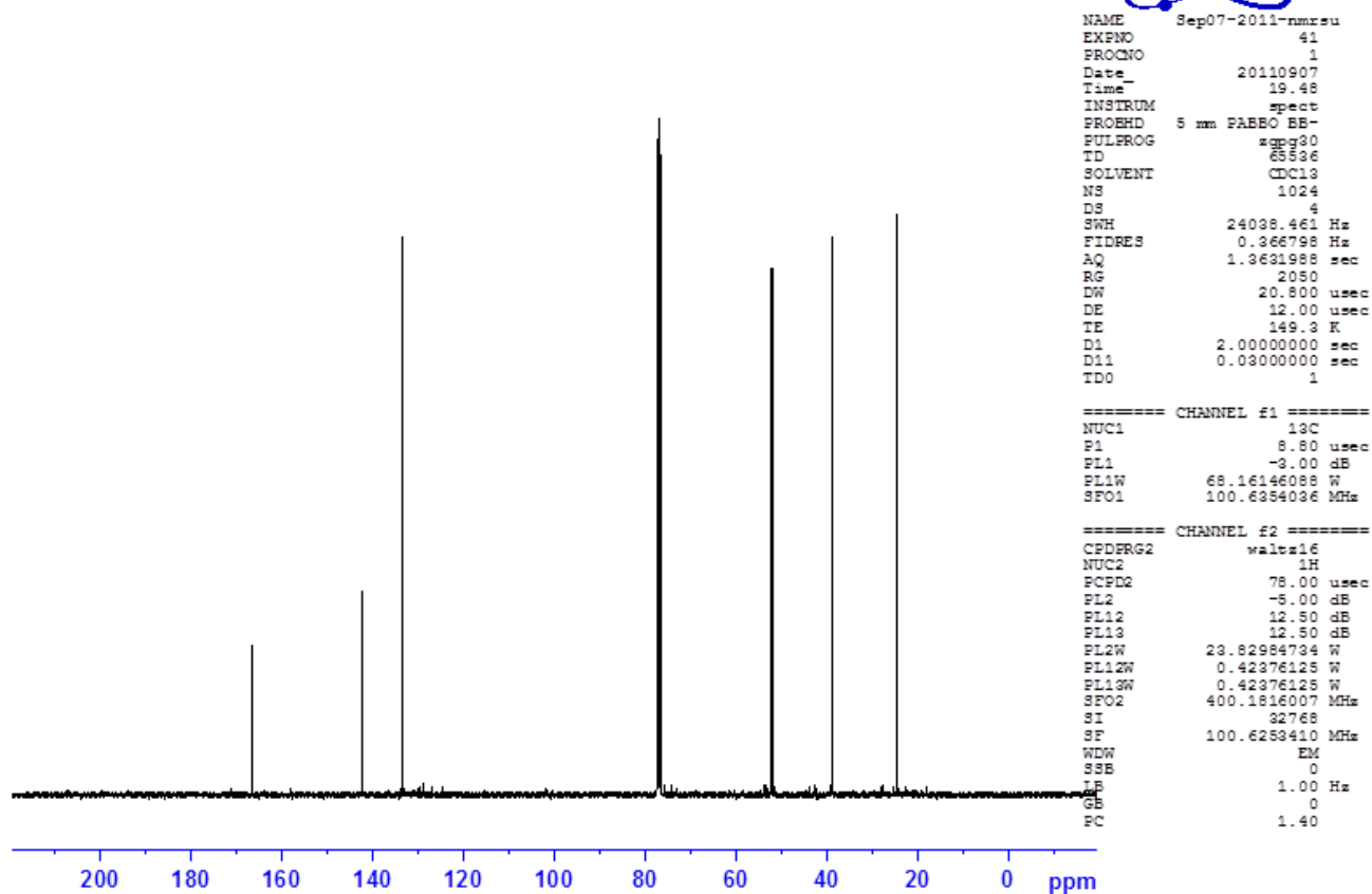
Figure S6. ^{13}\text{C} NMR spectrum of compound 5
