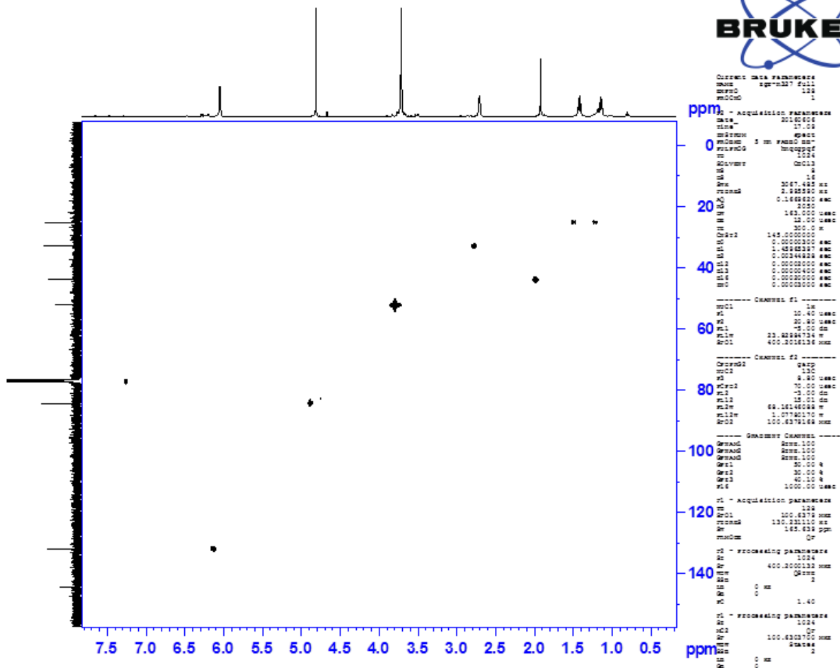
Figure S3. HMQC NMR spectrum of compound 6
