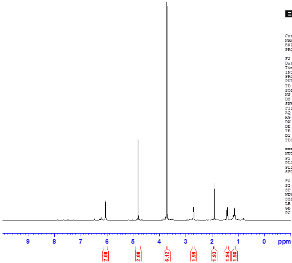
Figure S1. ^1\text{H} NMR spectrum of compound 6
