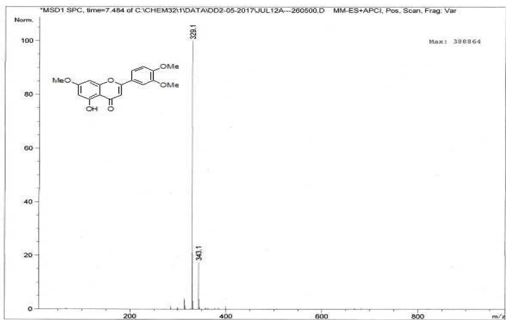
Figure S9. Mass data of compound 2c
