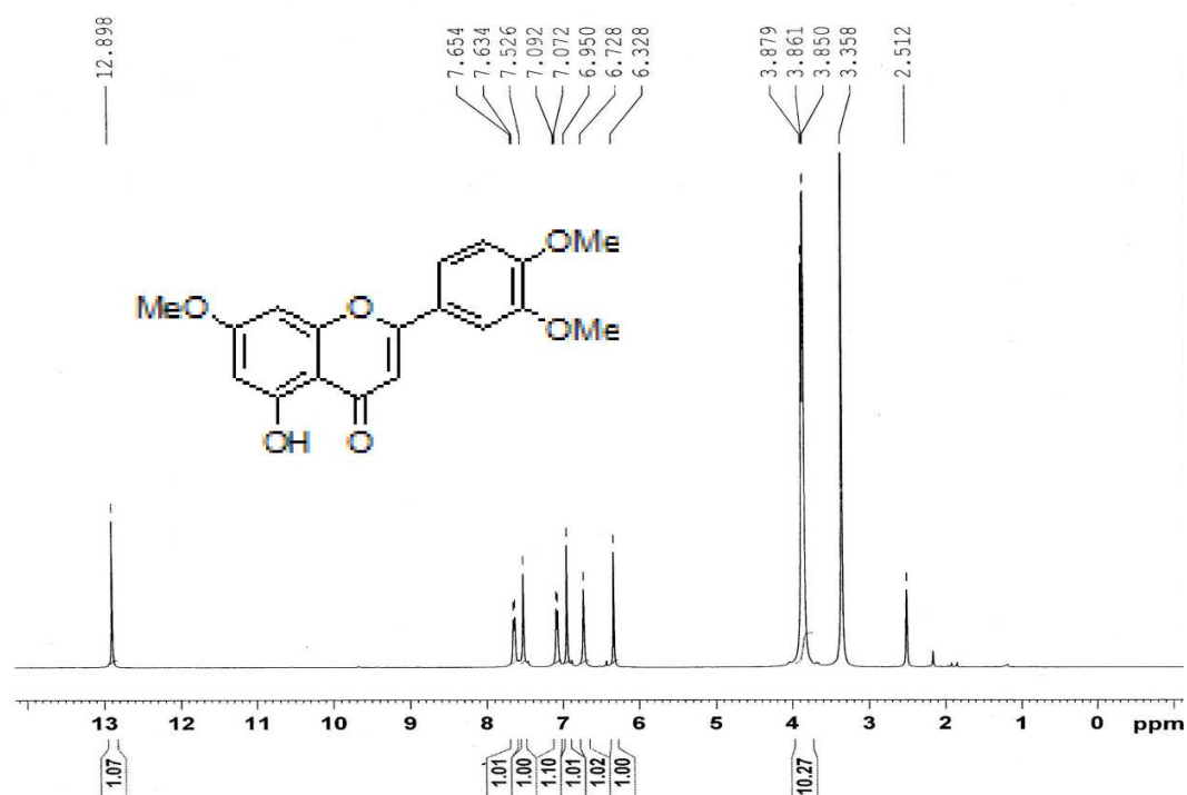
Figure 7. 1 H NMR data of compound 2c
