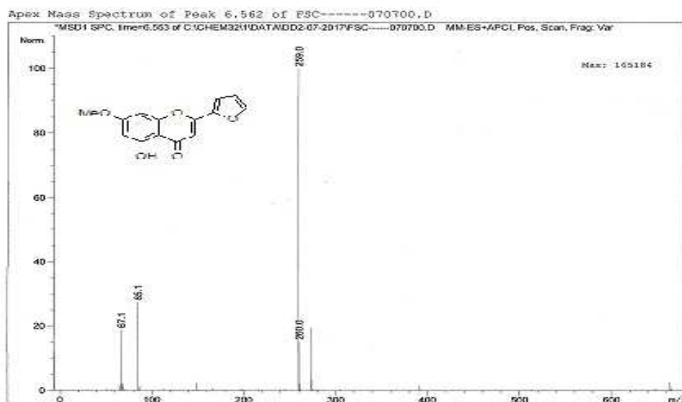
Figure S3. Mass data of compound 2a
