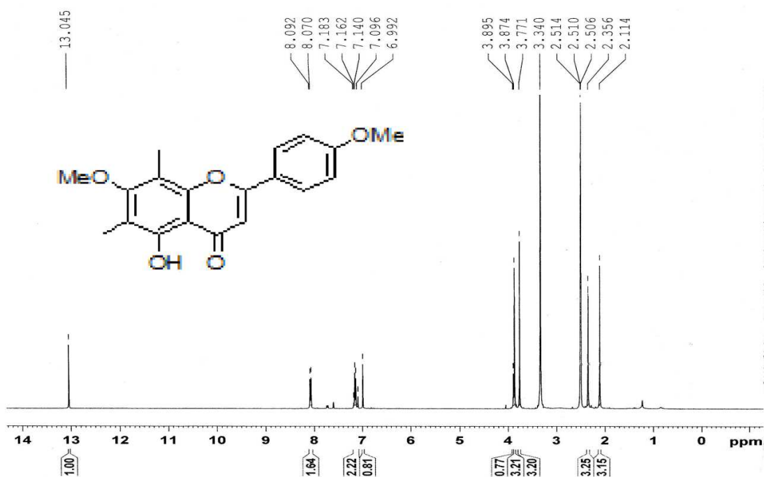
Figure S10. 1 H NMR data of compound 2d
