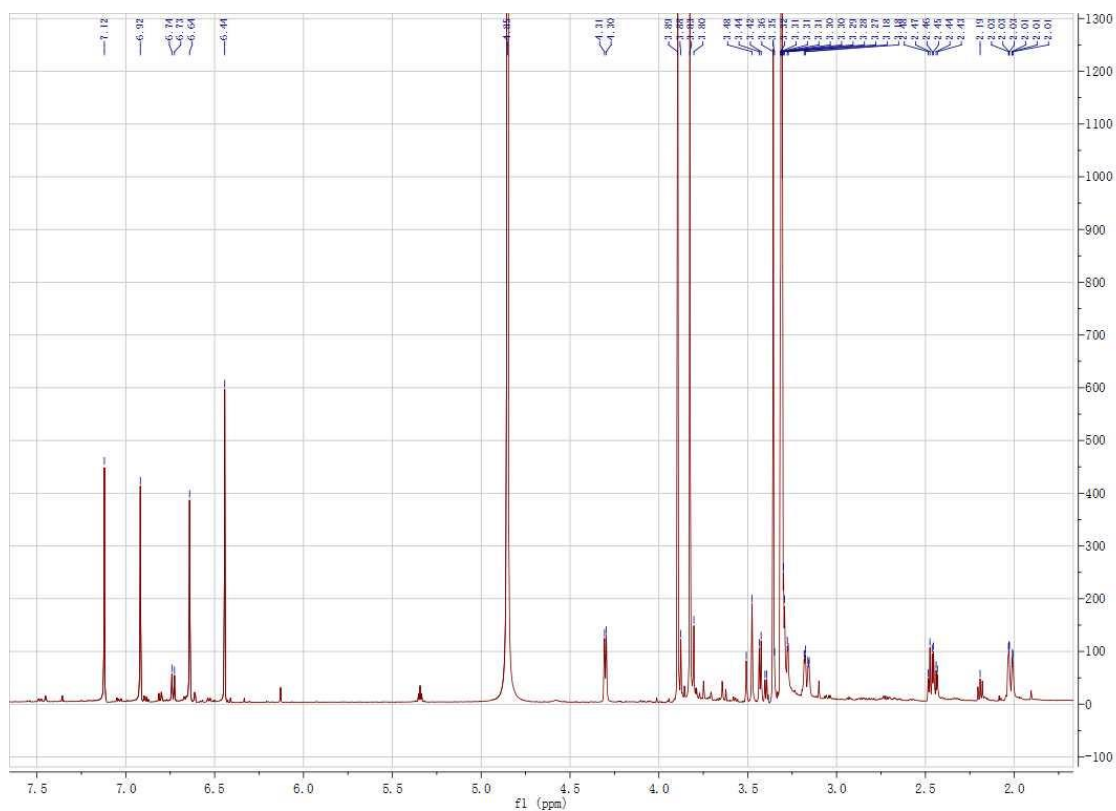
Figure S2: ^1\text{H} NMR (600 MHz, \text{CD}_3\text{OD} ) spectrum of the new compound 1
