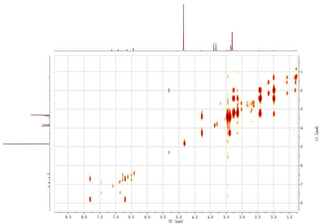
Figure S5: 1 H- 1 H COSY spectrum of the new compound 1
