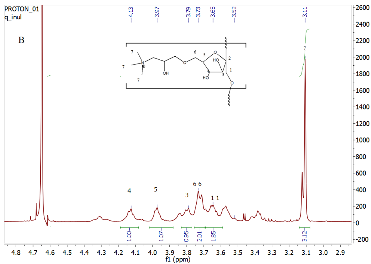
Figure S2: ^1\text{H} -NMR spectra of A: Native inulin and B: QIn
