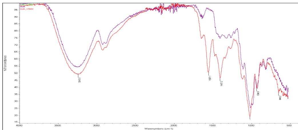
Figure S1 : FT-IR spectra of native inulin (purple line) and Qin (red line)
