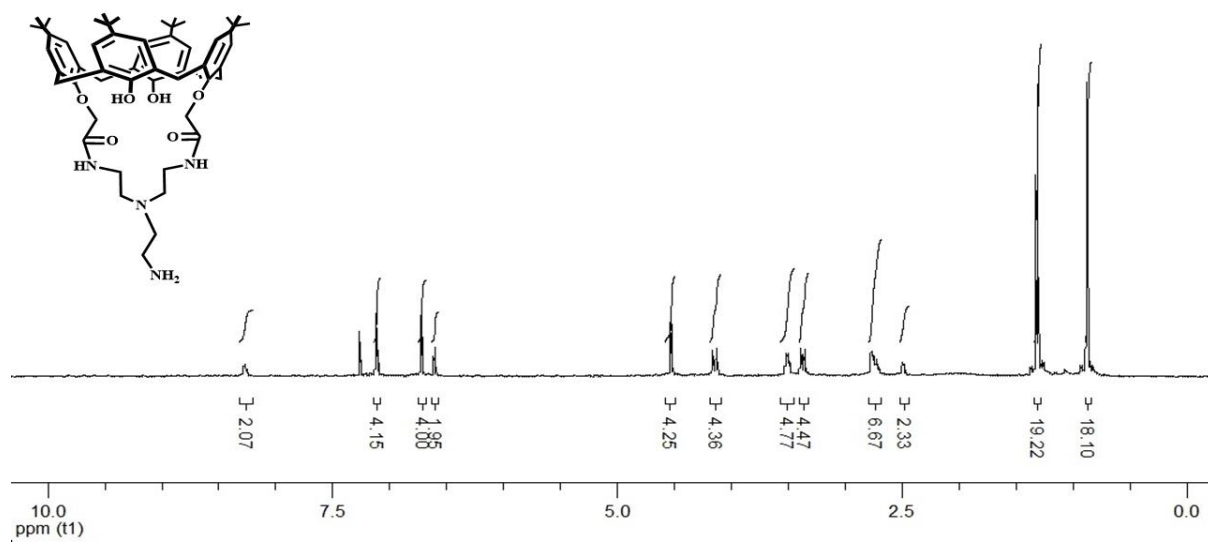
Figure S1: 1 H NMR spectrum of Calix-tren
