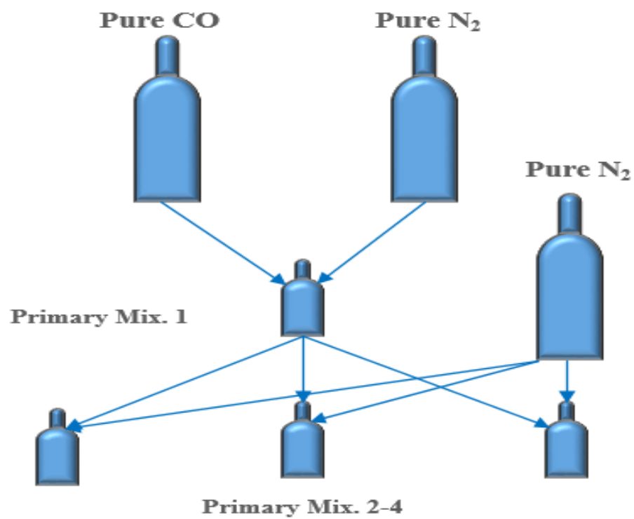
Figure S2: Schematic representation of the preparation of the primary gas mixtures
