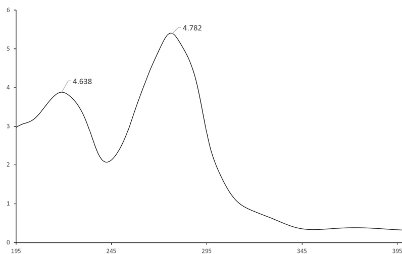
Figure S14: The UV spectrum of compound 1
