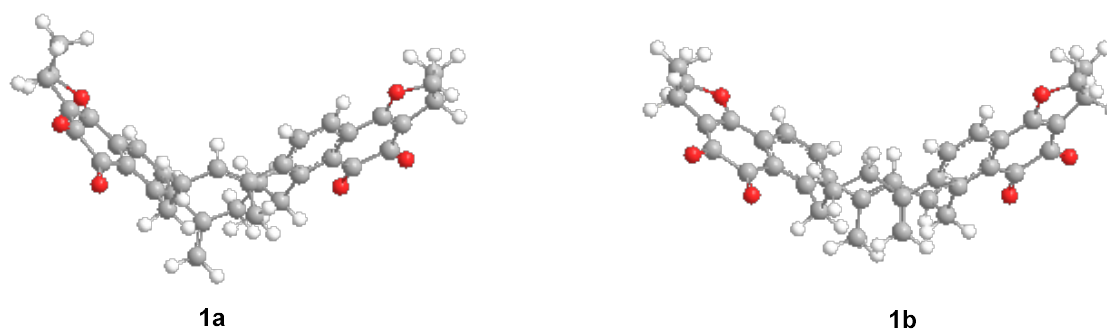
Figure S15: Most stable conformers of 3R, 3R'-1 calculated with DFT at the CAM-B3LYP/DGDZVP level.
