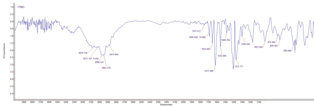
Figure S13: The IR spectrum of compound 1
