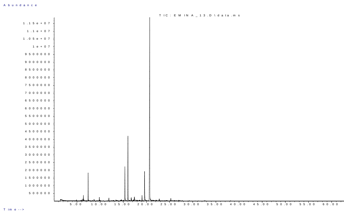
Figure S16: GC-MS chromatogram of C. nepeta - dried sample HS volatiles on F1, location D
