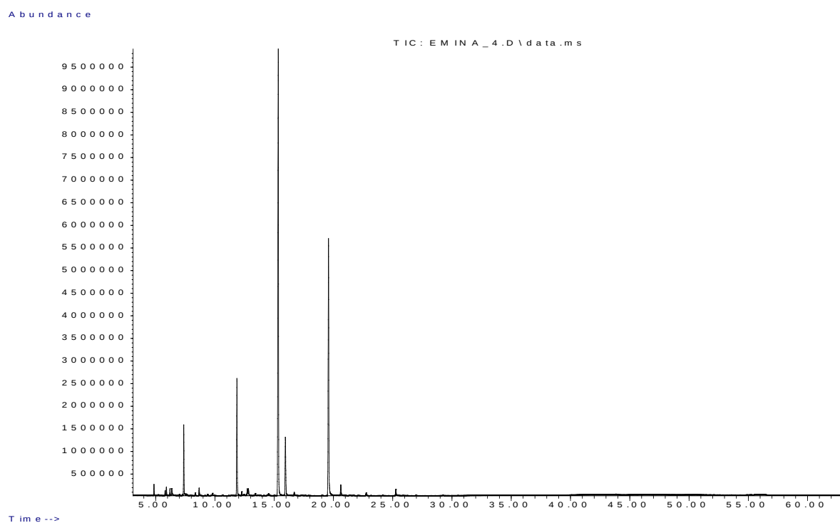
Figure S9: GC-MS chromatogram of C. nepeta of EO volatiles, location B
