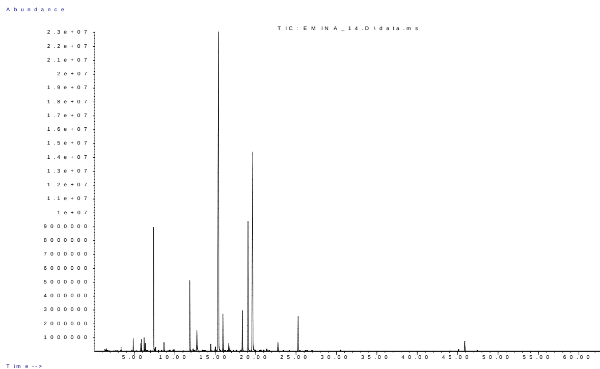
Figure S6: GC-MS chromatogram of C. nepeta - fresh sample HS volatiles on F2, location B
