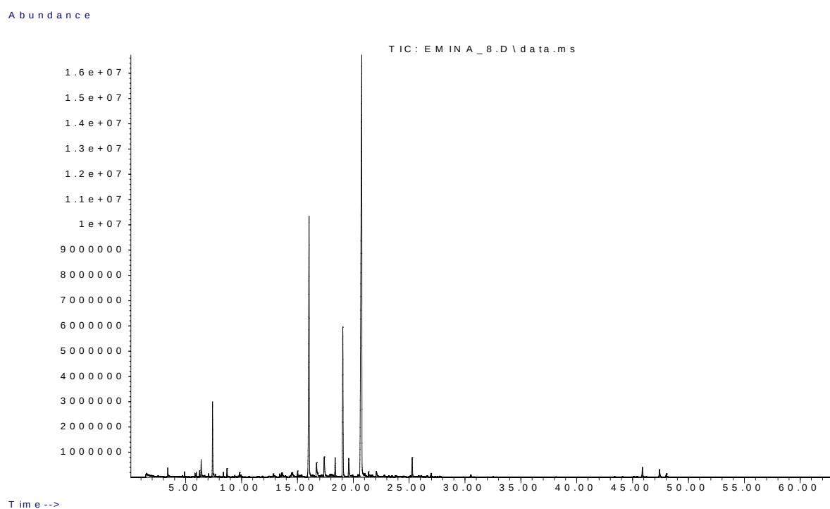
Figure S10: GC-MS chromatogram of C. nepeta - fresh sample HS volatiles on F1, location C
