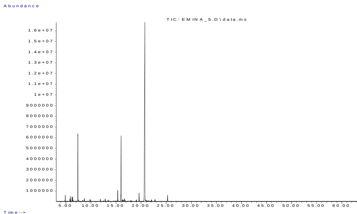
Figure S4: GC-MS chromatogram of C. nepeta of EO volatiles, location A
