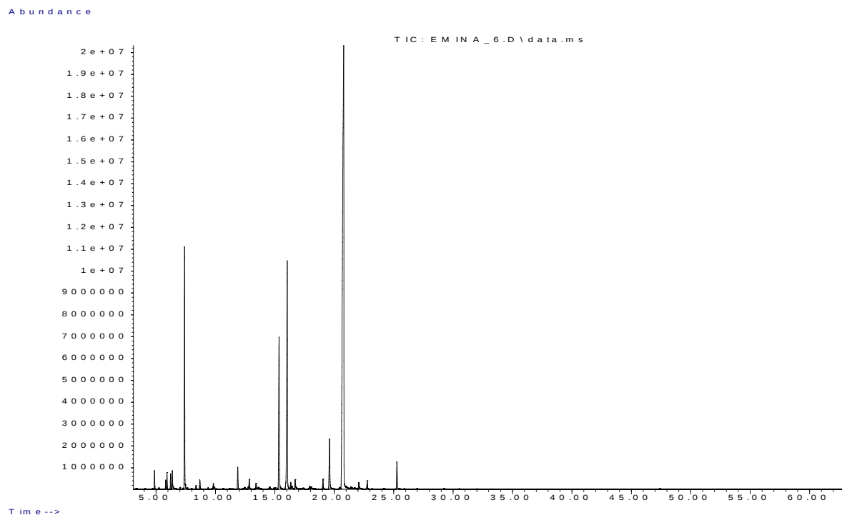
Figure S18: GC-MS chromatogram of C. nepeta EO volatiles, location D
