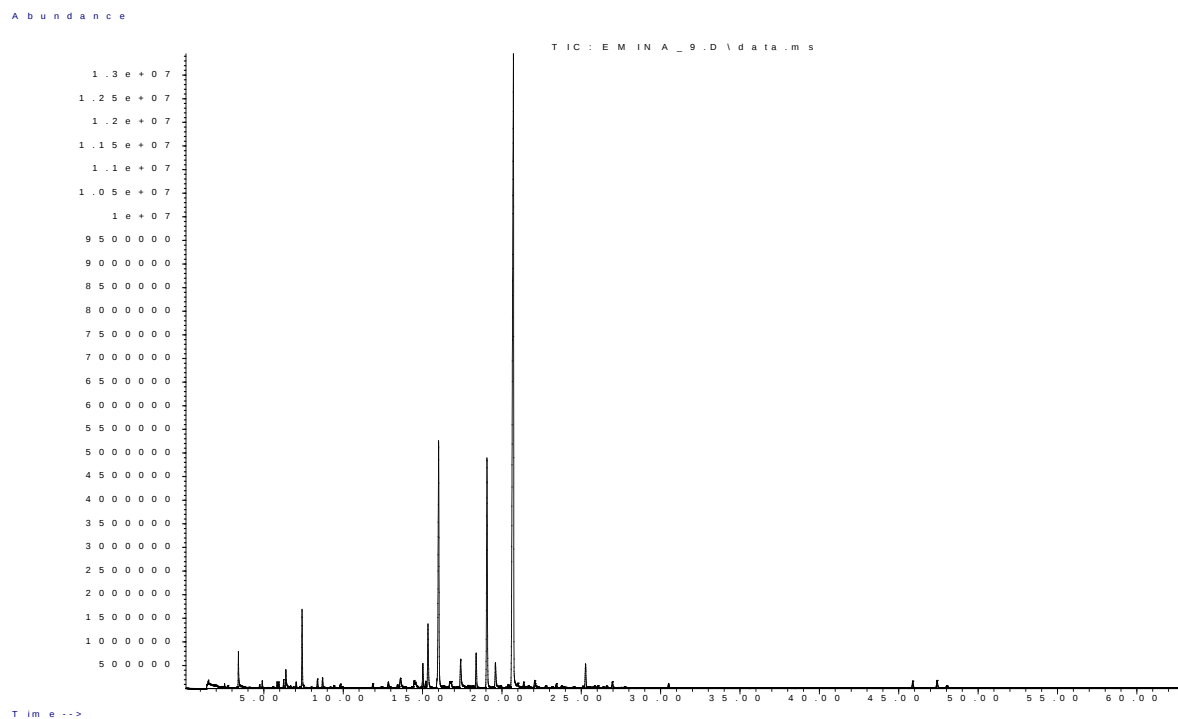
Figure S14: GC-MS chromatogram of C. nepeta - fresh sample HS volatiles on F1, location D
