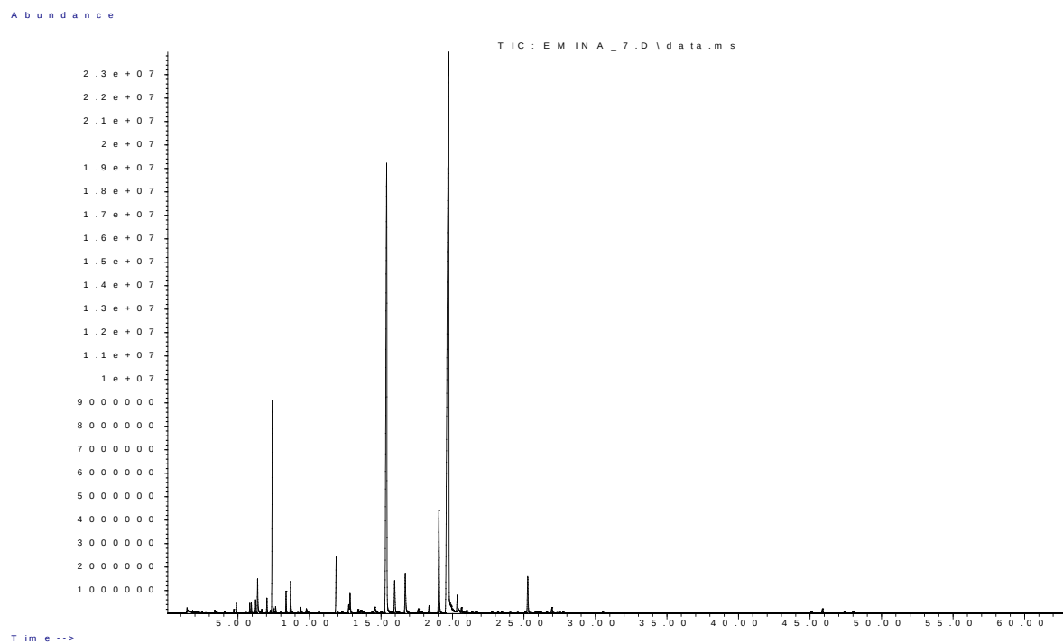
Figure S5: GC-MS chromatogram of C. nepeta - fresh sample HS volatiles on F1, location B
