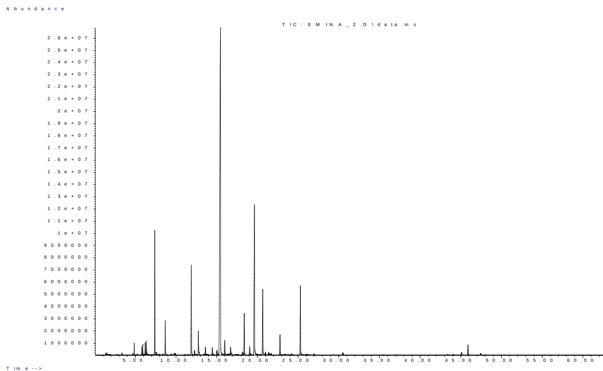
Figure S1: GC-MS chromatogram of C. nepeta - fresh sample HS volatiles on F2- location A
