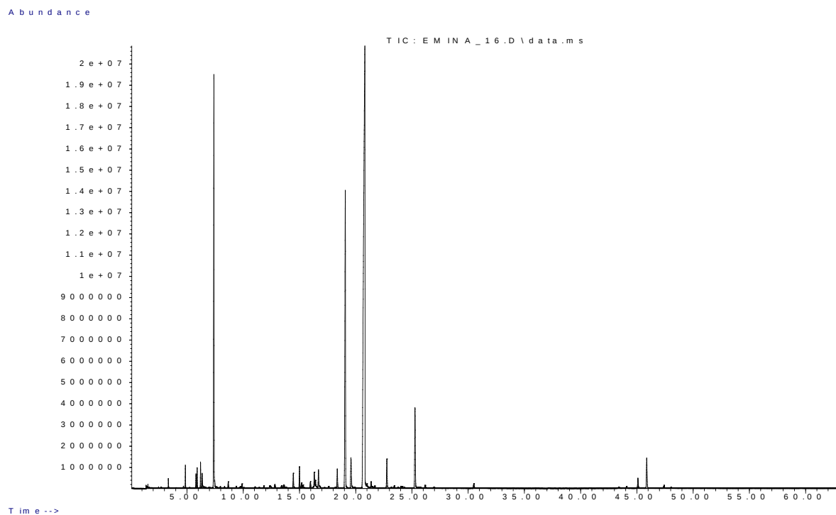
Figure S15: GC-MS chromatogram of C. nepeta - fresh sample HS volatiles on F2, location D
