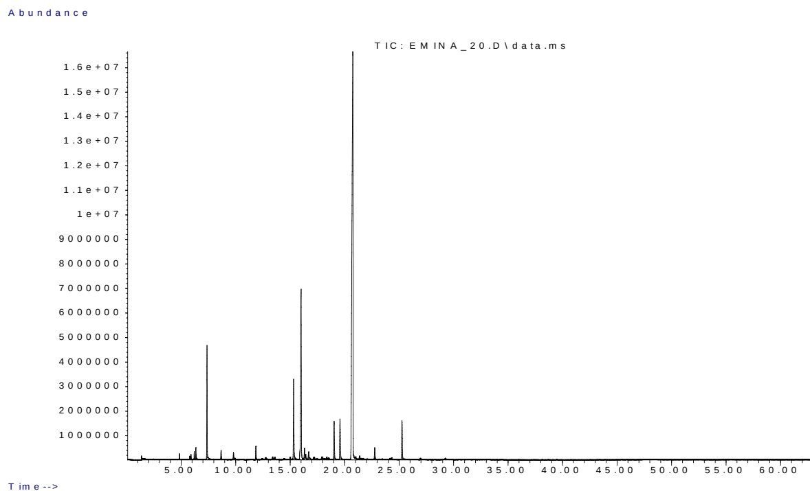
Figure S17: GC-MS chromatogram of C. nepeta -dried sample HS volatiles on F1, location D
