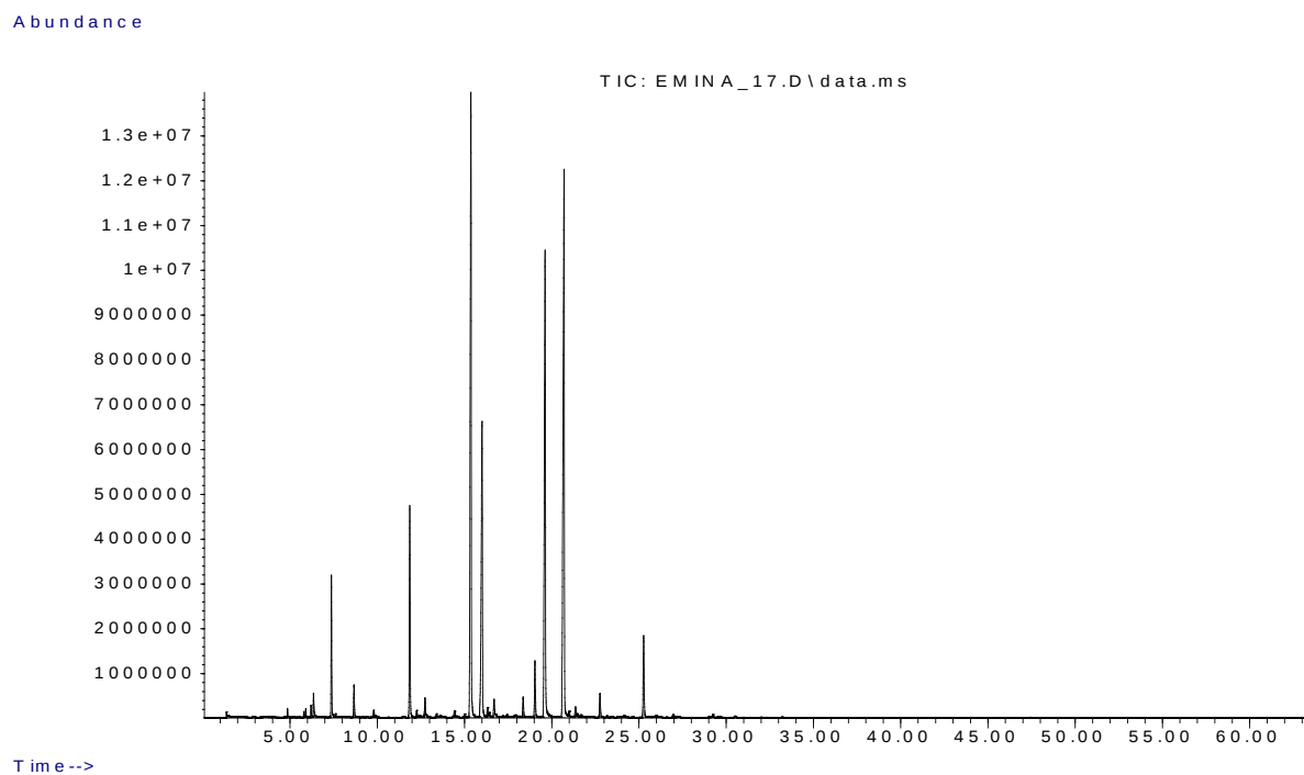
Figure S3: GC-MS chromatogram of C. nepeta -dried sample HS volatiles on F2, location A
