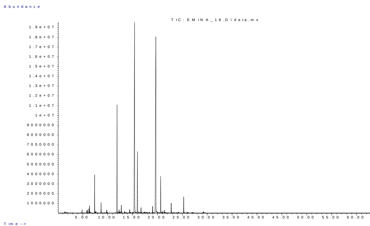
Figure S8: GC-MS chromatogram of C. nepeta - dried sample HS volatiles on F2, location B
