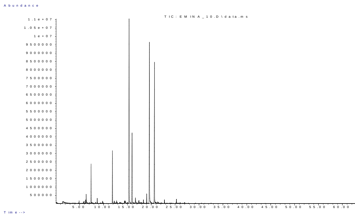
Figure S2: GC-MS chromatogram of C. nepeta - dried sample HS volatiles on F1, location A
