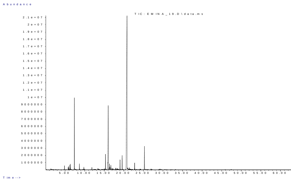
Figure S13: GC-MS chromatogram of C. nepeta - dried sample HS volatiles on F2, location C
