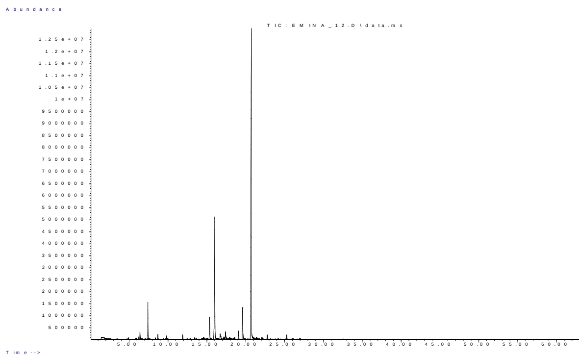
Figure S12: GC-MS chromatogram of C. nepeta - dried sample HS volatiles on F1, location C
