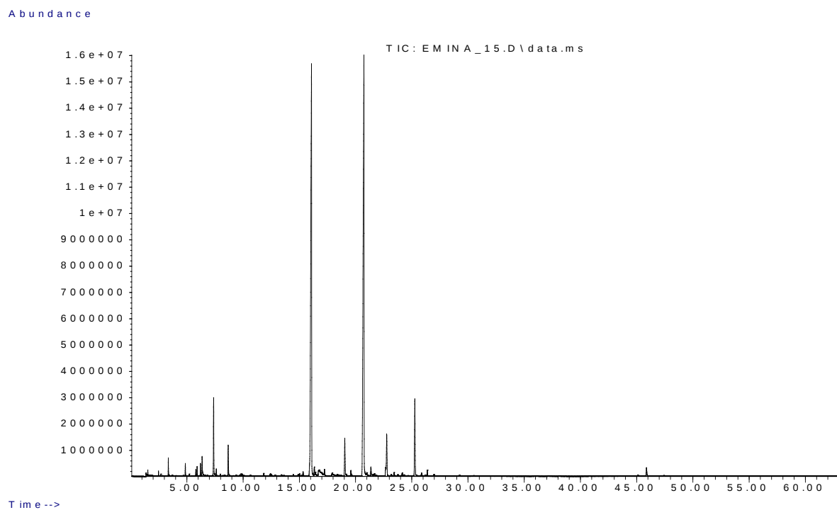
Figure S11: GC-MS chromatogram of C. nepeta - fresh sample HS volatiles on F2, location C
