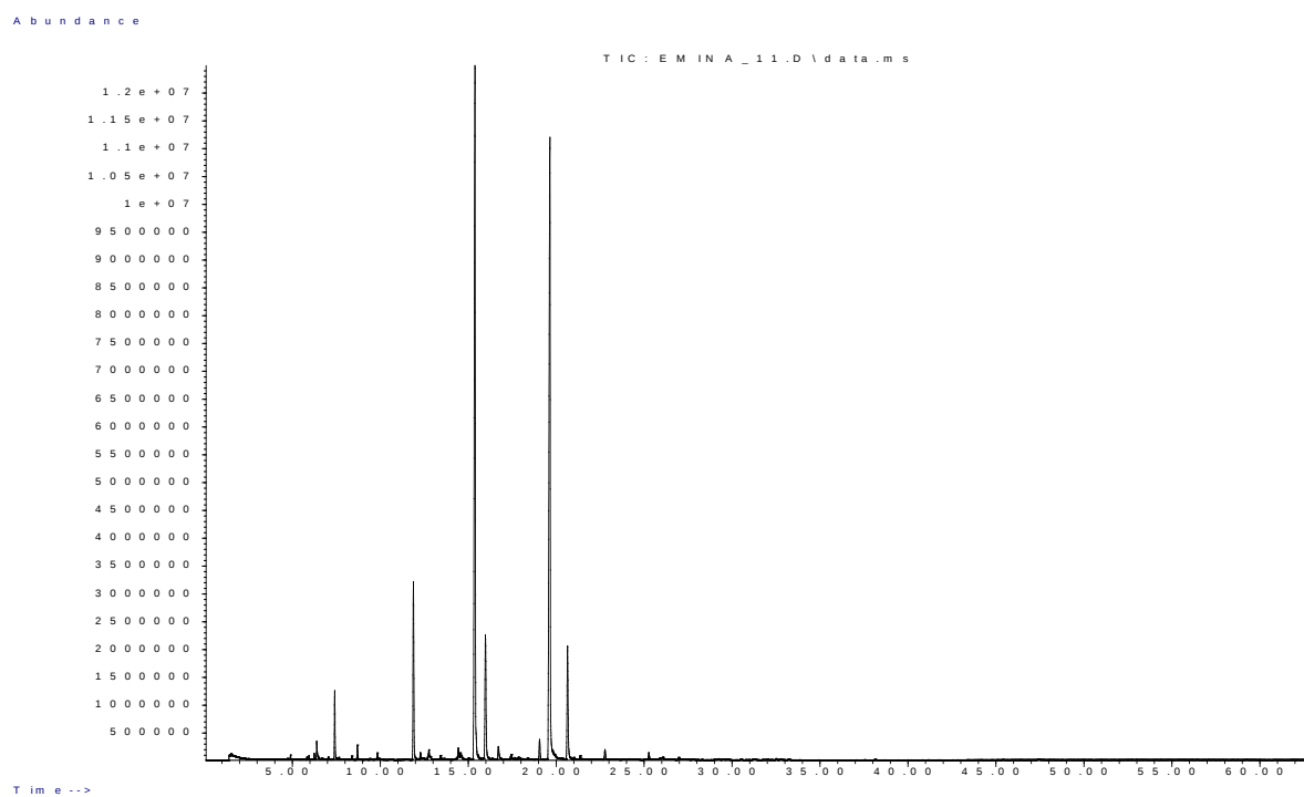
Figure S7: GC-MS chromatogram of C. nepeta - dried sample HS volatiles on F1, location B
