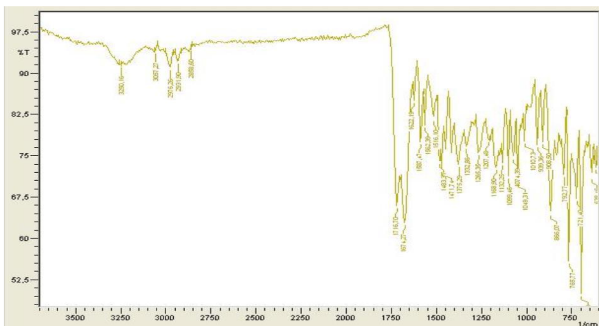
Figure S87: IR spectrum of the compound 4p
