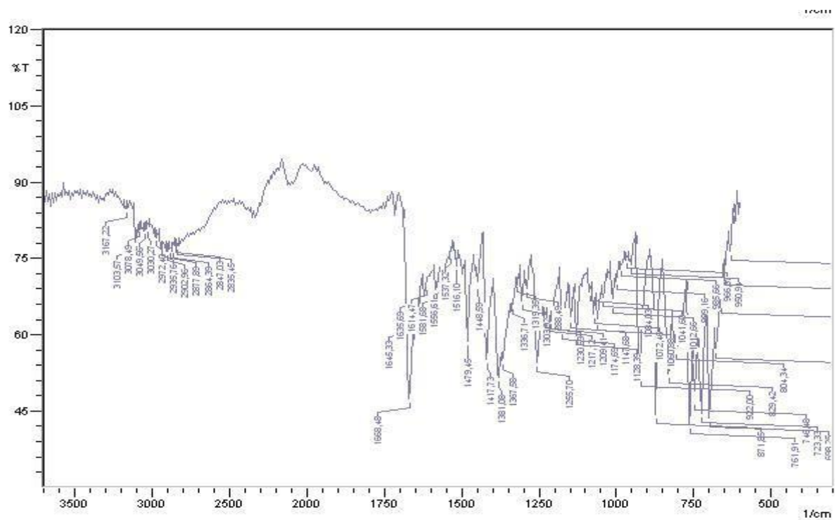
Figure S25: IR spectrum of the compound 3j
