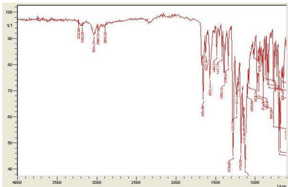
Figure S19: IR spectrum of the compound 3h
