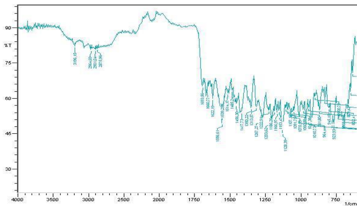
Figure S37: IR spectrum of the compound 3n
