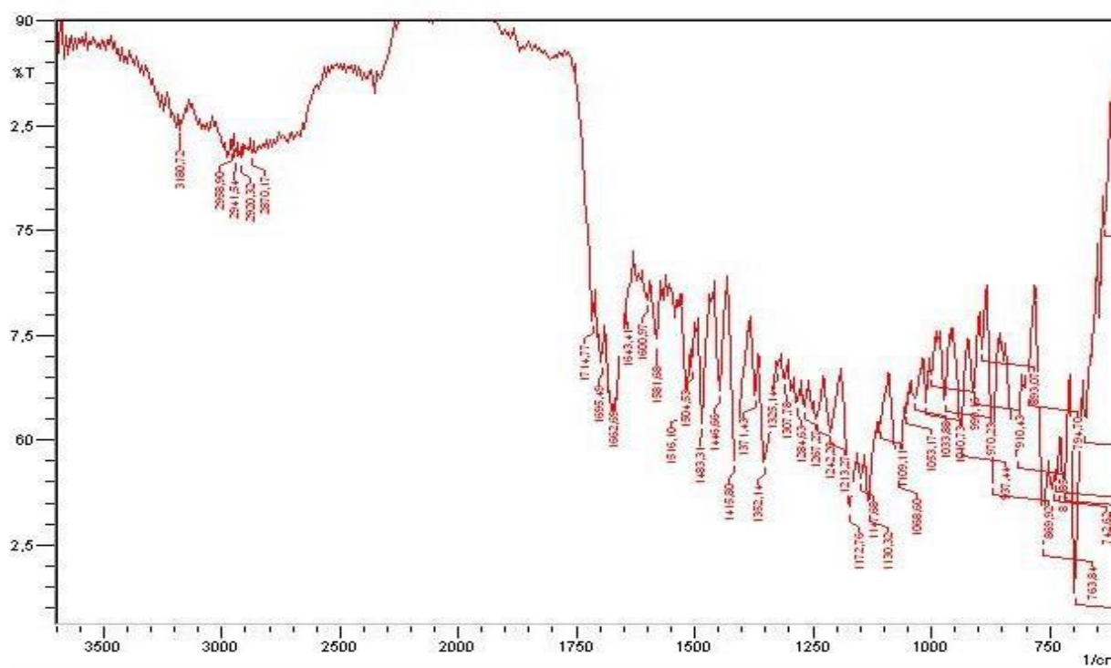
Figure S70: IR spectrum of the compound 4j
