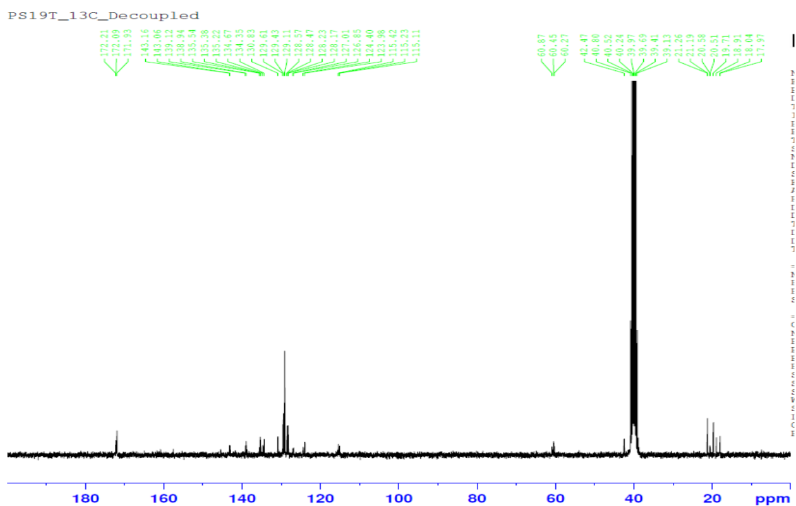
Figure S92: ^{13}\text{C} -NMR spectrum of the compound 4r
