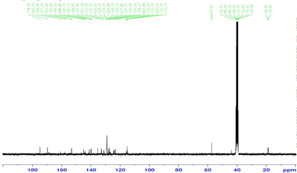
Figure S33: ^{13}\text{C} -NMR spectrum of the compound 31
