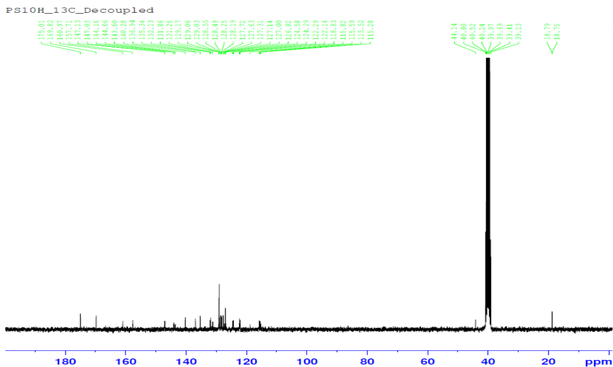
Figure S24: ^{13}\text{C} -NMR spectrum of the compound 3i
