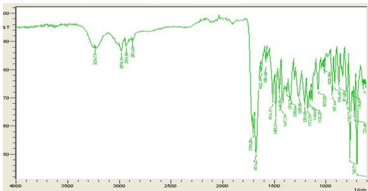
Figure S90: IR spectrum of the compound 4r
