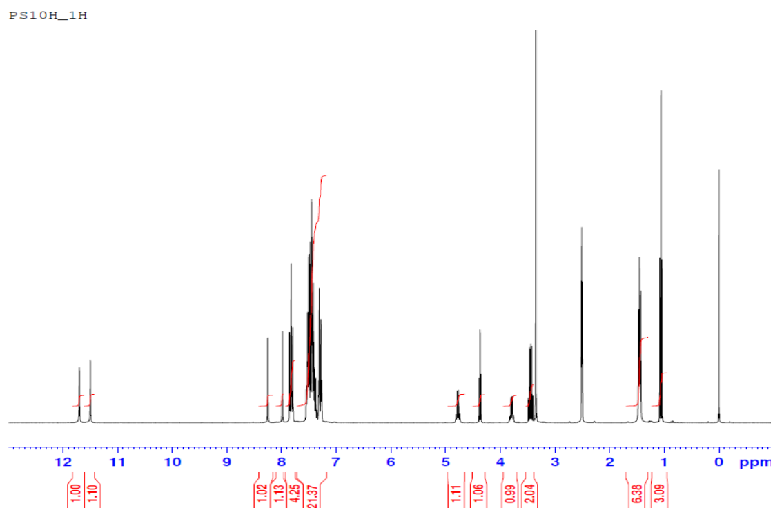
Figure S23: ^1\text{H} -NMR spectrum of the compound 3i
