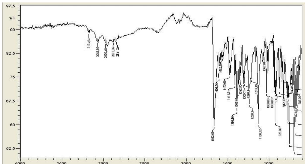
Figure S40: IR spectrum of the compound 3o
