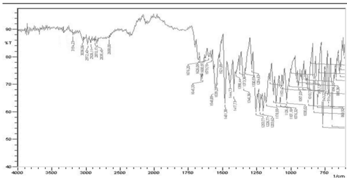
Figure S28: IR spectrum of the compound 3k
