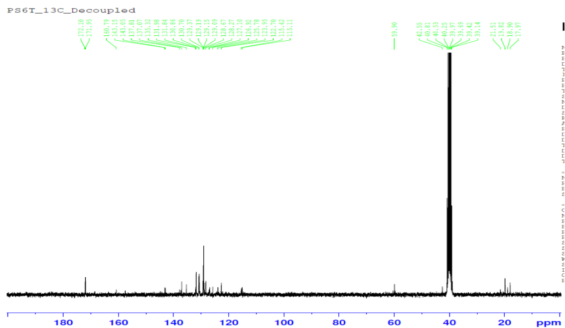
Figure S58: ^{13}\text{C} -NMR spectrum of the compound 4e
