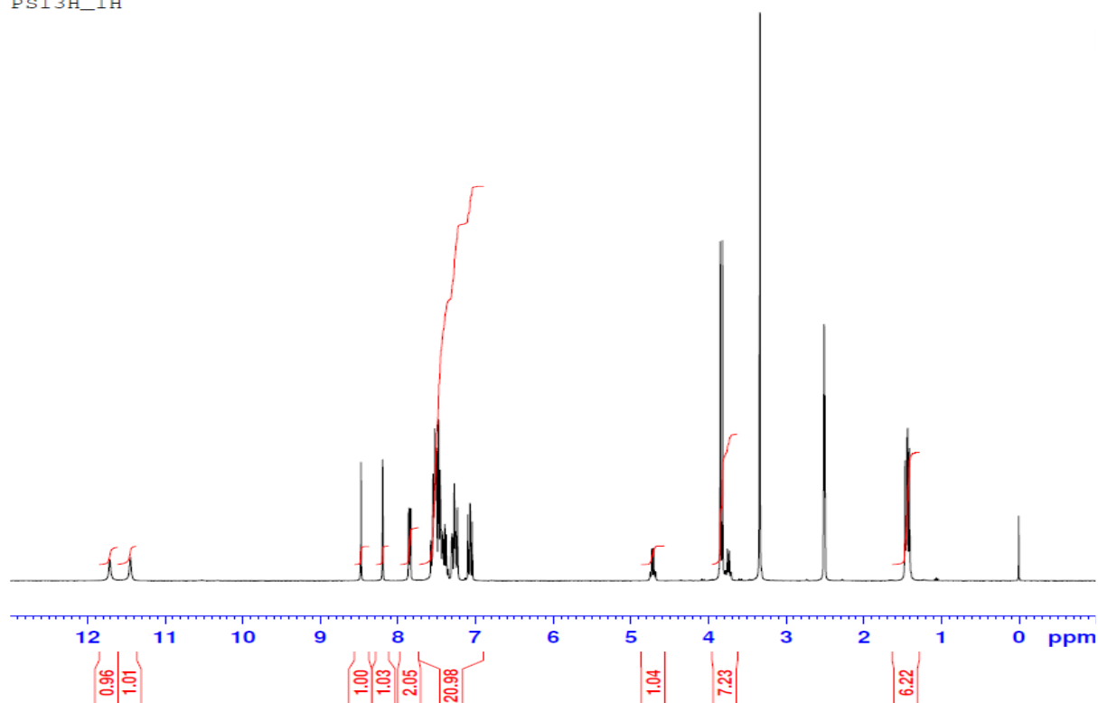
Figure S29: ^1\text{H} -NMR spectrum of the compound 3k
