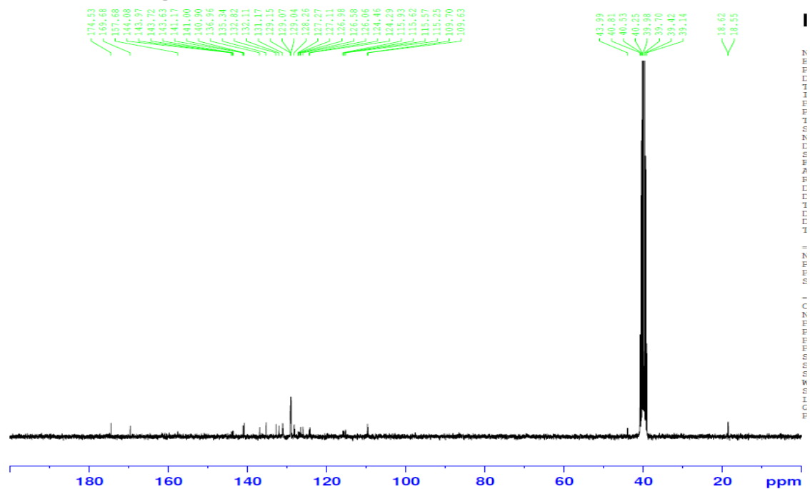
Figure S27: 13 C-NMR spectrum of the compound 3j
