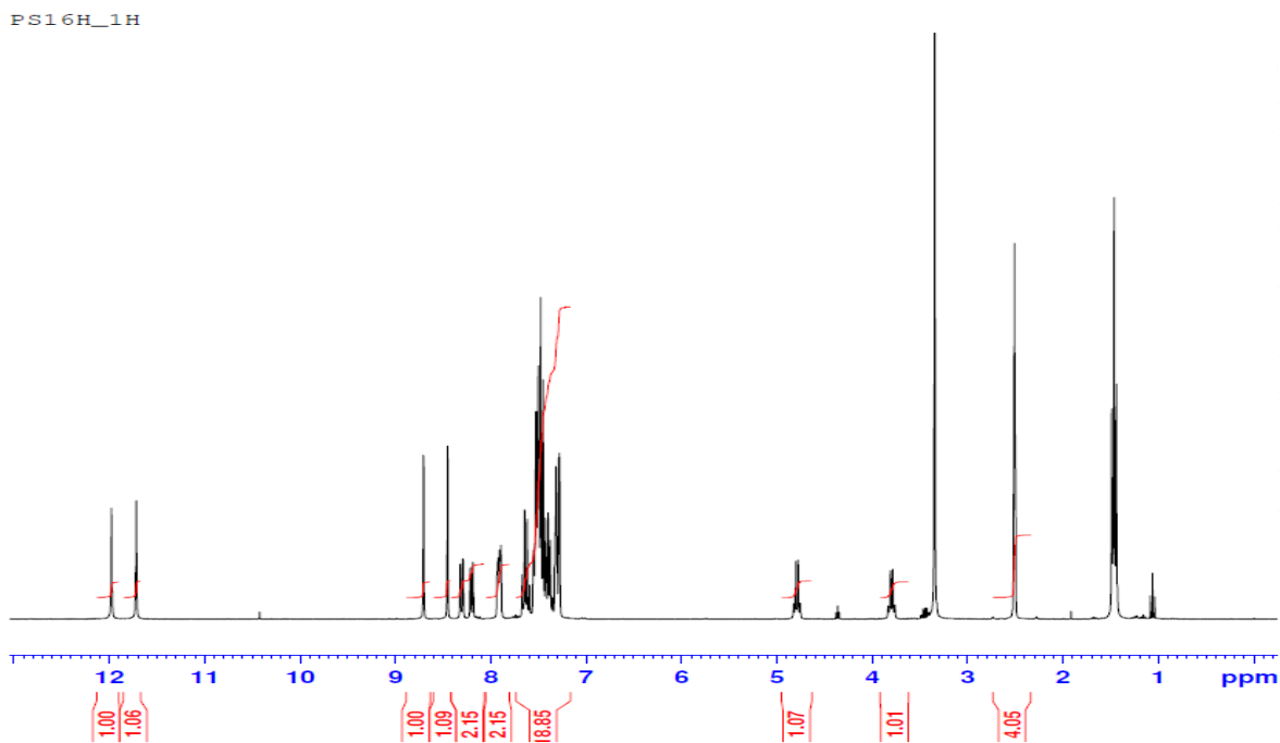
Figure S38: ^1\text{H} -NMR spectrum of the compound 3n
