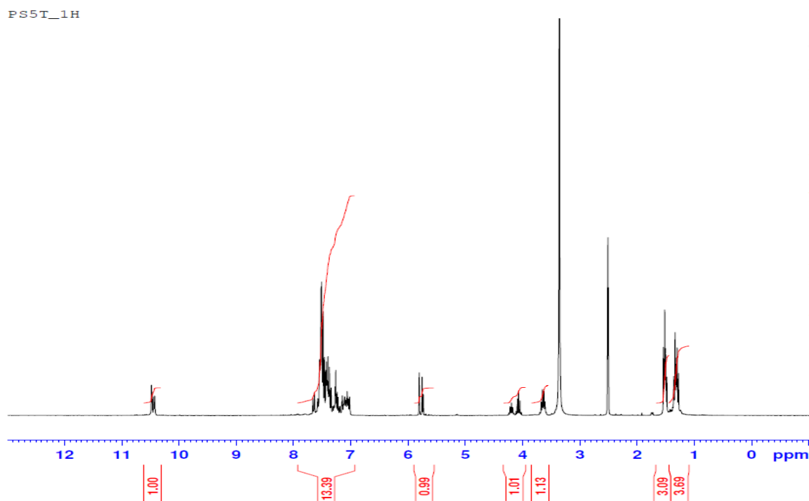
Figure S54: ^1\text{H} -NMR spectrum of the compound 4d
