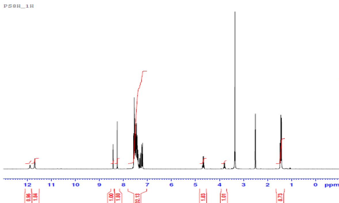
Figure S18: ^1\text{H} -NMR spectrum of the compound 3g
