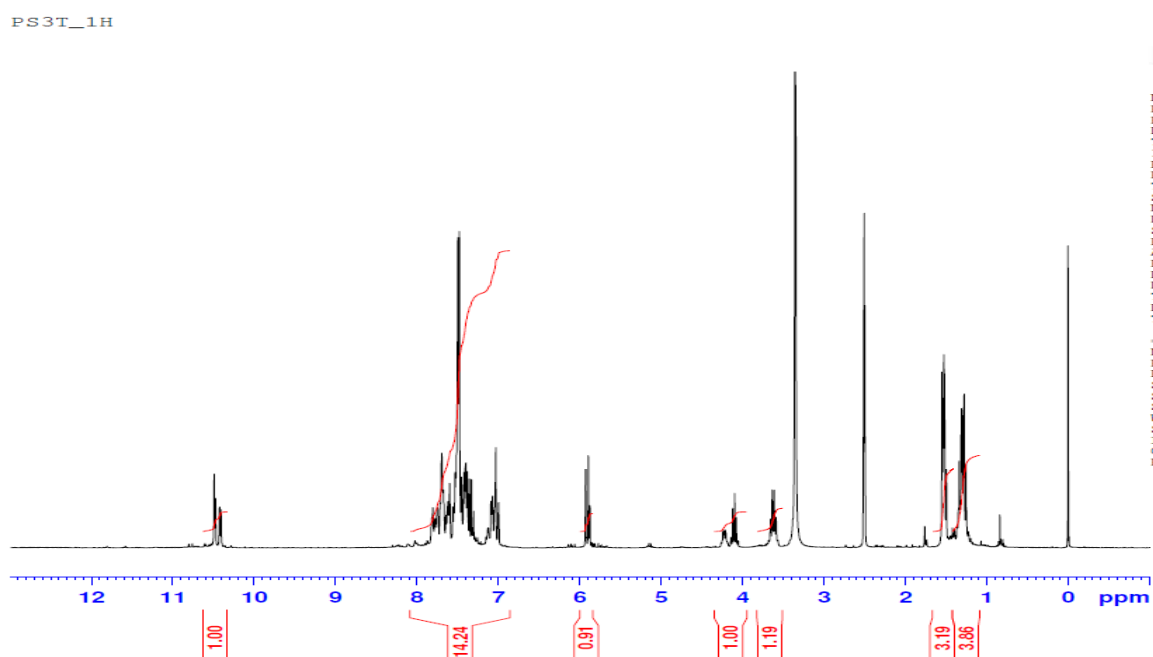
Figure S51: ^1\text{H} -NMR spectrum of the compound 4c
