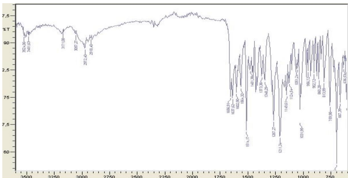
Figure S43: IR spectrum of the compound 3s
