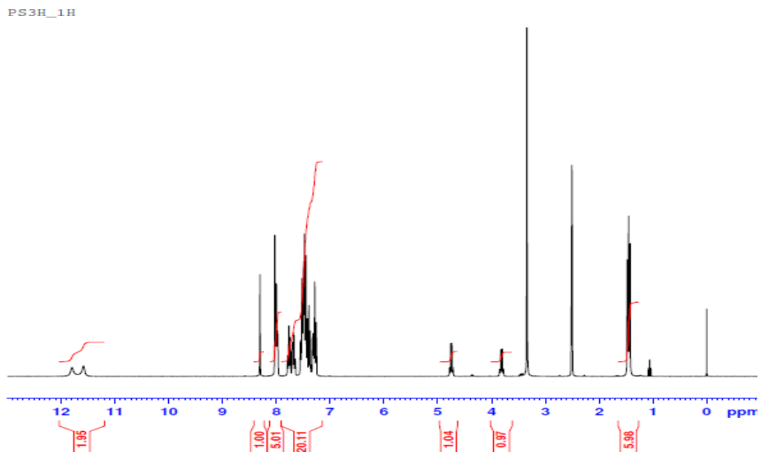
Figure S8: 1 H-NMR spectrum of the compound 3c
