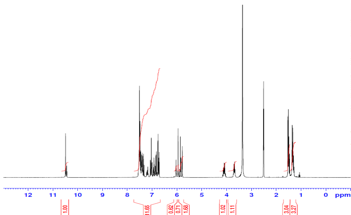
Figure S60: ^1\text{H} -NMR spectrum of the compound 4f
