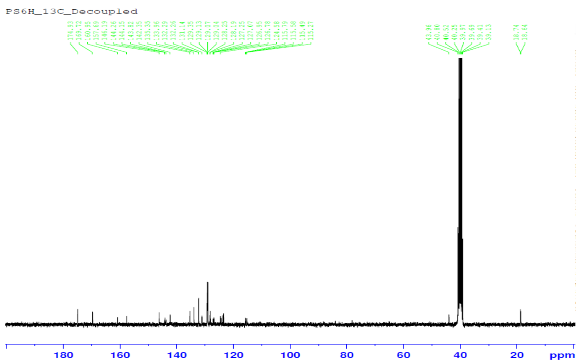
Figure S13: ^{13}\text{C} -NMR spectrum of the compound 3e
