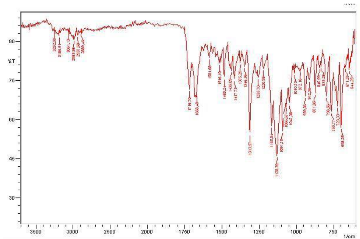
Figure S82: IR spectrum of the compound 4n
