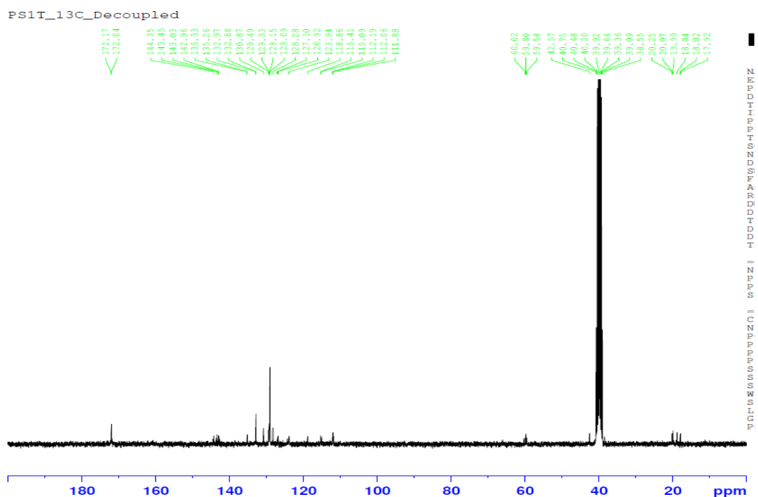
Figure S46: ^{13}\text{C} -NMR spectrum of the compound 4a
