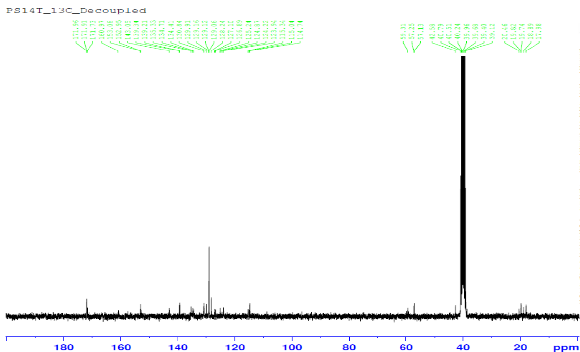
Figure S78: ^{13}\text{C} -NMR spectrum of the compound 4l
