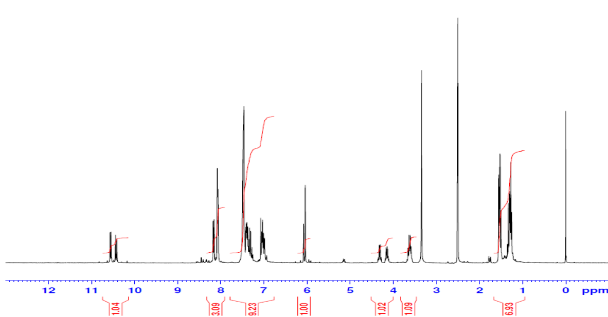
Figure S65: ^1\text{H} -NMR spectrum of the compound 4h
