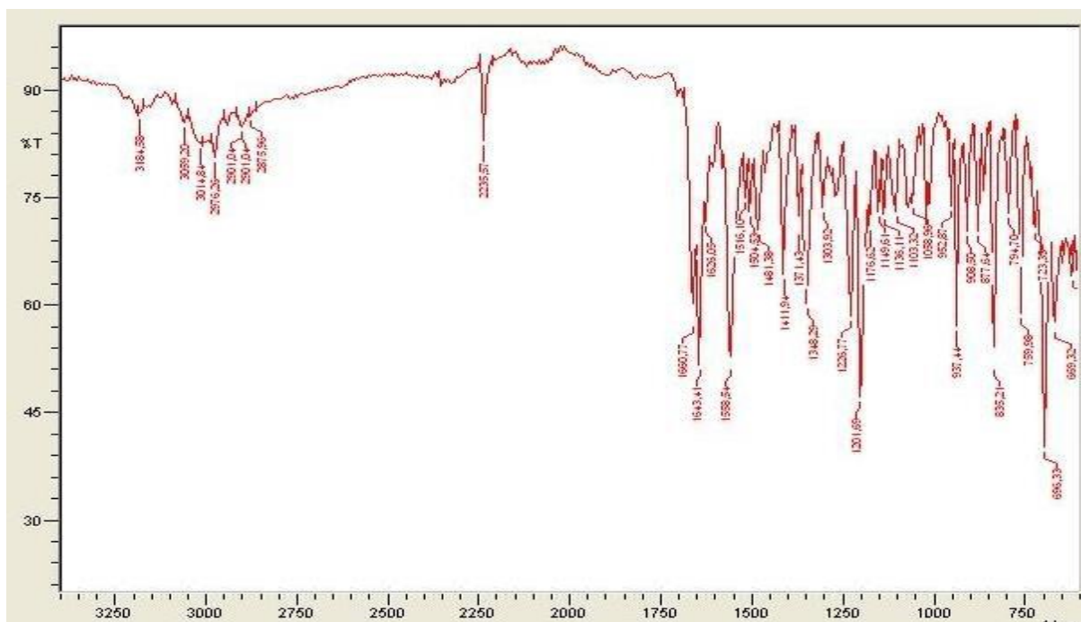
Figure S1: IR spectrum of the compound 3a
