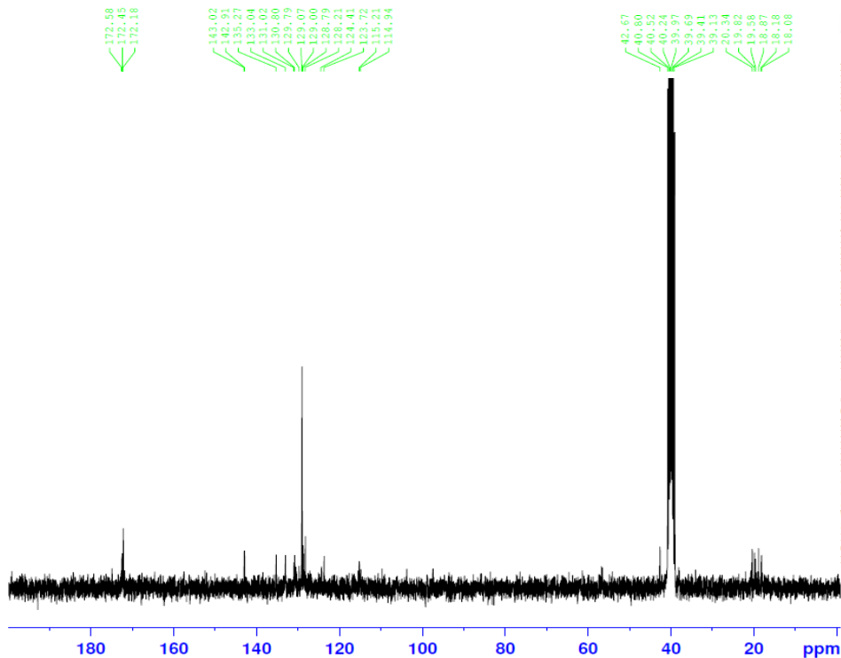
Figure S84: ^{13}\text{C} -NMR spectrum of the compound 4n
