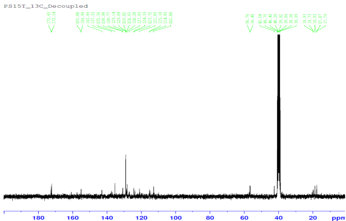
Figure S81: ^{13}\text{C} -NMR spectrum of the compound 4m
