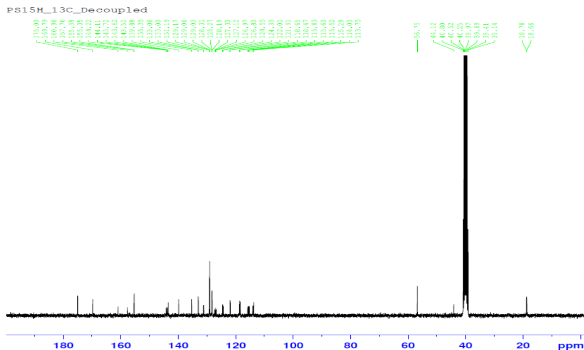
Figure S36: ^{13}\text{C} -NMR spectrum of the compound 3m
