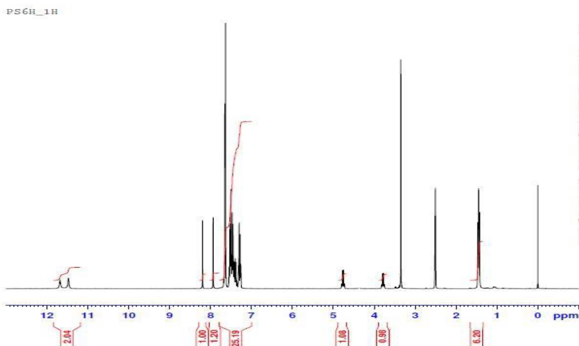
Figure S12: ^1\text{H} -NMR spectrum of the compound 3e
