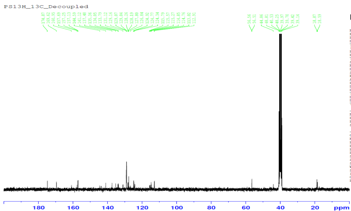
Figure S30: ^{13}\text{C} -NMR spectrum of the compound 3k
