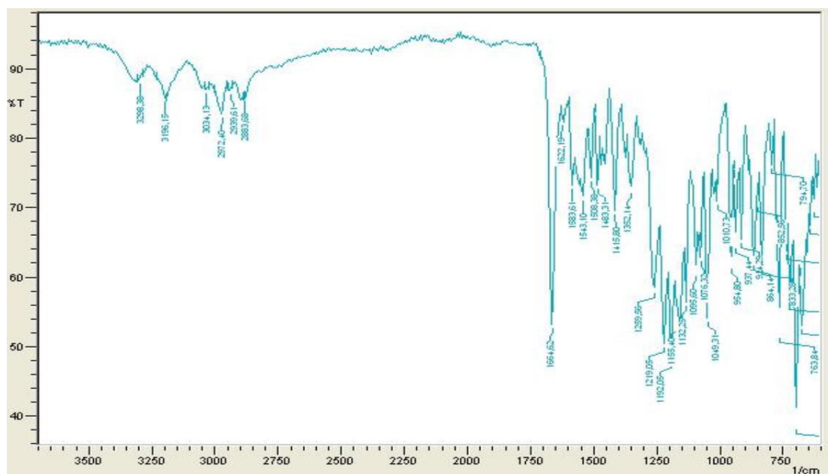
Figure S41: IR spectrum of the compound 3p
