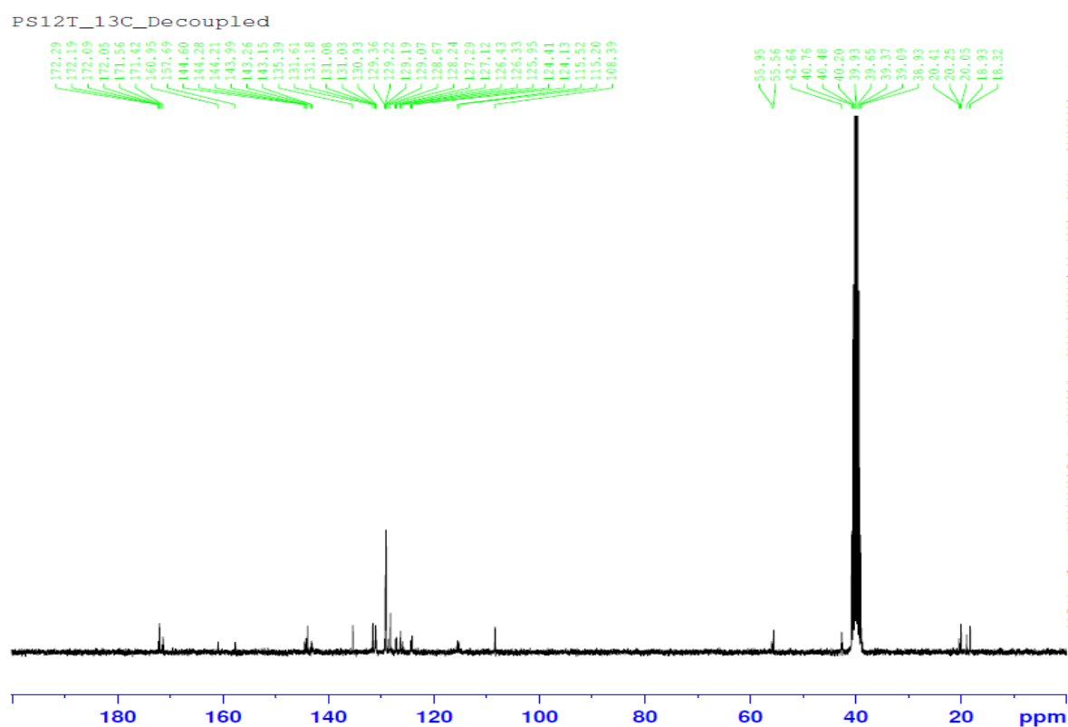
Figure S72: ^{13}\text{C} -NMR spectrum of the compound 4j
