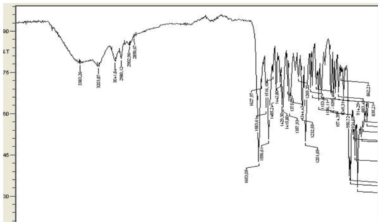
Figure S17: IR spectrum of the compound 3g
