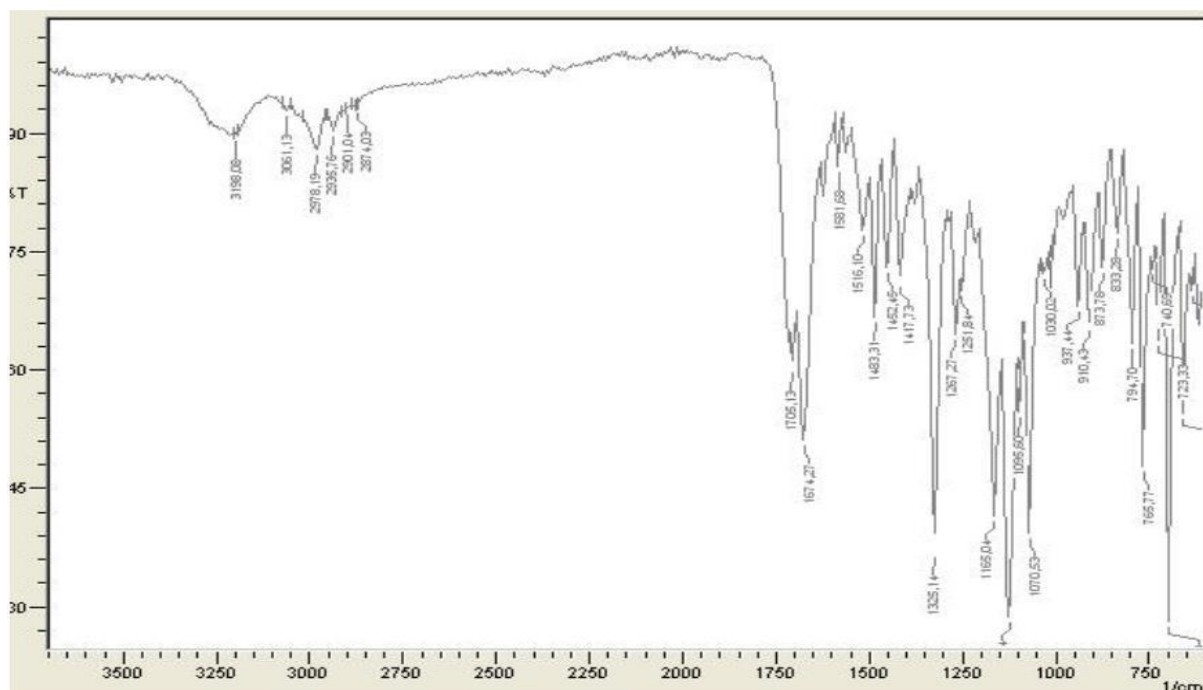
Figure S50: IR spectrum of the compound 4c
