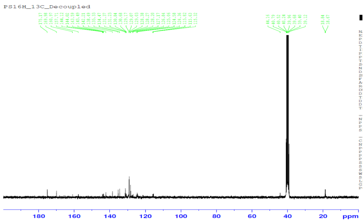
Figure S39: ^{13}\text{C} -NMR spectrum of the compound 3n
