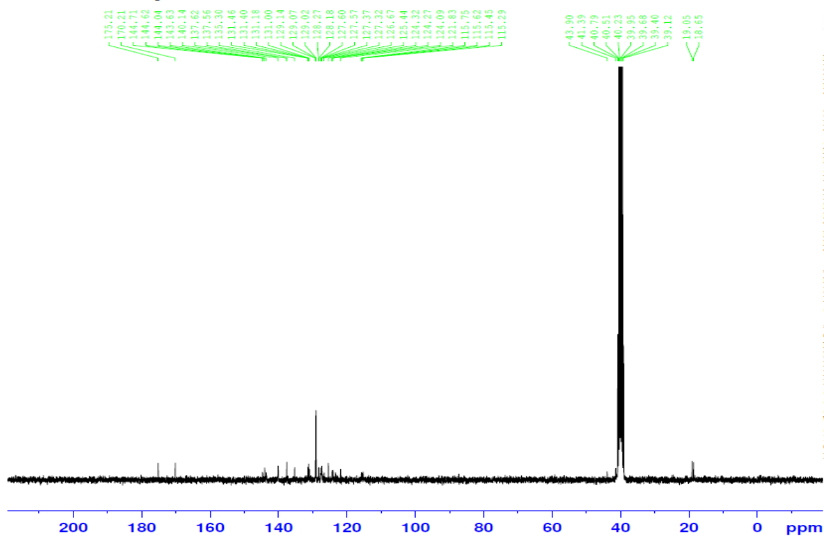
Figure S21: 13 C-NMR spectrum of the compound 3h
