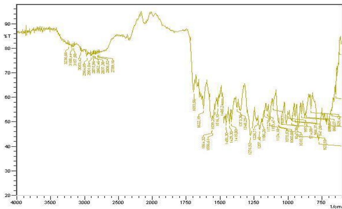
Figure S34: IR spectrum of the compound 3m
