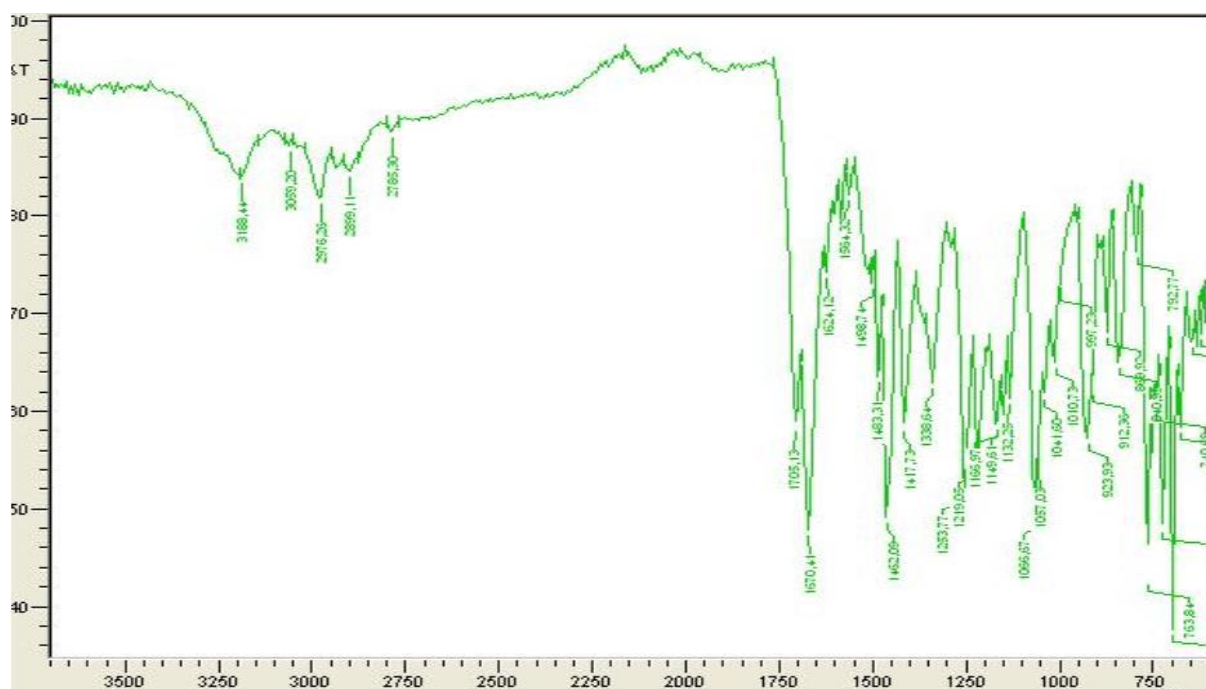
Figure S59: IR spectrum of the compound 4f
