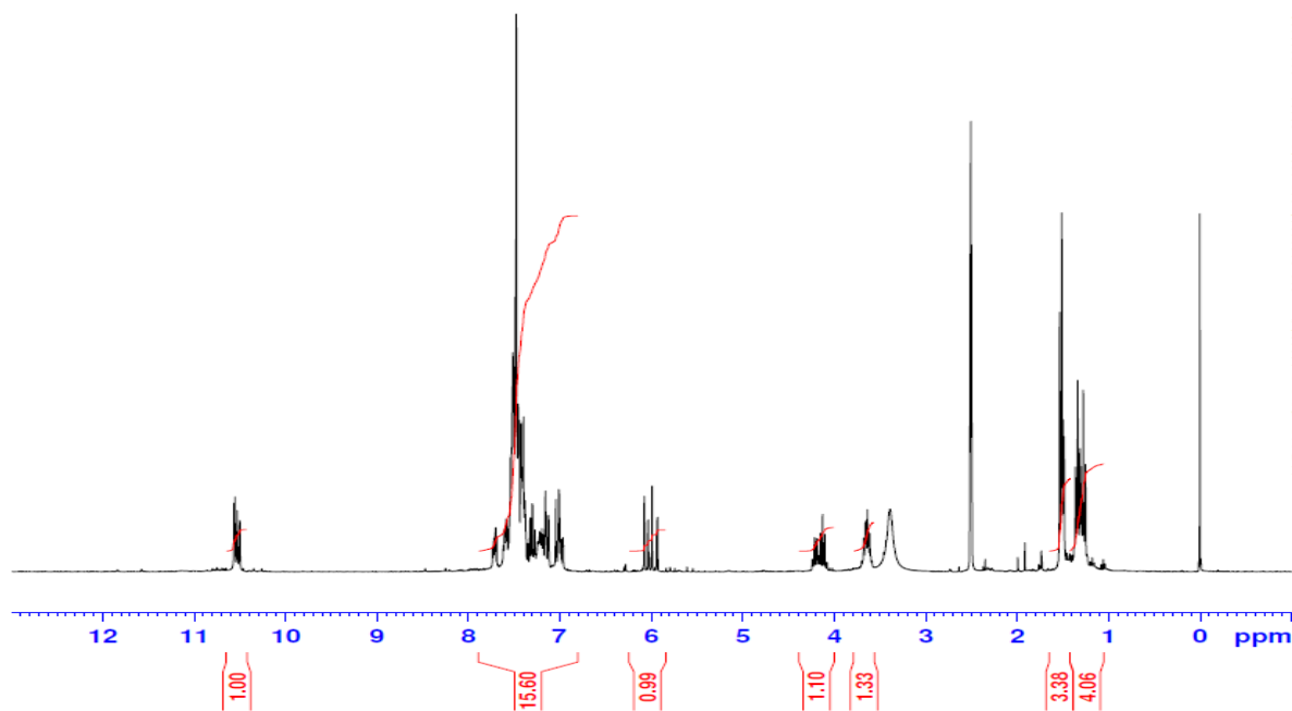
Figure S68: 1 H-NMR spectrum of the compound 4i
