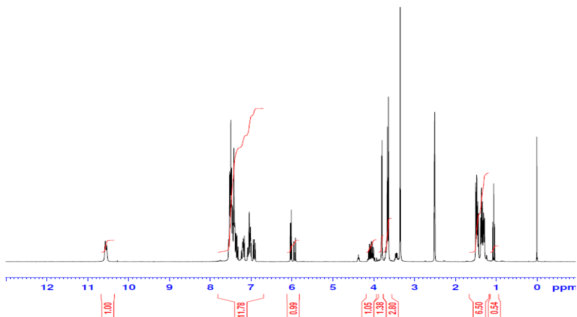
Figure S74: ^1\text{H} -NMR spectrum of the compound 4k
