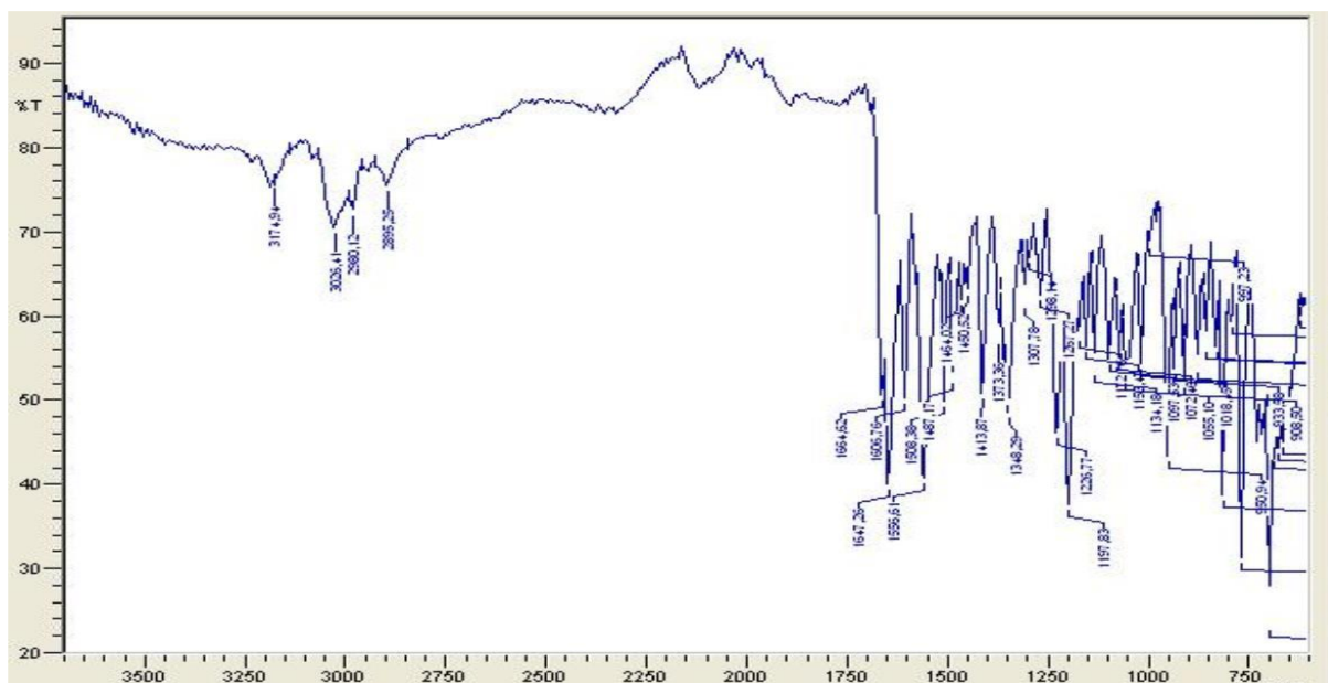
Figure S42: IR spectrum of the compound 3r
