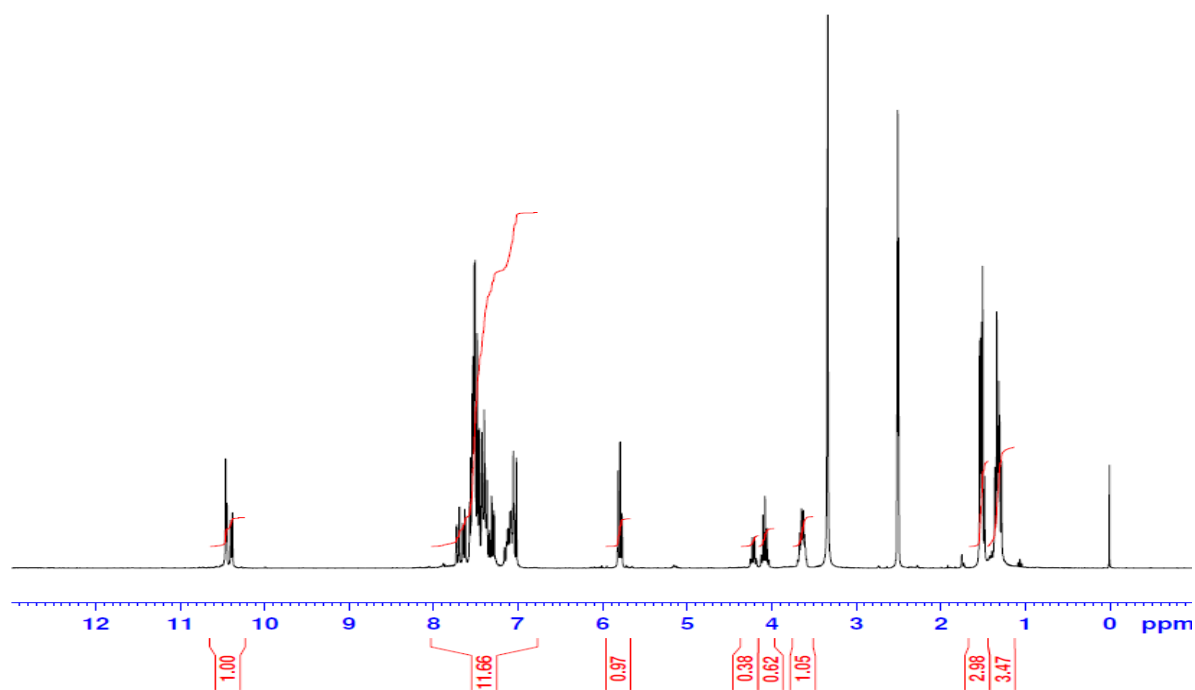
Figure S86: 1 H-NMR spectrum of the compound 4o
