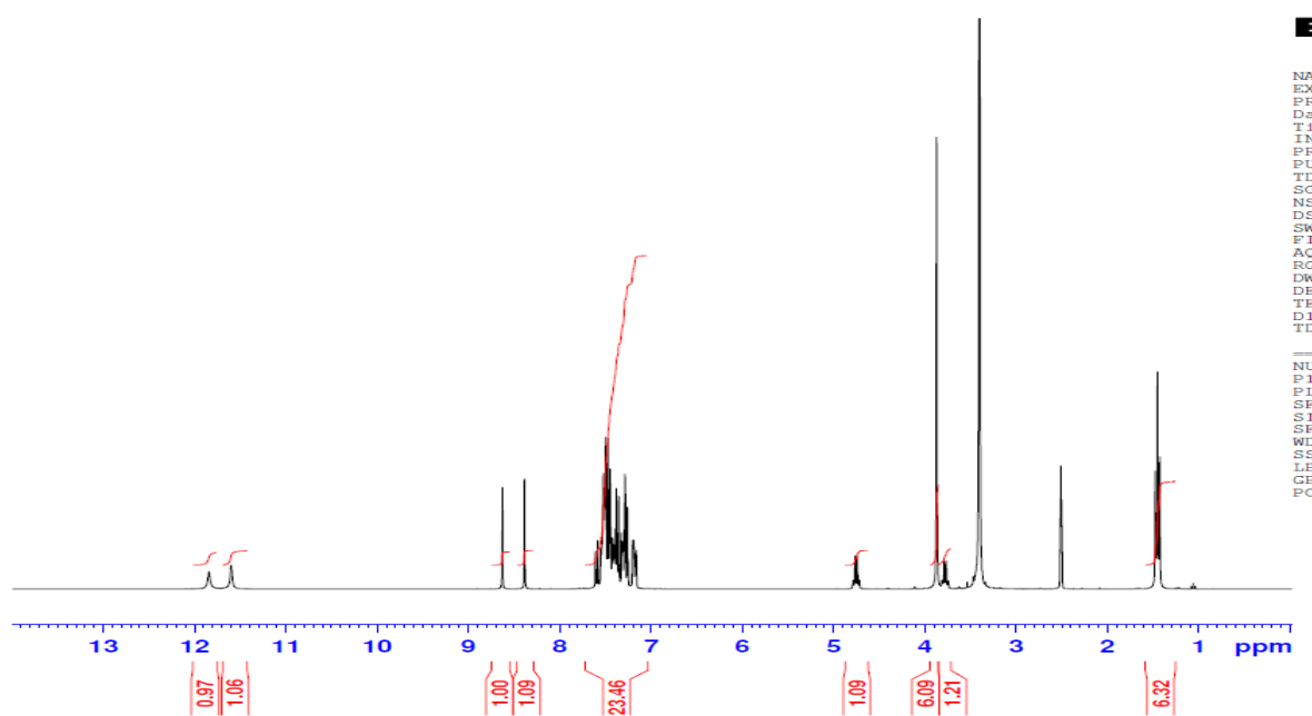
Figure S35: 1 H-NMR spectrum of the compound 3m
