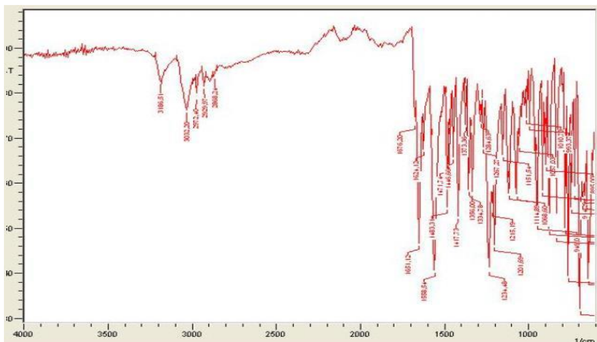
Figure S10: IR spectrum of the compound 3d
