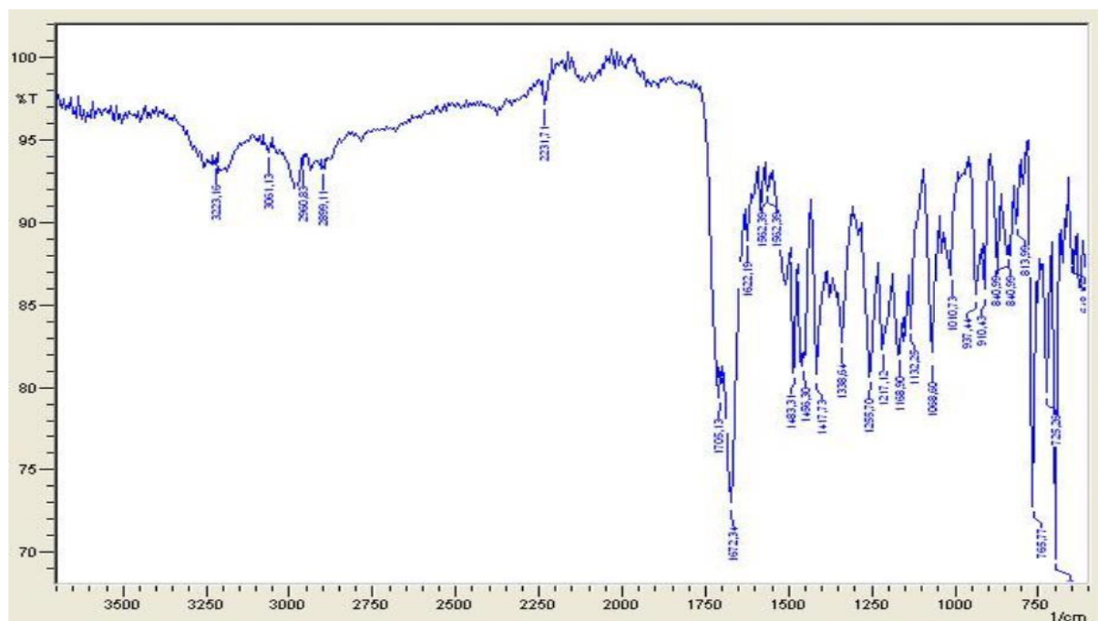
Figure S44: IR spectrum of the compound 4a
