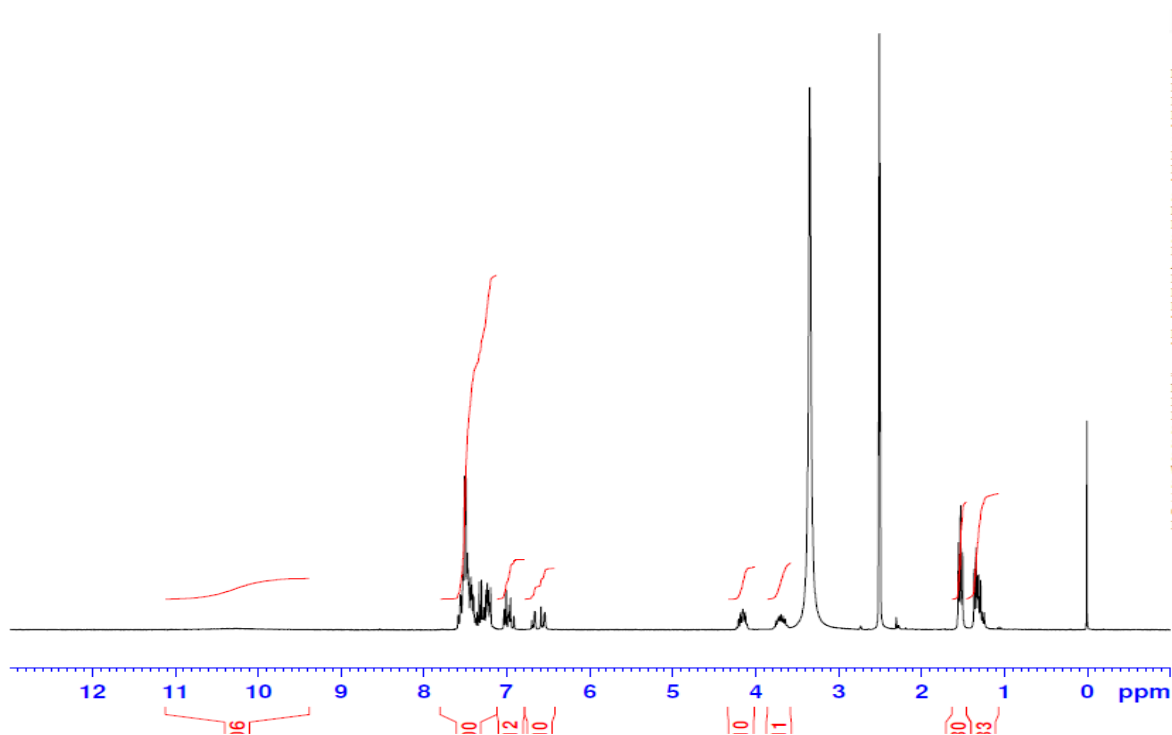
Figure S63: ^1\text{H} -NMR spectrum of the compound 4g
