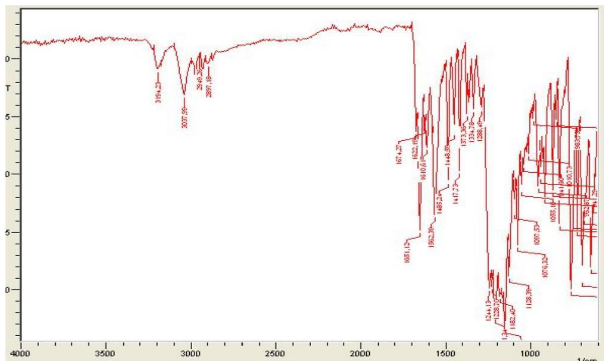
Figure S22: IR spectrum of the compound 3i
