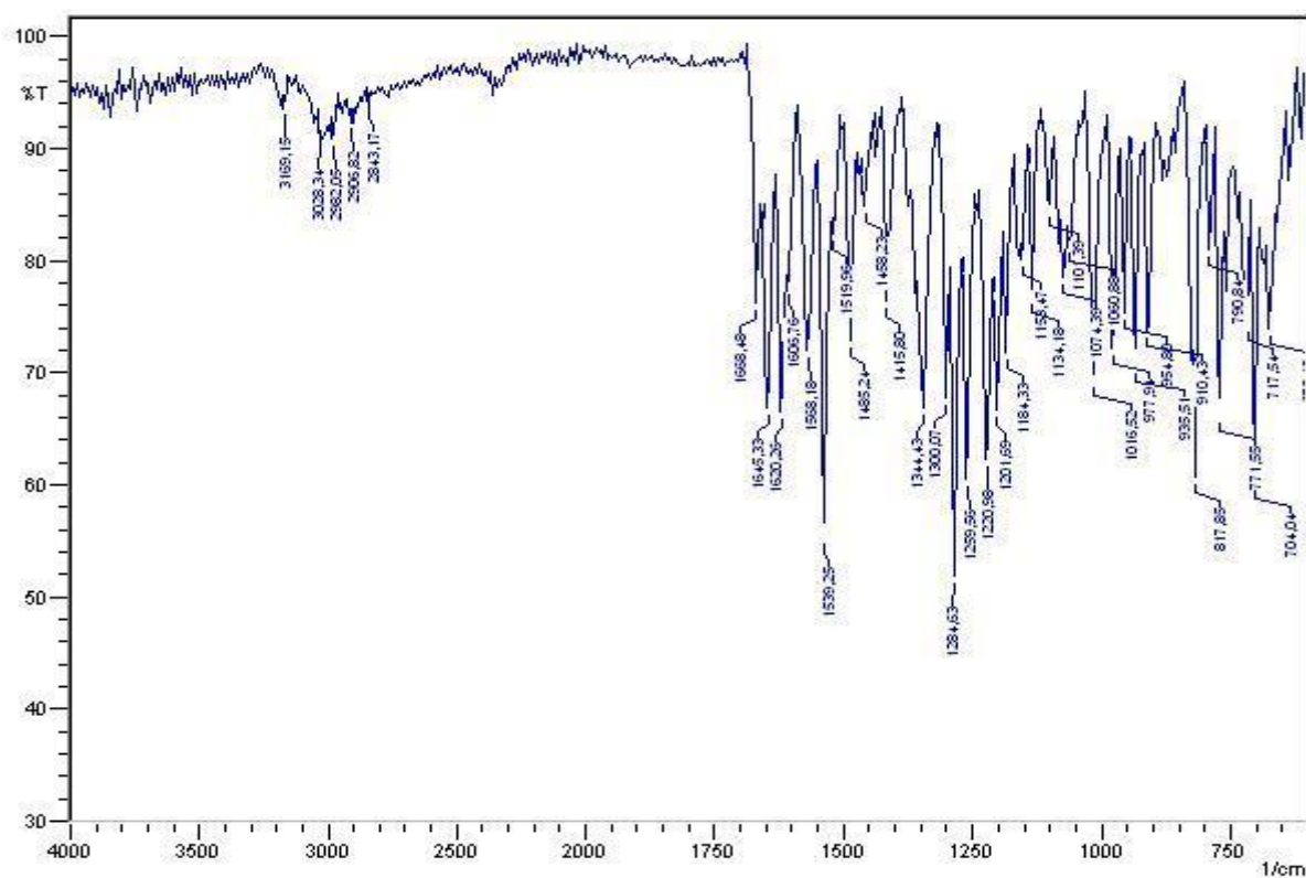
Figure S31: IR spectrum of the compound 3l
