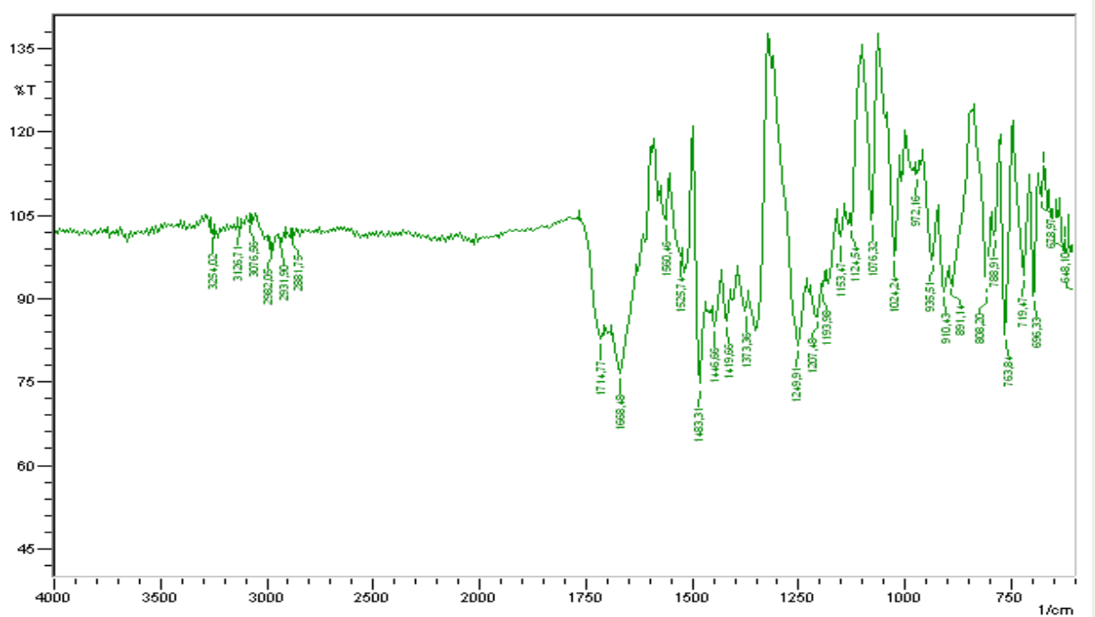
Figure S73: IR spectrum of the compound 4k
