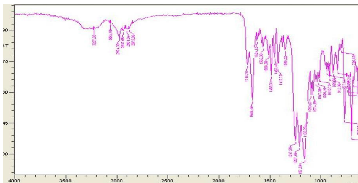
Figure S67: IR spectrum of the compound 4i
