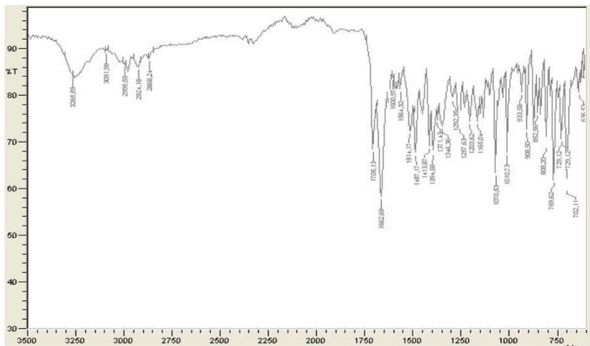
Figure S56: IR spectrum of the compound 4e
