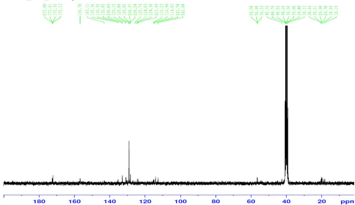
Figure S75: ^{13}\text{C} -NMR spectrum of the compound 4k
