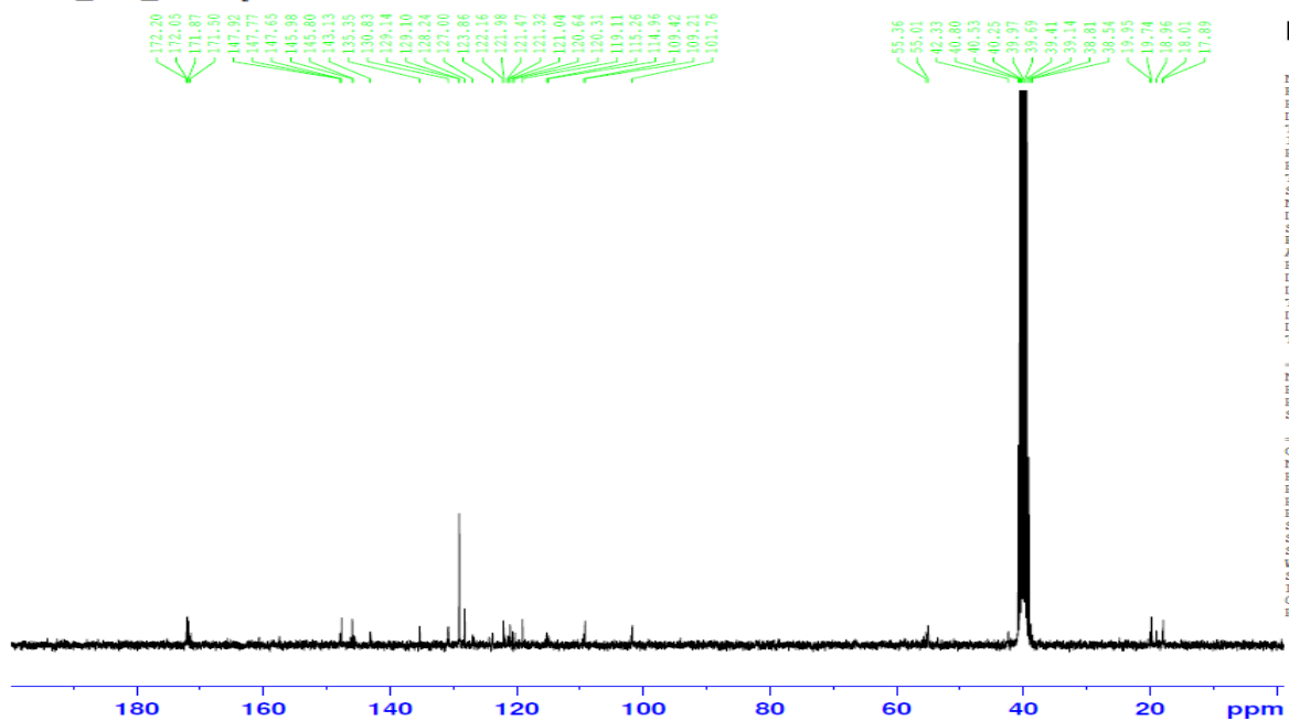
Figure S61: ^{13}\text{C} -NMR spectrum of the compound 4f
