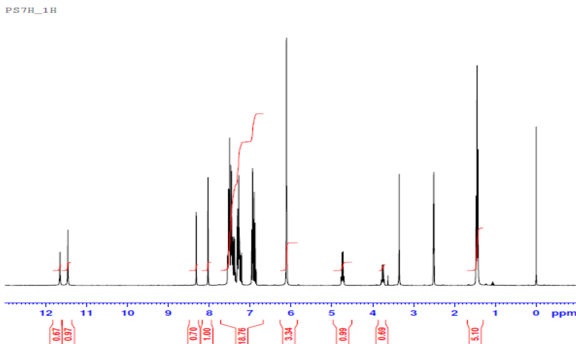
Figure S15: ^1\text{H} -NMR spectrum of the compound 3f
