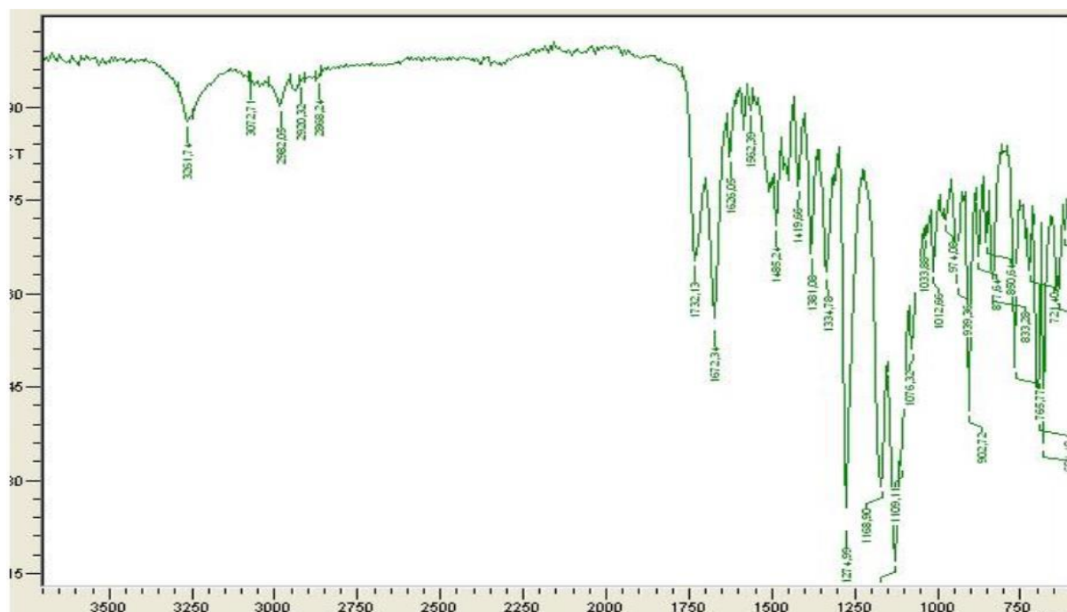
Figure S64: IR spectrum of the compound 4h
