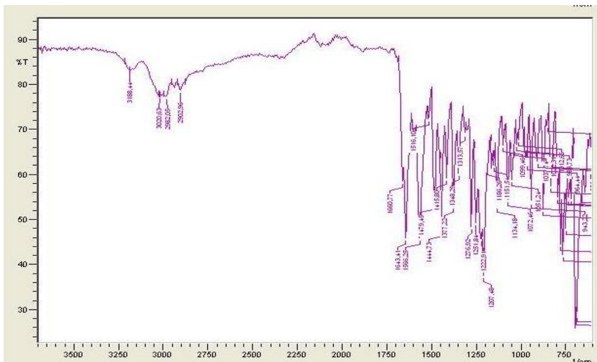
Figure S4: IR spectrum of the compound 3b
