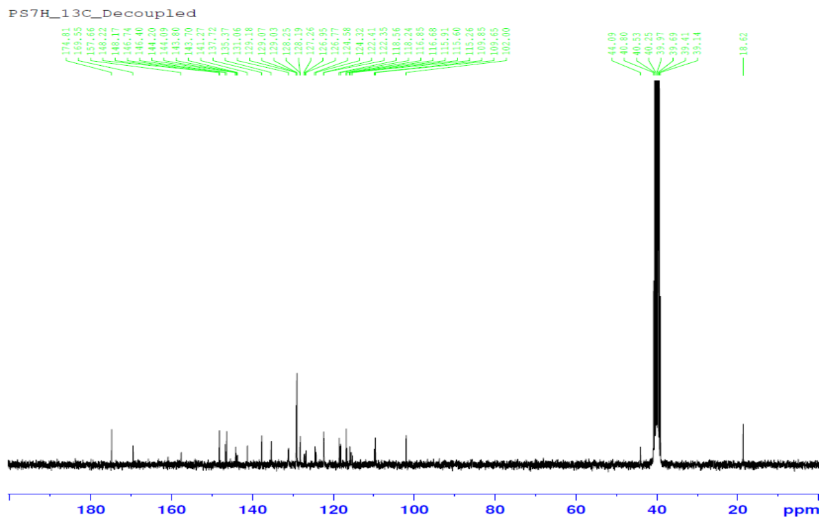
Figure S16: ^{13}\text{C} -NMR spectrum of the compound 3f
