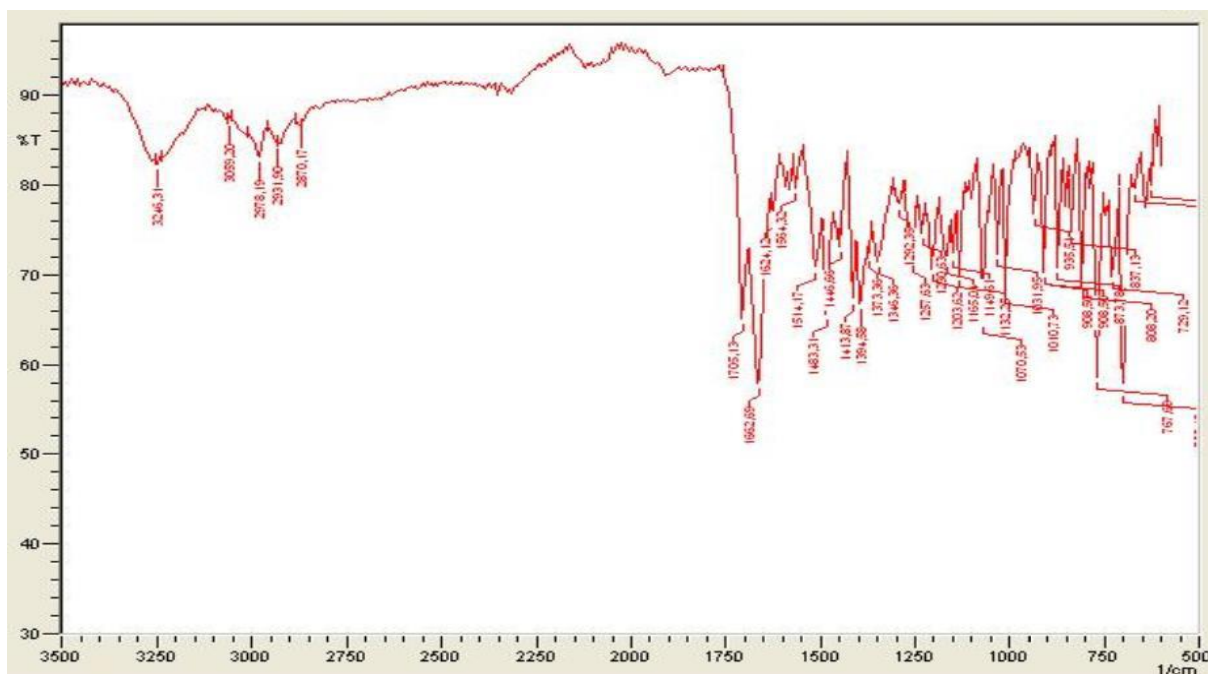
Figure S85: IR spectrum of the compound 4o
