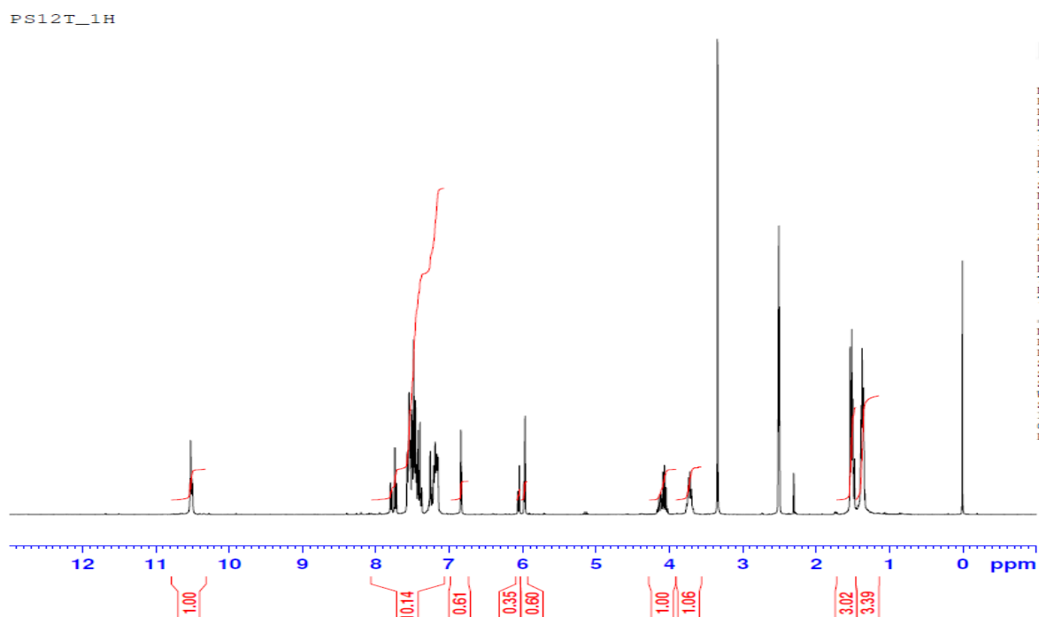
Figure S71: ^1\text{H} -NMR spectrum of the compound 4j
