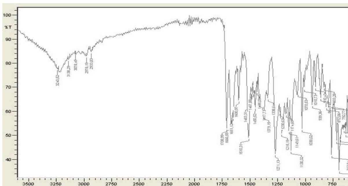
Figure S93: IR spectrum of the compound 4s
