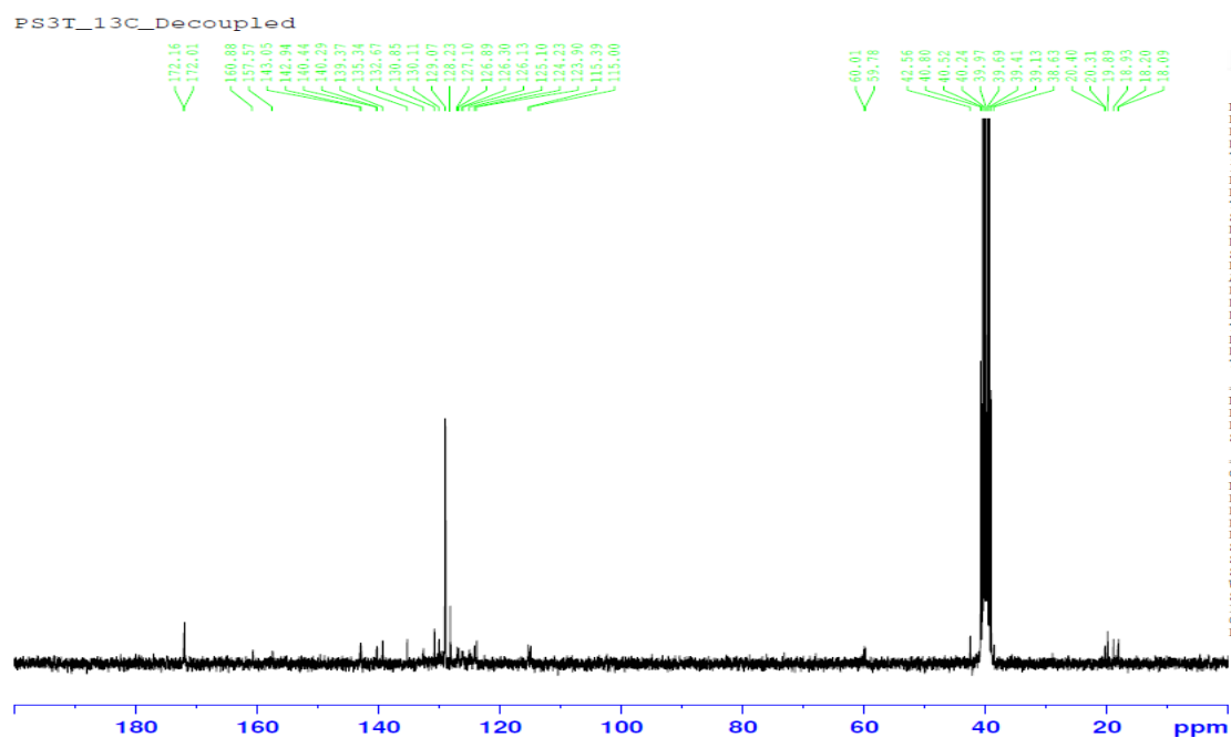
Figure S52: ^{13}\text{C} -NMR spectrum of the compound 4c
