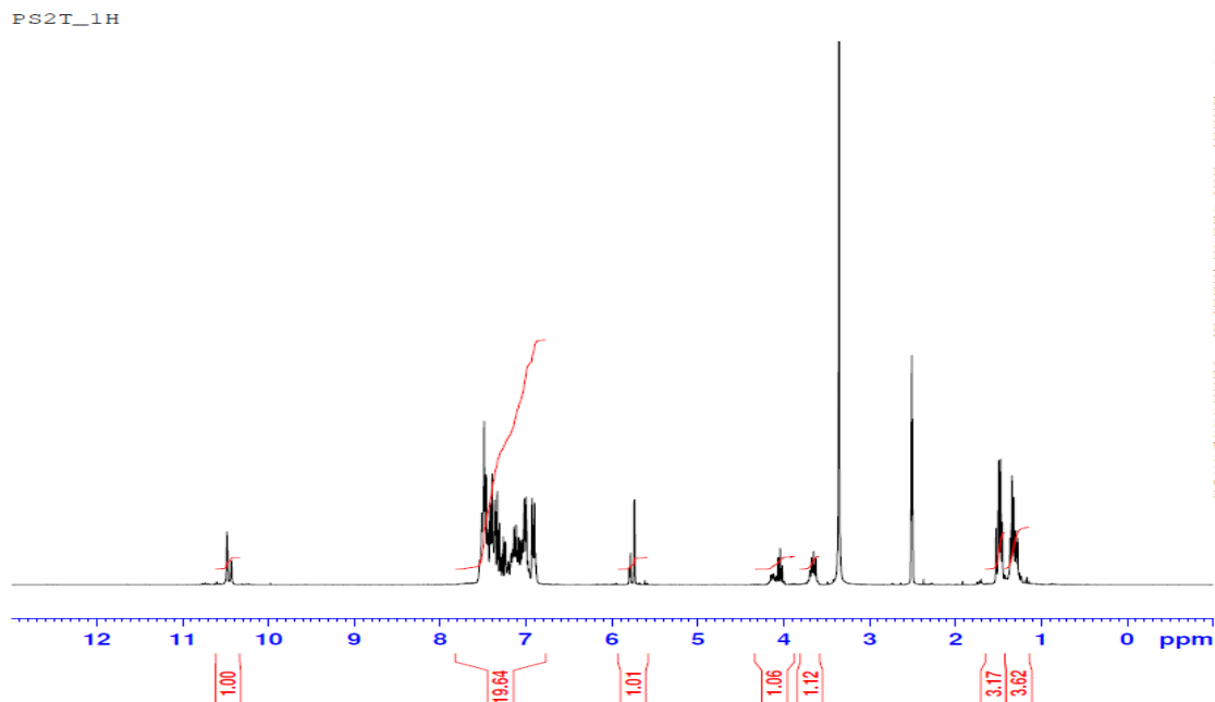
Figure S48: ^1\text{H} -NMR spectrum of the compound 4b
