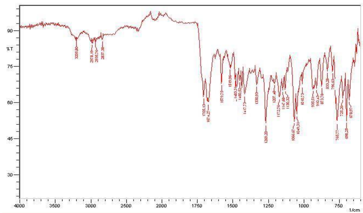
Figure S79: IR spectrum of the compound 4m
