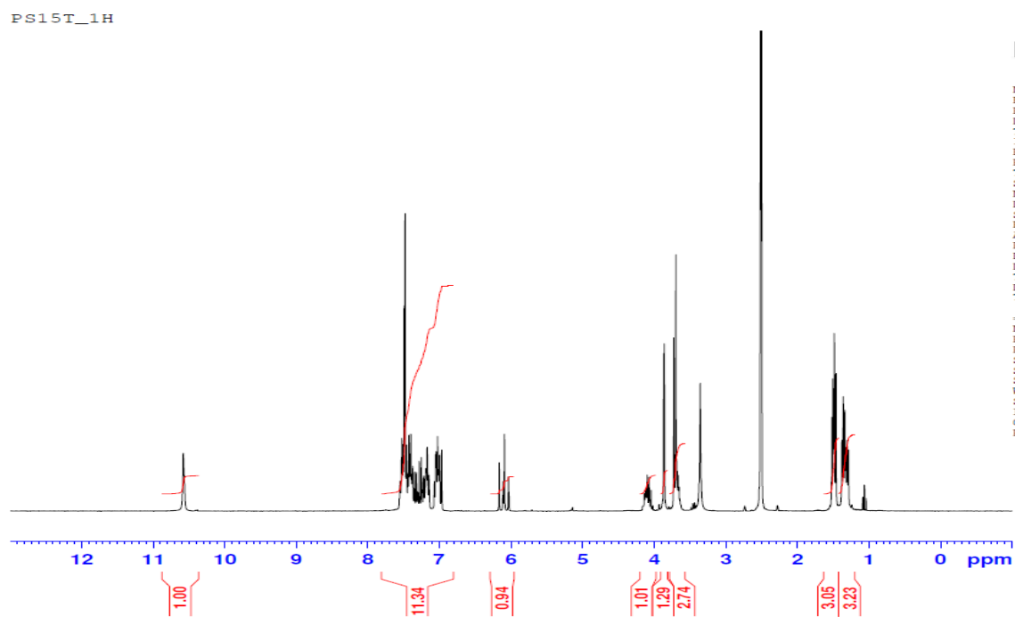
Figure S80: ^1\text{H} -NMR spectrum of the compound 4m
