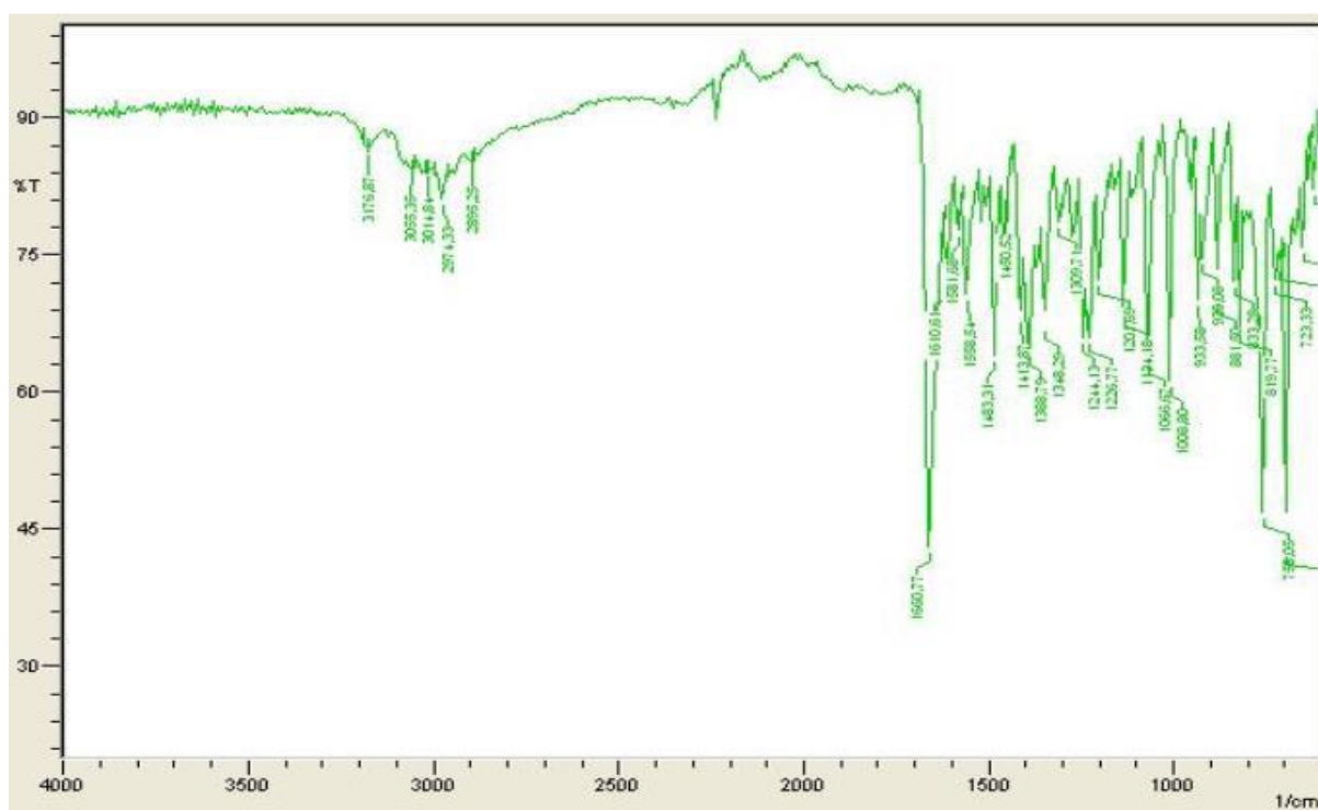
Figure S11: IR spectrum of the compound 3e
