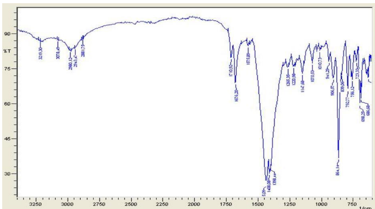
Figure S62: IR spectrum of the compound 4g
