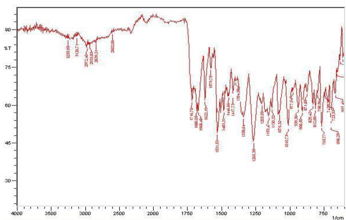
Figure S76: IR spectrum of the compound 4l
