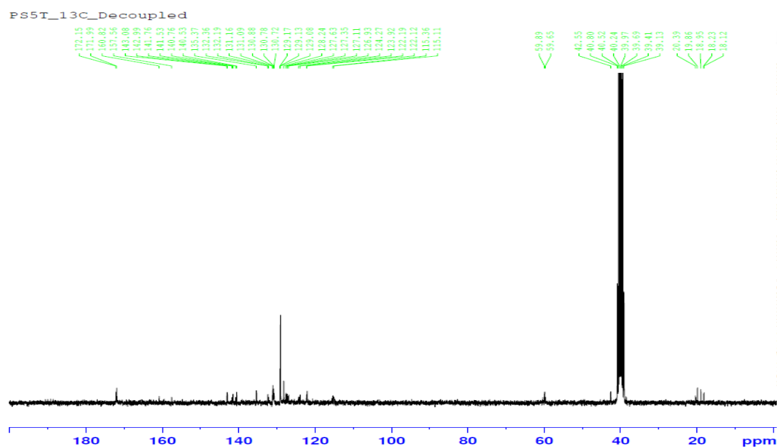
Figure S55: ^{13}\text{C} -NMR spectrum of the compound 4d
