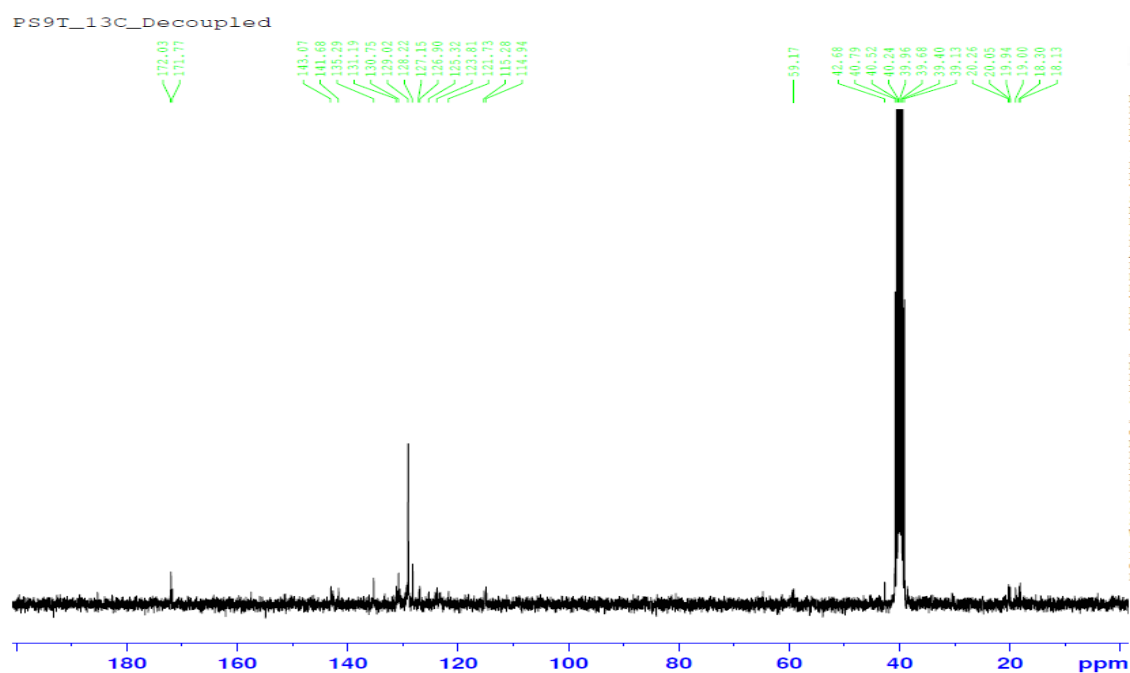
Figure S66: ^{13}\text{C} -NMR spectrum of the compound 4h
