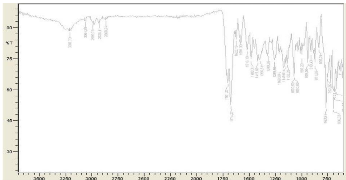
Figure S53: IR spectrum of the compound 4d
