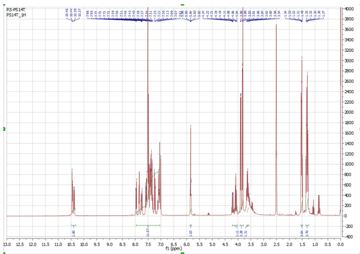
Figure S77: ^1\text{H} -NMR spectrum of the compound 4l
