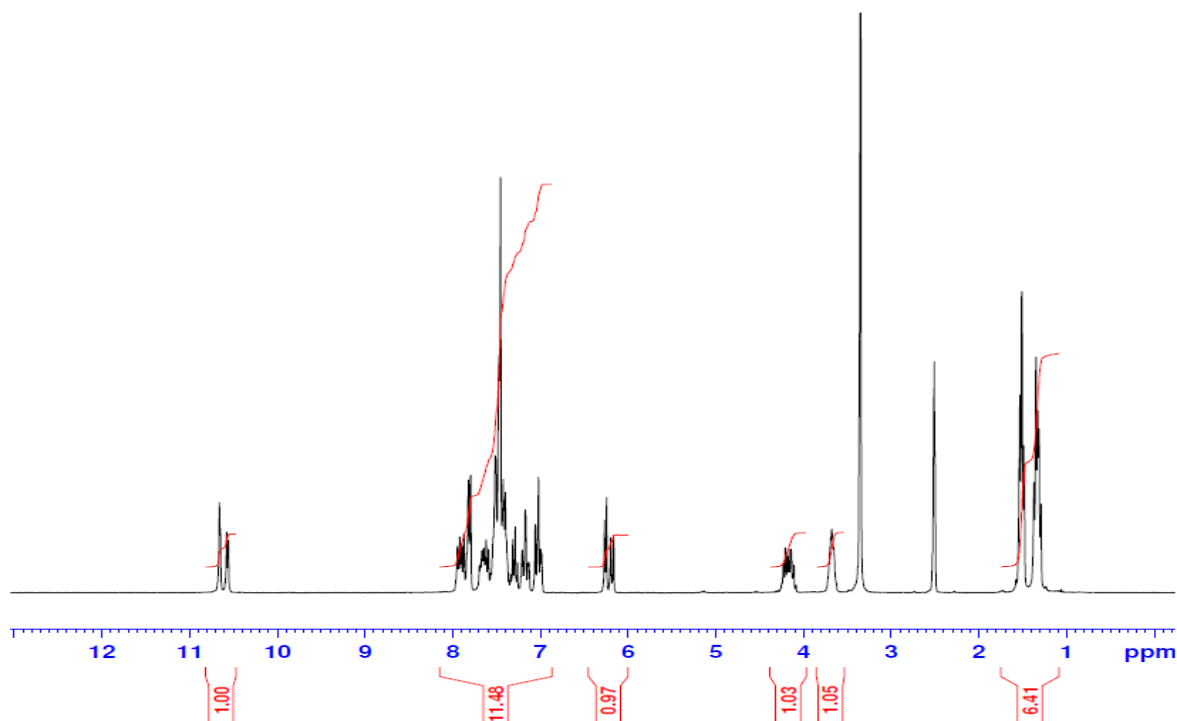
Figure S83: ^1\text{H} -NMR spectrum of the compound 4n
