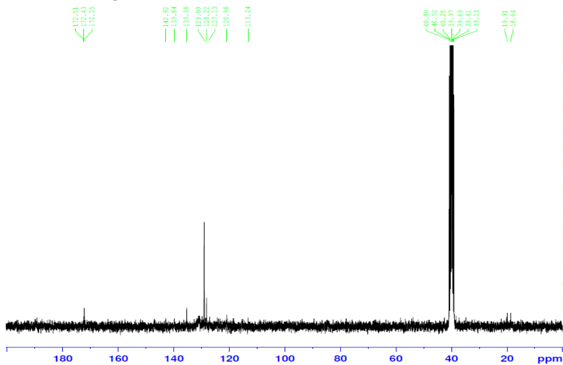
Figure S69: 13 C-NMR spectrum of the compound 4i
