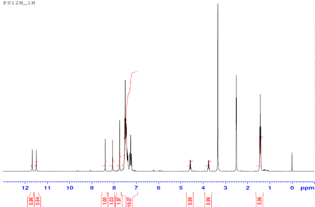
Figure S26: 1 H-NMR spectrum of the compound 3j
