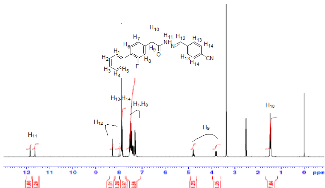
Figure S2: ^1\text{H} -NMR spectrum of the compound 3a
