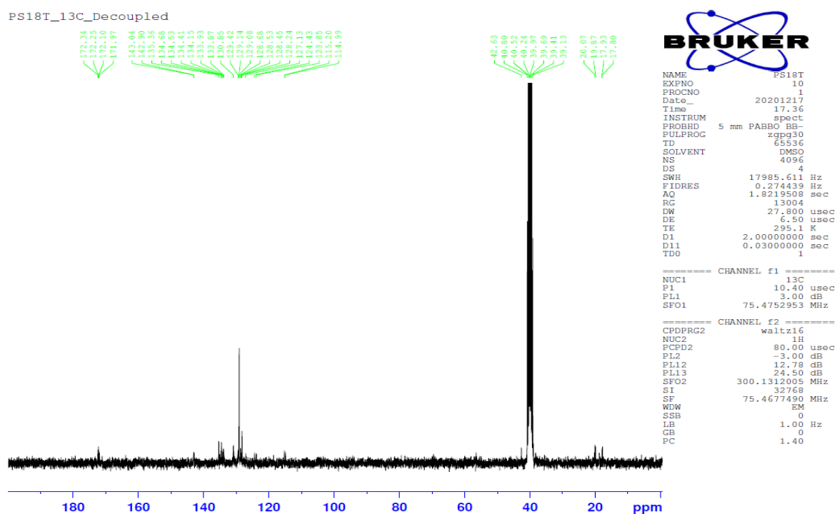
Figure S89: ^{13}\text{C} -NMR spectrum of the compound 4p
