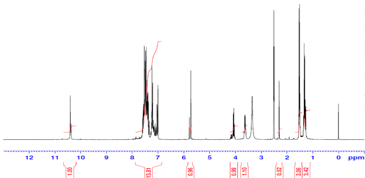
Figure S57: ^1\text{H} -NMR spectrum of the compound 4e
