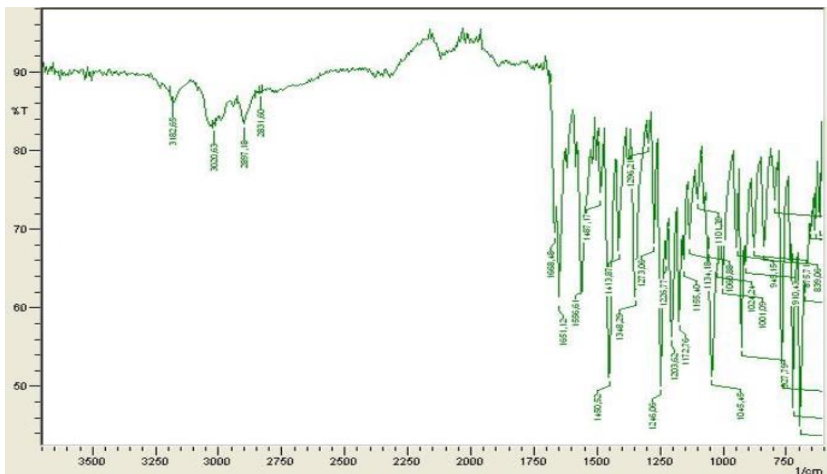
Figure S14: IR spectrum of the compound 3f
