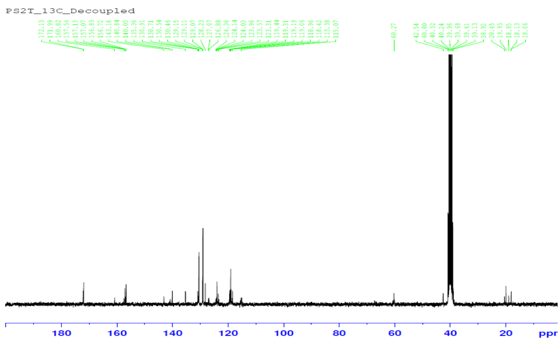
Figure S49: ^{13}\text{C} -NMR spectrum of the compound 4b
