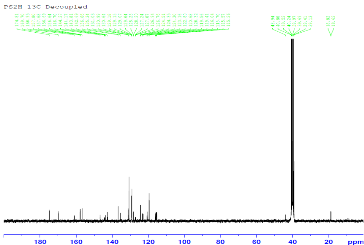
Figure S6: ^{13}\text{C} -NMR spectrum of the compound 3b
