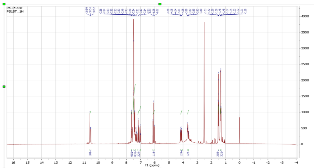
Figure S88: ^1\text{H} -NMR spectrum of the compound 4p
