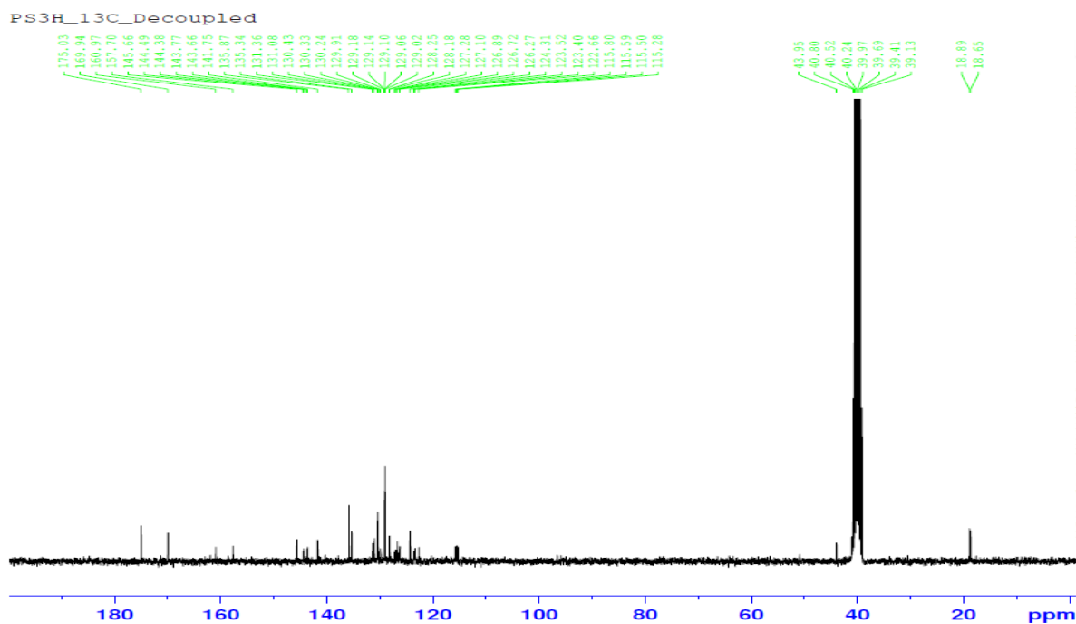
Figure S9: 13 C-NMR spectrum of the compound 3c
