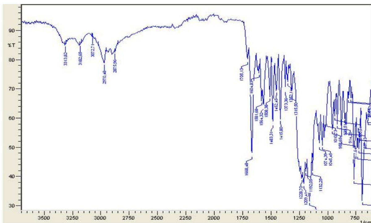
Figure S47: IR spectrum of the compound 4b
