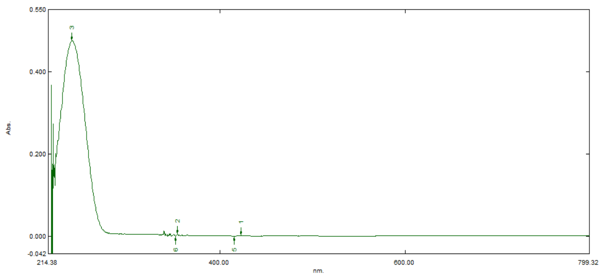
Figure S2: Identification of SPI using UV-Spectrophotometer
