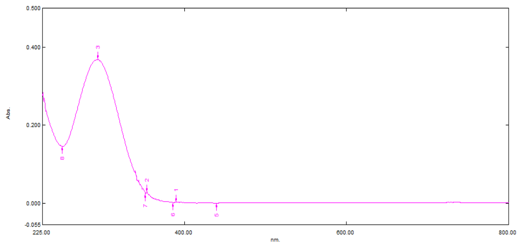
Figure S1: Identification of TOR using UV-Spectrophotometer
