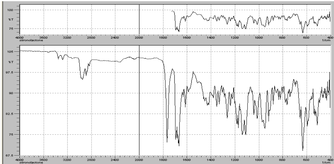
Figure S4 : Reference IR spectra of SPI
