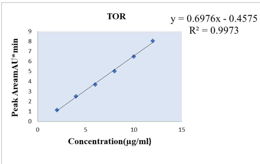
Figure S5 : Calibration curve of TOR
