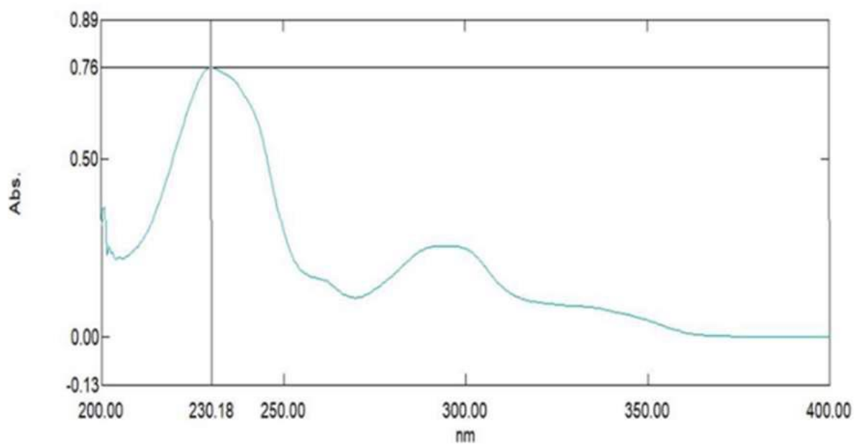
Figure 2: UV spectra of Desidustat
