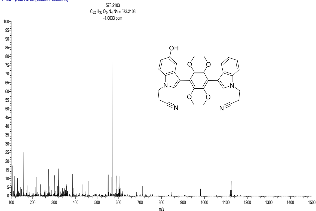
Figure S27: HRESIMS spectrum of compound 9
