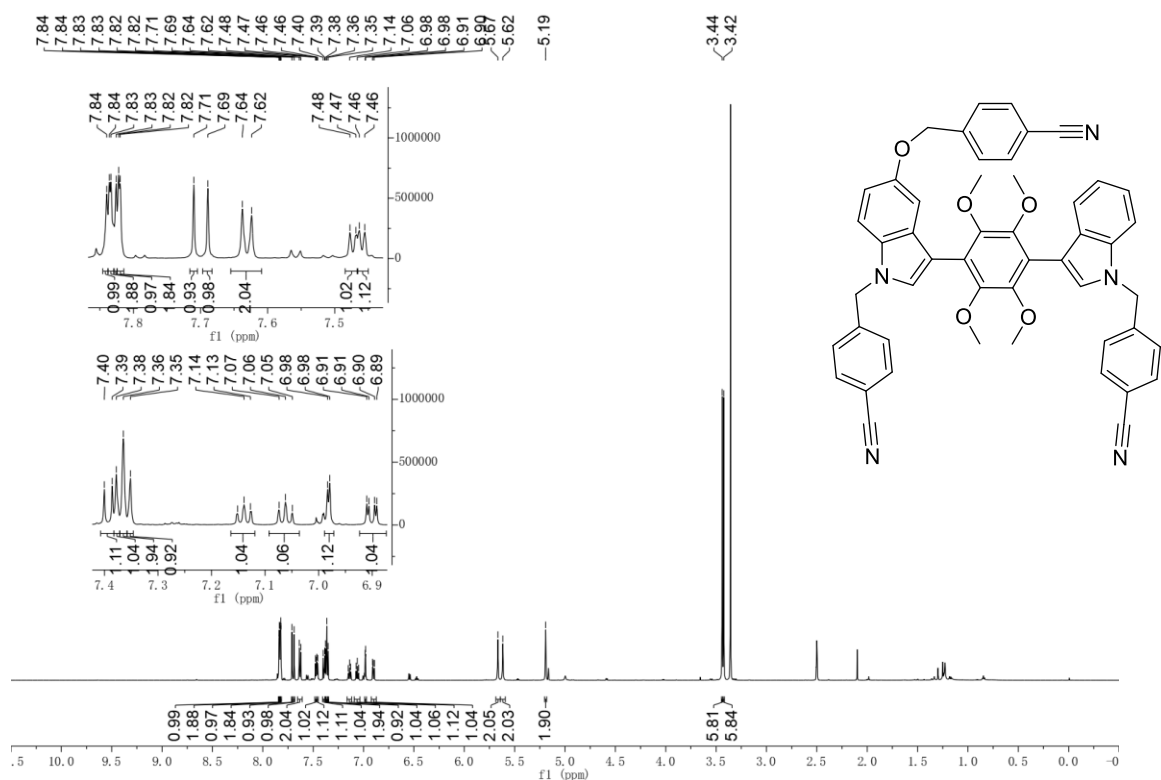
Figure S37: 1 H-NMR (600 MHz, DMSO- d 6 ) spectrum of compound 13
