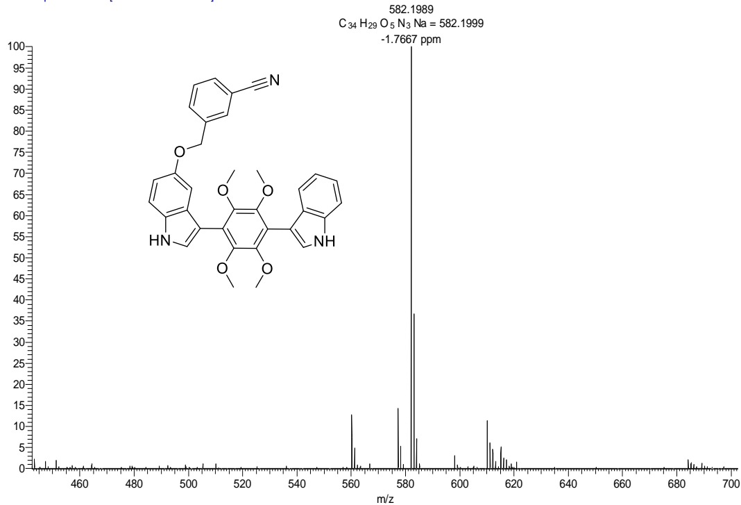
Figure S18: HRESIMS spectrum of compound 6
