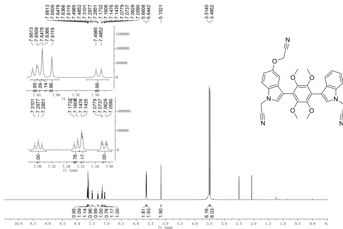
Figure S22: 1 H-NMR (600 MHz, DMSO- d 6 ) spectrum of compound 8
