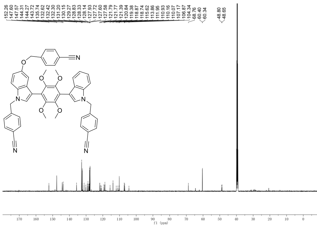
Figure S38: 13 C-NMR (150 MHz, DMSO- d 6 ) spectrum of compound 13
