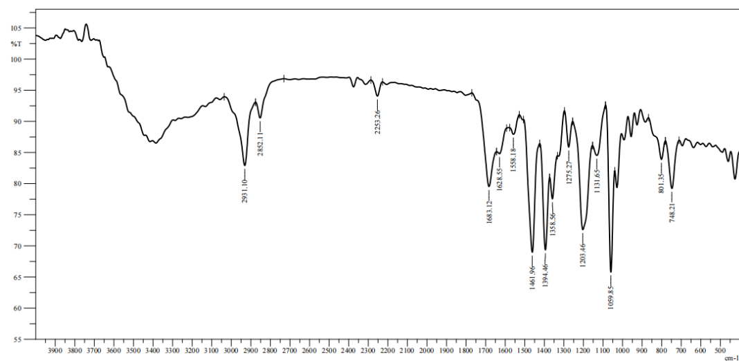
Figure S54: Infrared (IR) spectrum of compound 9 (KBr pellet)
