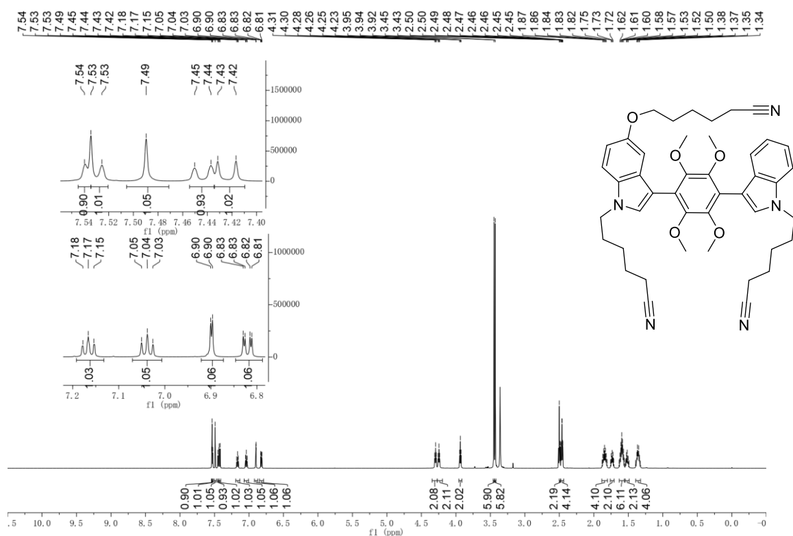
Figure S33: HRESIMS spectrum of compound 11
