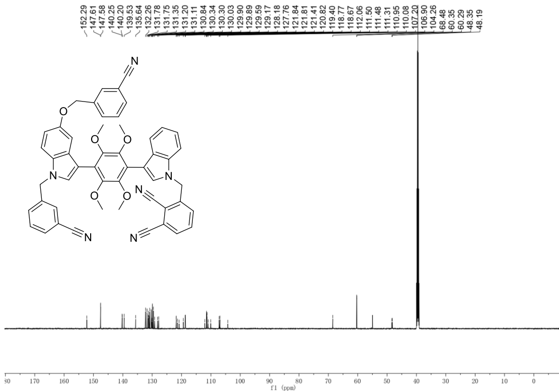
Figure S44: 13 C-NMR (150 MHz, DMSO- d 6 ) spectrum of compound 15
