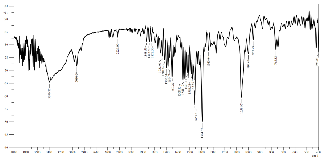
Figure S52: Infrared (IR) spectrum of compound 7 (KBr pellet)
