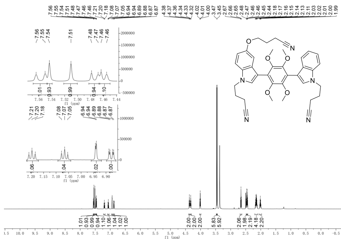
Figure S27: HRESIMS spectrum of compound 9
