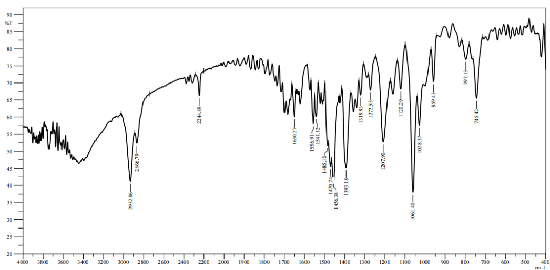
Figure S57: Infrared (IR) spectrum of compound 12 (KBr pellet)
