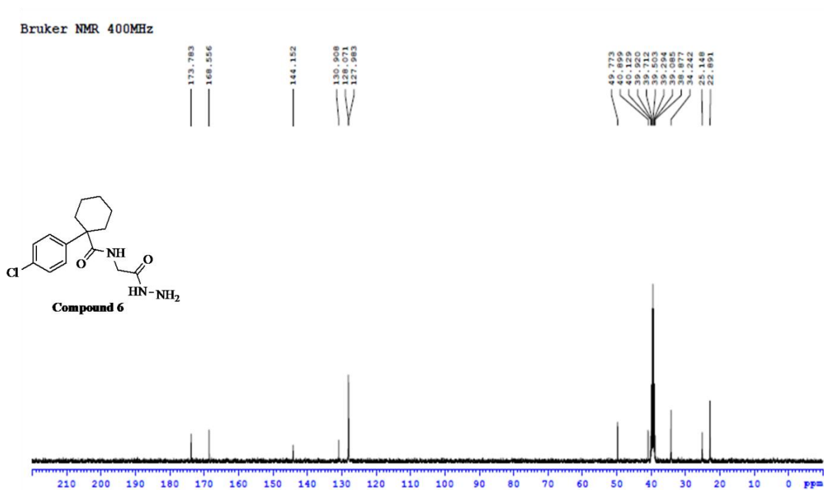
Figure S14: 13 C NMR spectrum of compound 6
