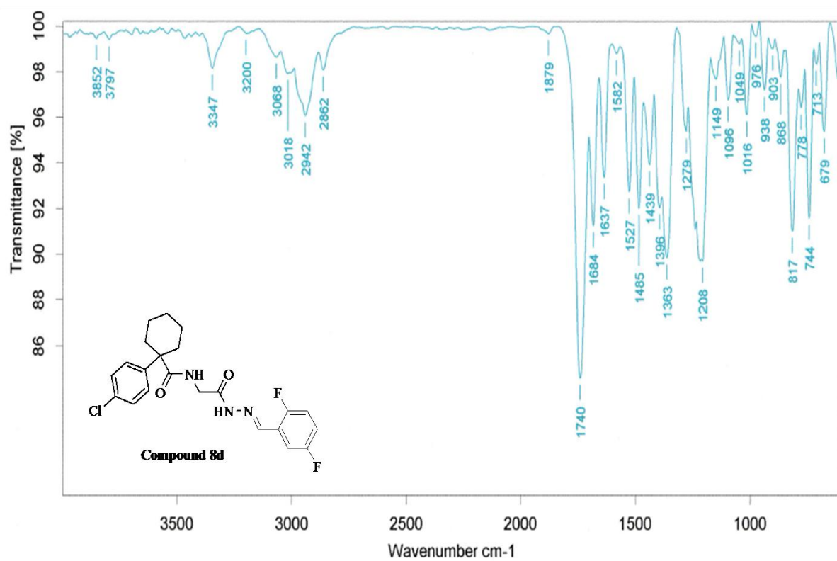
Figure S31: FT-IR spectrum of compound 8d
