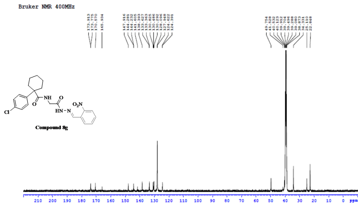
Figure S42: 13 C NMR spectrum of compound 8g
