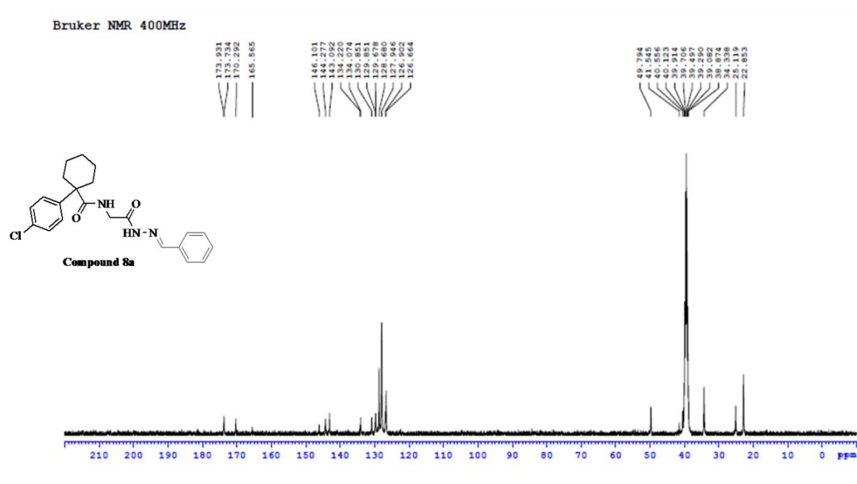
Figure S18: 13 C NMR spectrum of compound 8a
