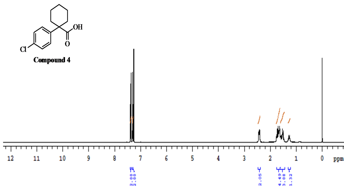
Figure S5: ^1\text{H} NMR spectrum of compound 4
