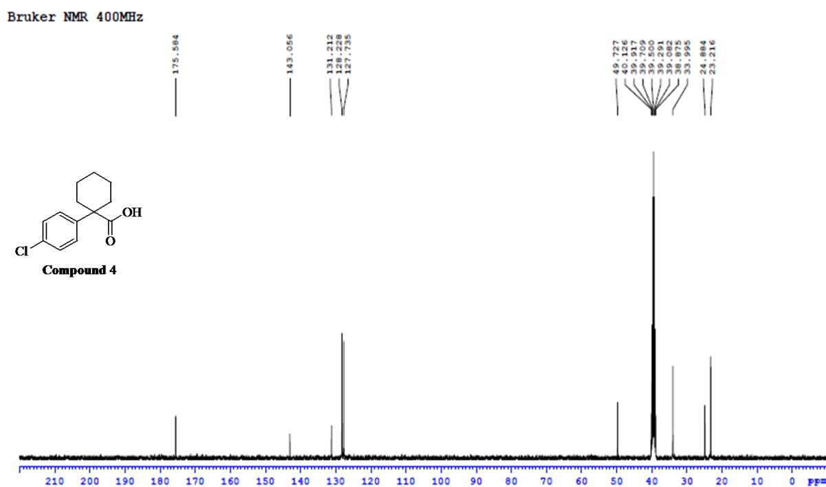
Figure S6: ^{13}\text{C} NMR spectrum of compound 4
