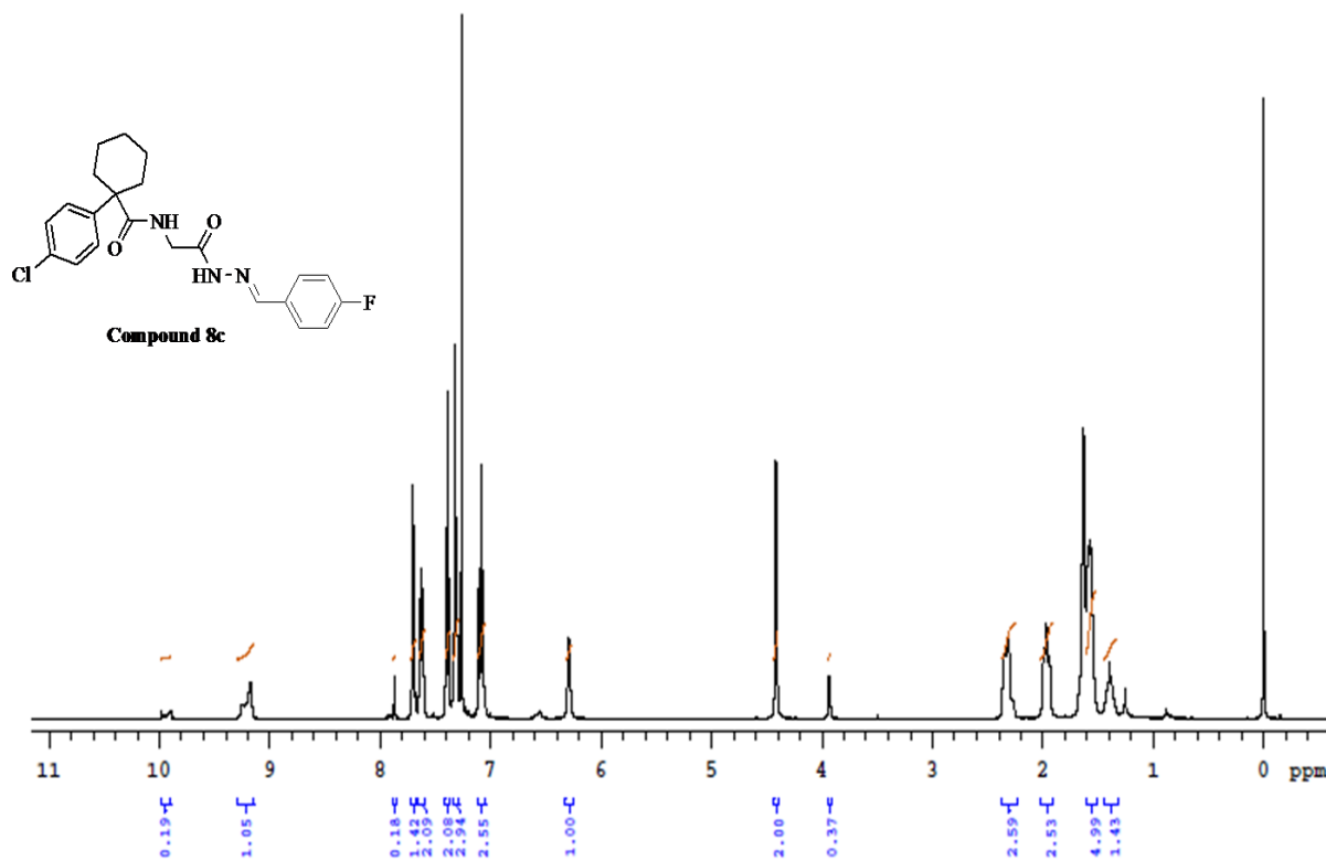
Figure S25: 1 H NMR spectrum of compound 8c
