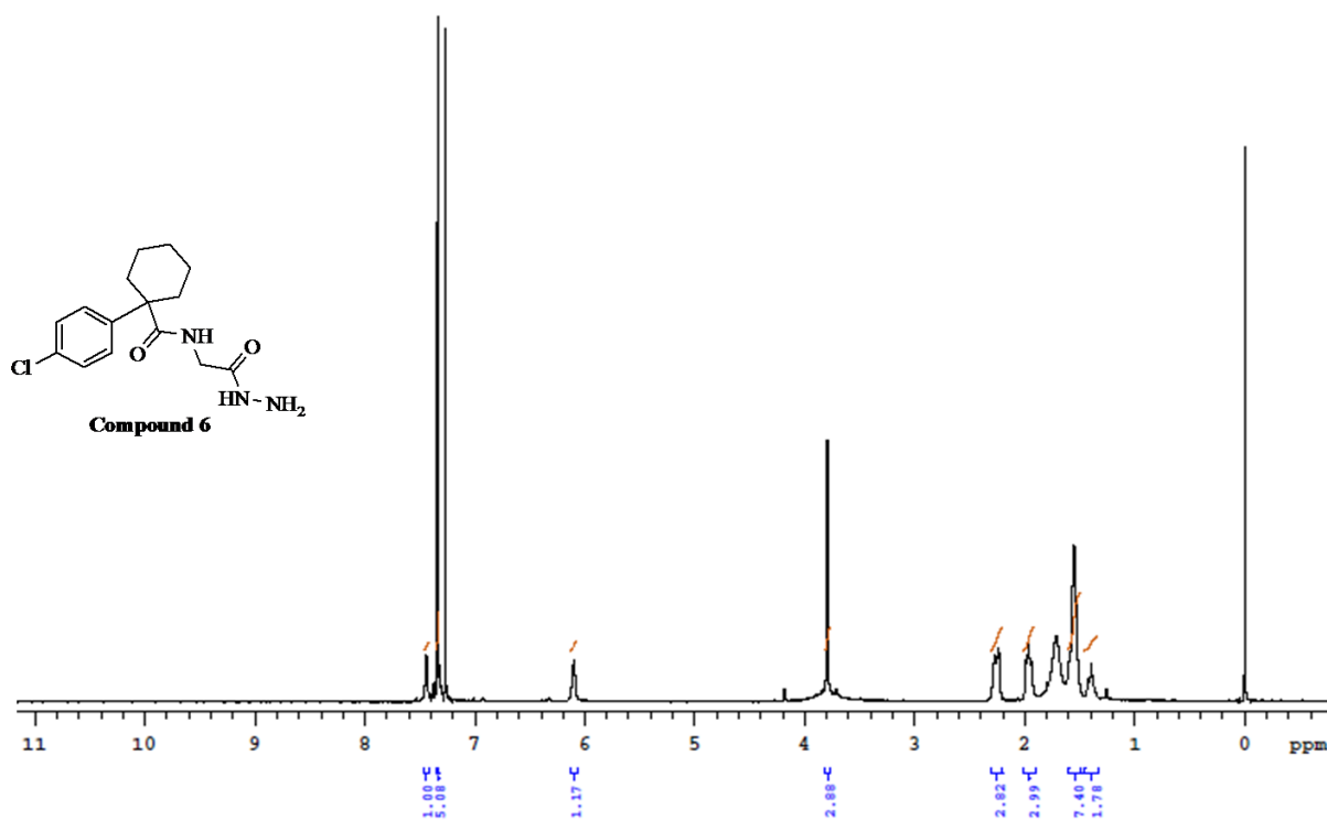
Figure S13: 1 H NMR spectrum of compound 6
