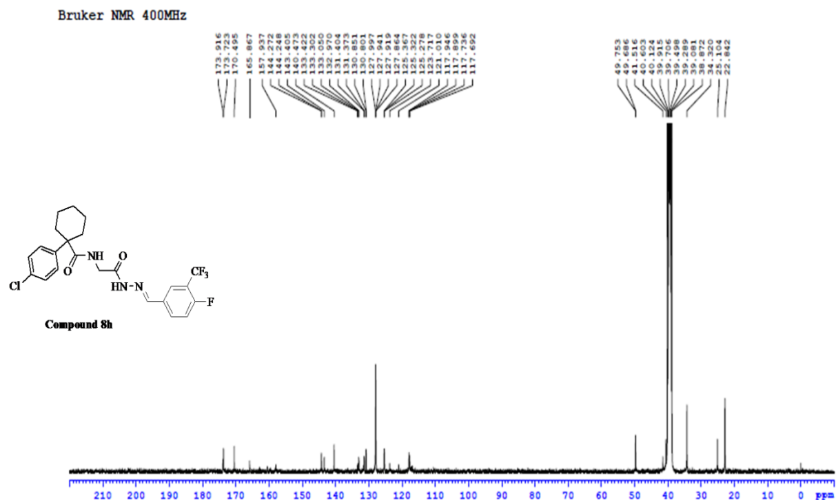
Figure S46: ^{13}\text{C} NMR spectrum of compound 8h
