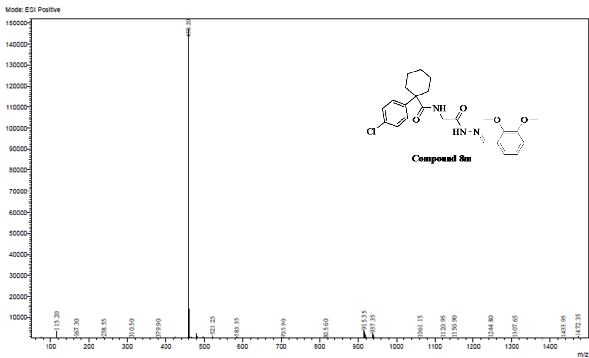
Figure S68: ESI-MS spectrum of compound 8m
