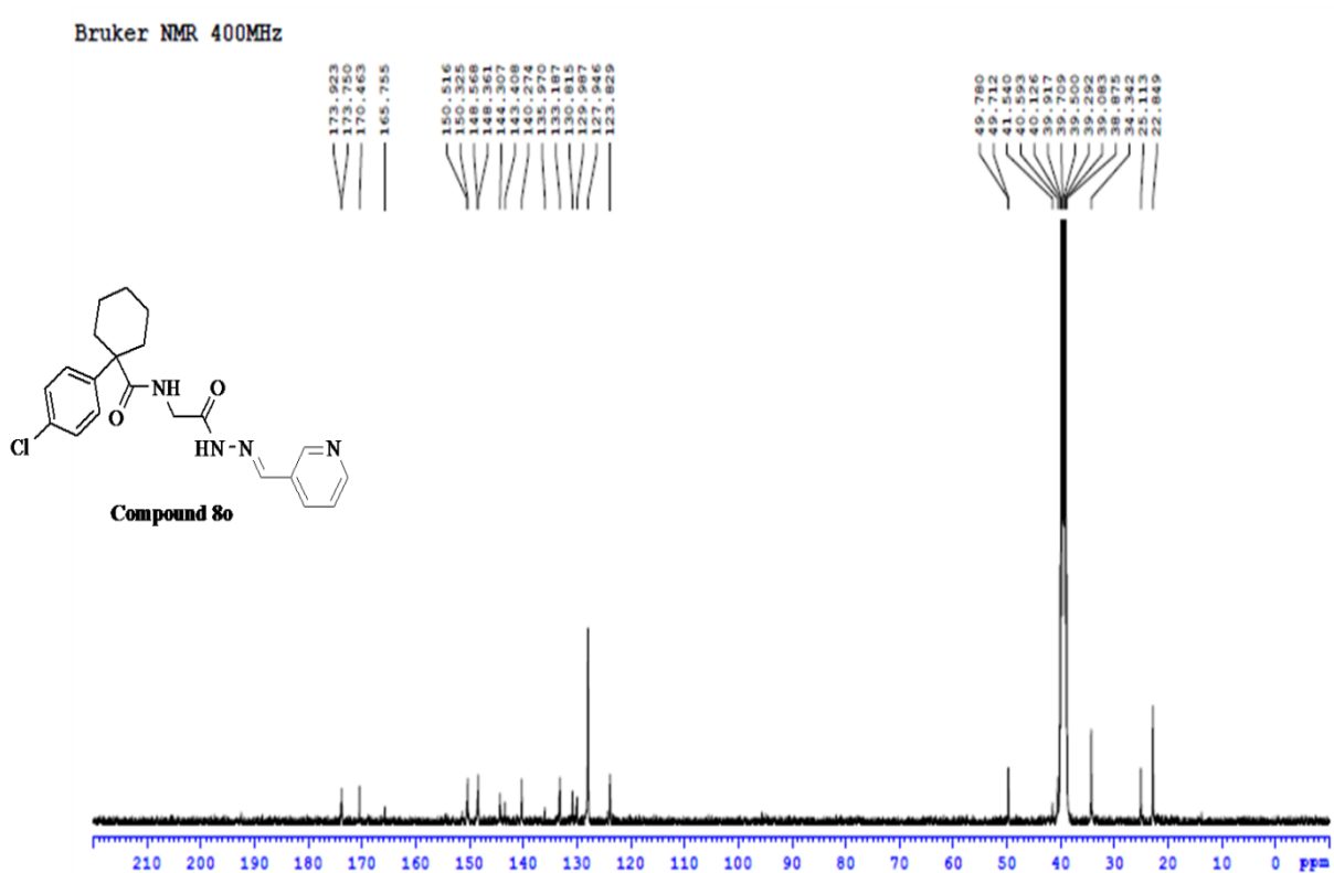
Figure S74: ^{13}\text{C} NMR spectrum of compound 8o
