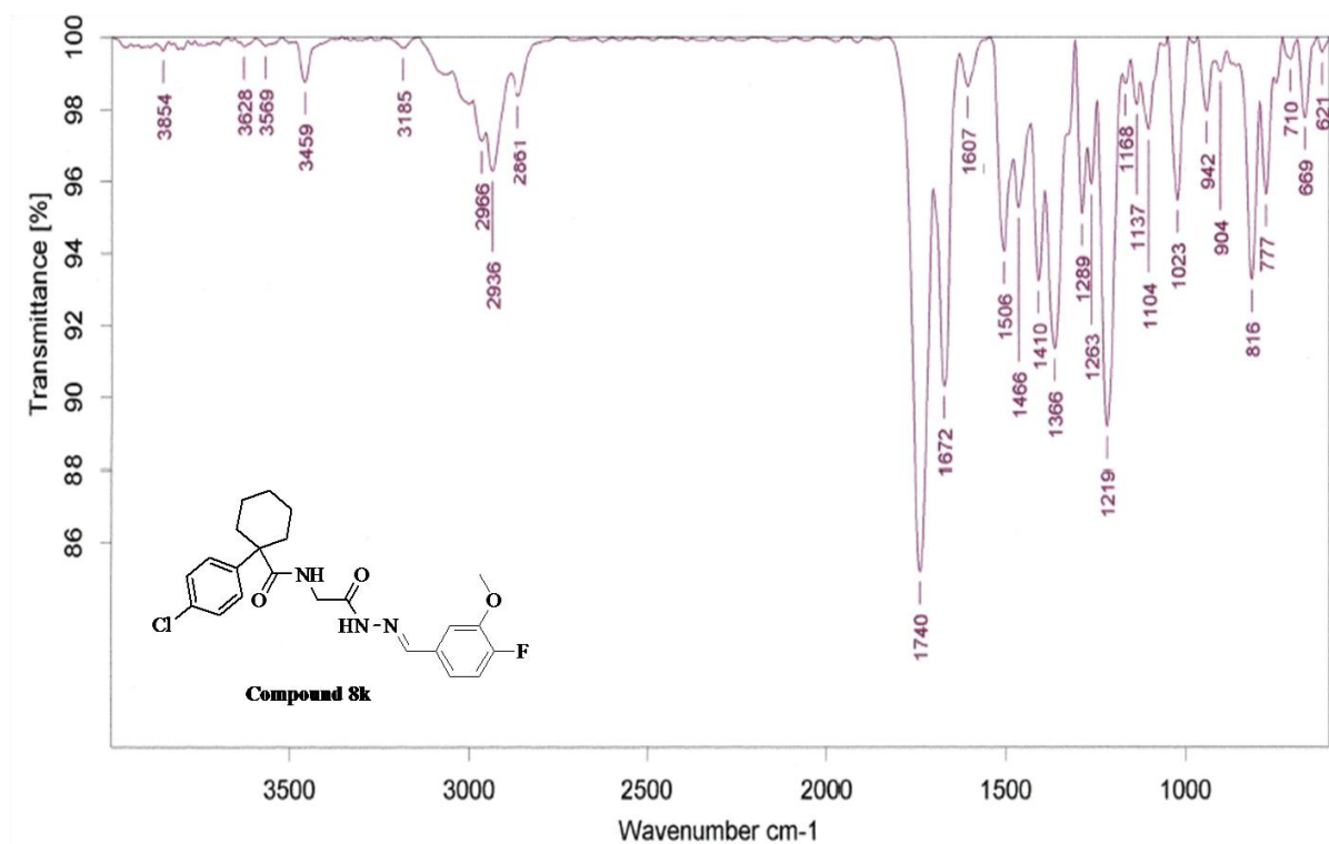
Figure S59: FT-IR spectrum of compound 8k
