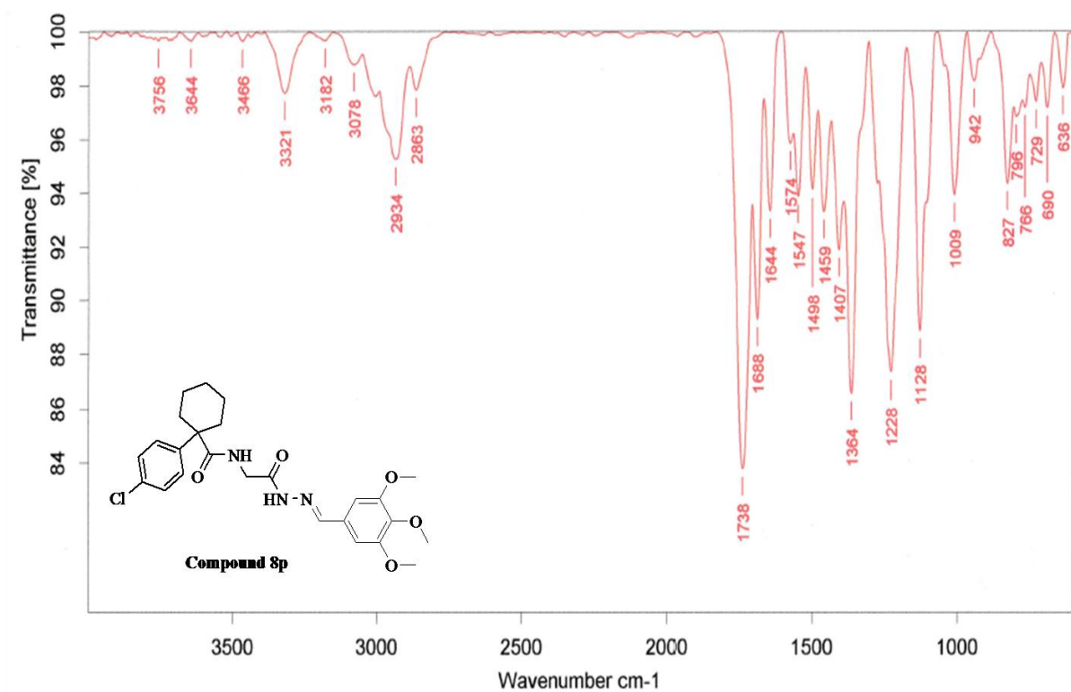
Figure S79: FT-IR spectrum of compound 8p
