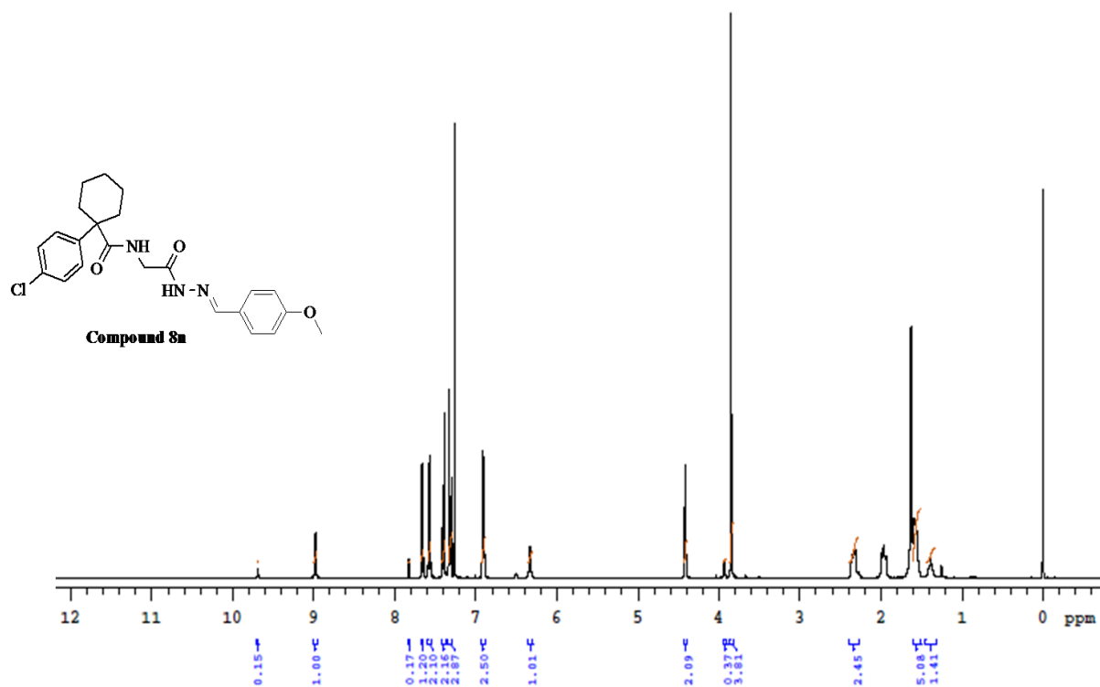
Figure S69: 1 H NMR spectrum of compound 8n
