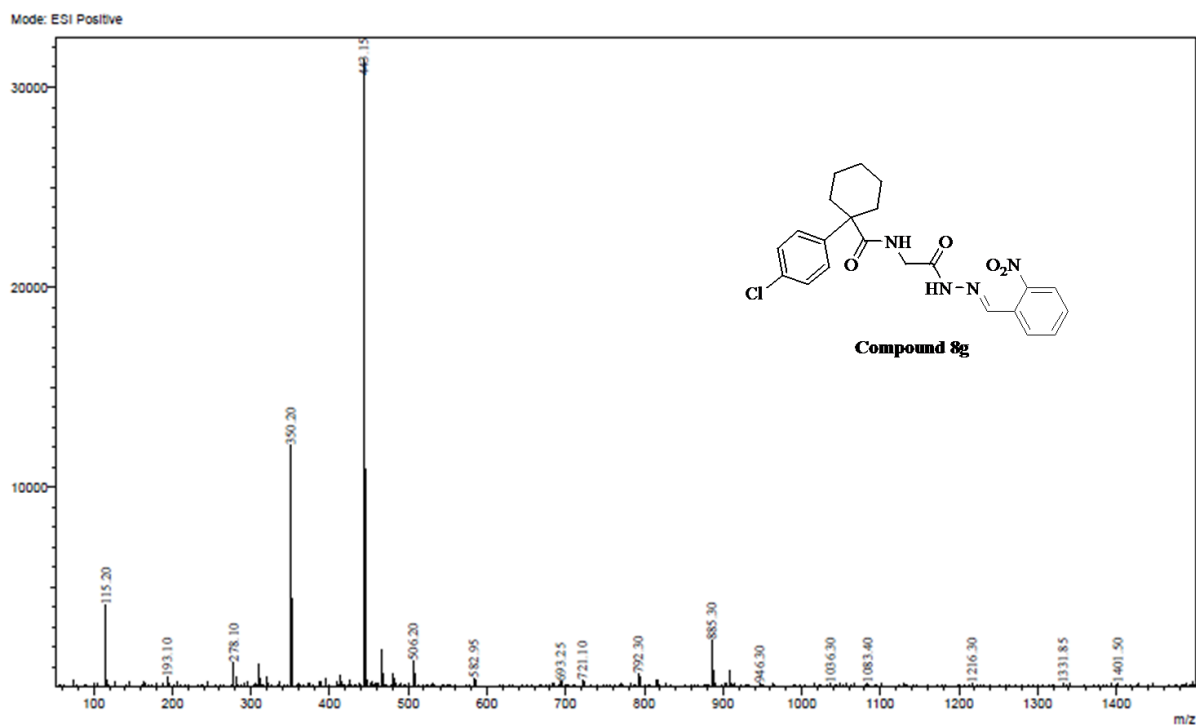
Figure S44: ESI-MS spectrum of compound 8g
