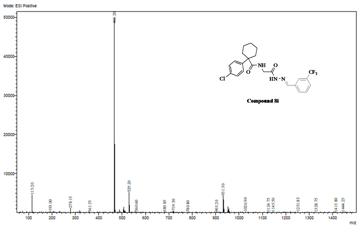
Figure S52: ESI-MS spectrum of compound 8i
