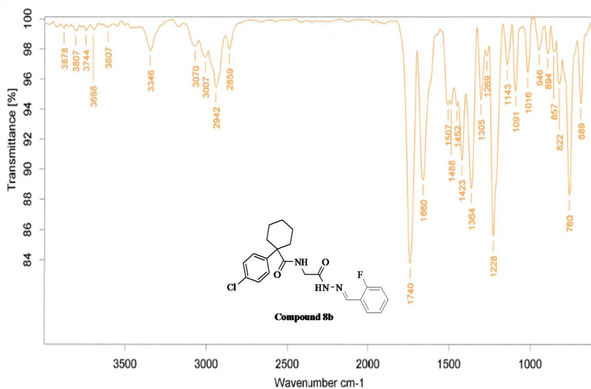
Figure S23: FT-IR spectrum of compound 8b
