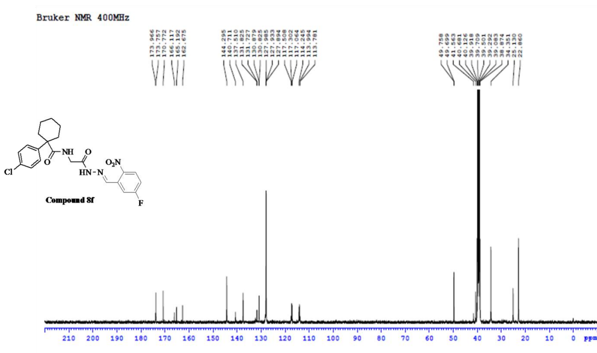
Figure S38: ^{13}\text{C} NMR spectrum of compound 8f
