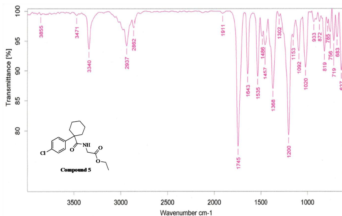
Figure S11: FT-IR spectrum of compound 5
