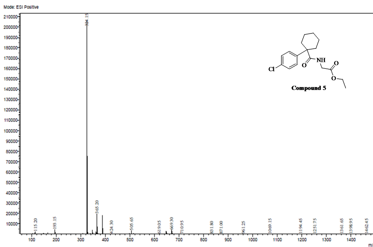
Figure S12: ESI-MS spectrum of compound 5
