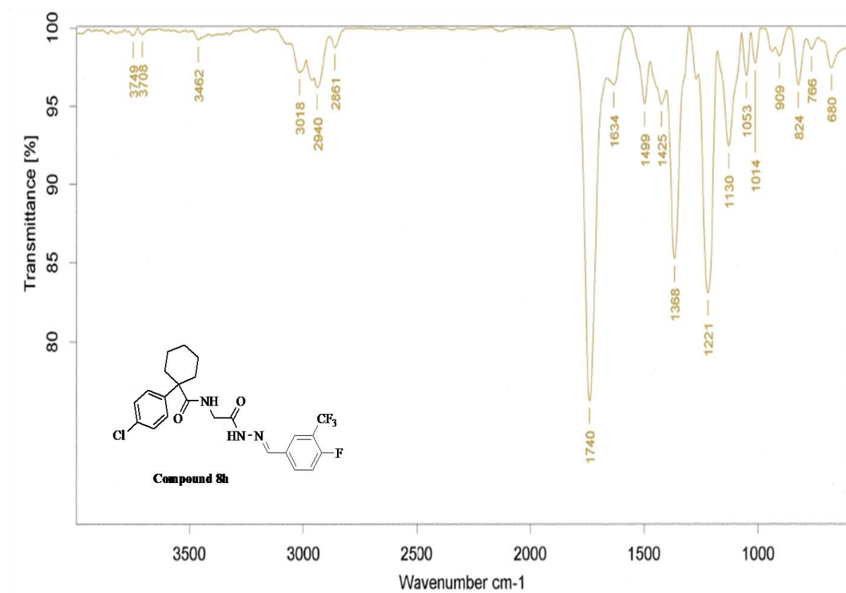
Figure S47: FT-IR spectrum of compound 8h
