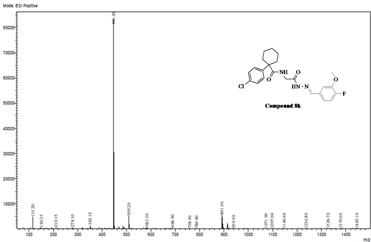
Figure S60: ESI-MS spectrum of compound 8k
