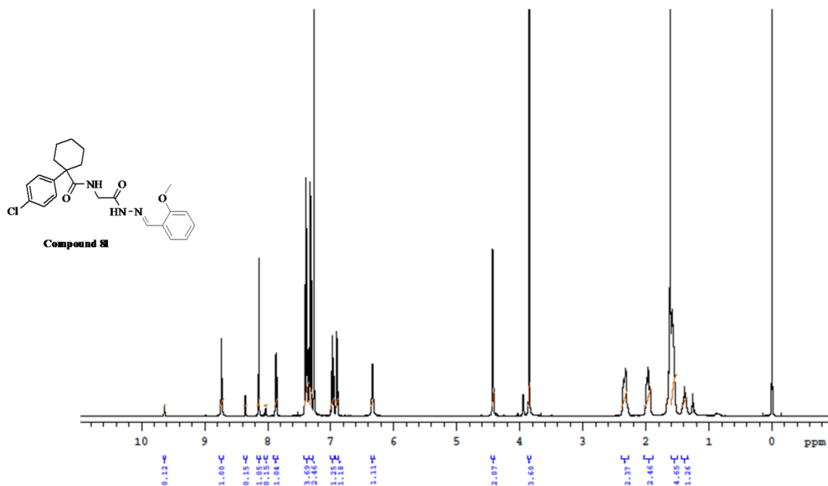
Figure S61: ^1\text{H} NMR spectrum of compound 8l
