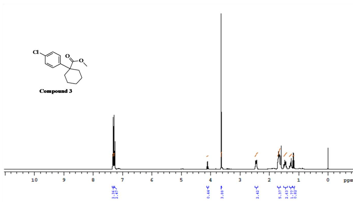
Figure S1: 1 H NMR spectrum of compound 3
