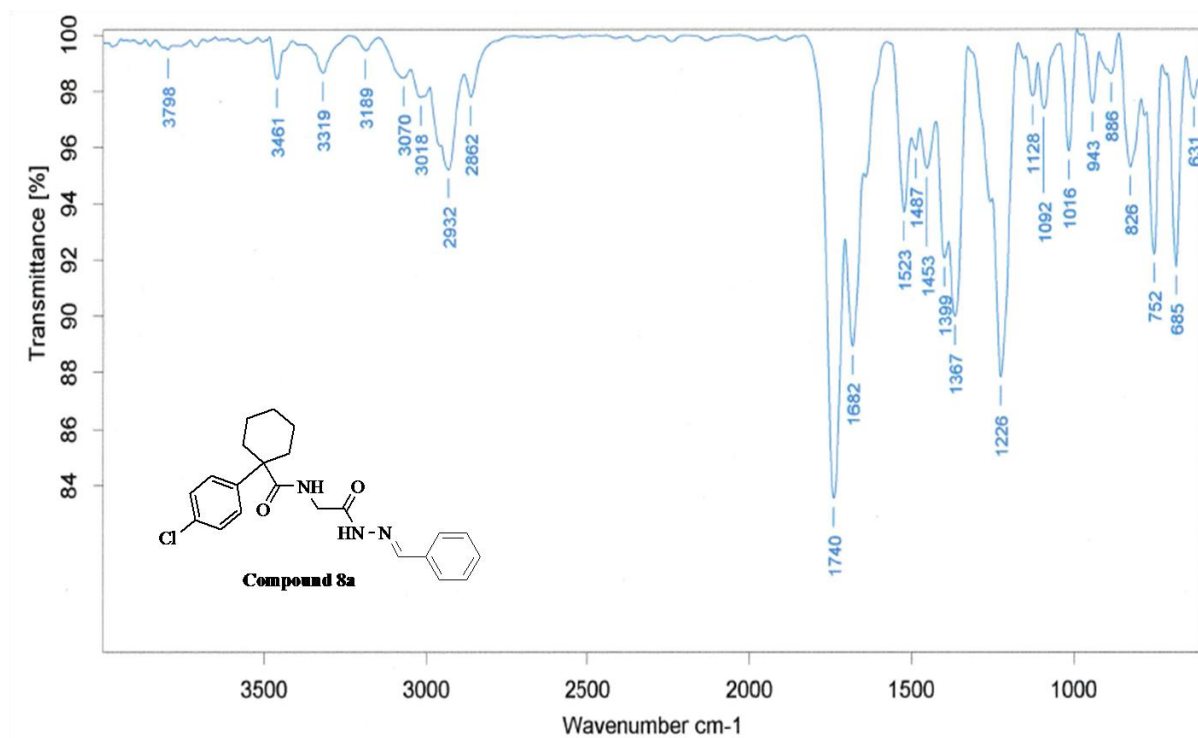
Figure S19: FT-IR spectrum of compound 8a
