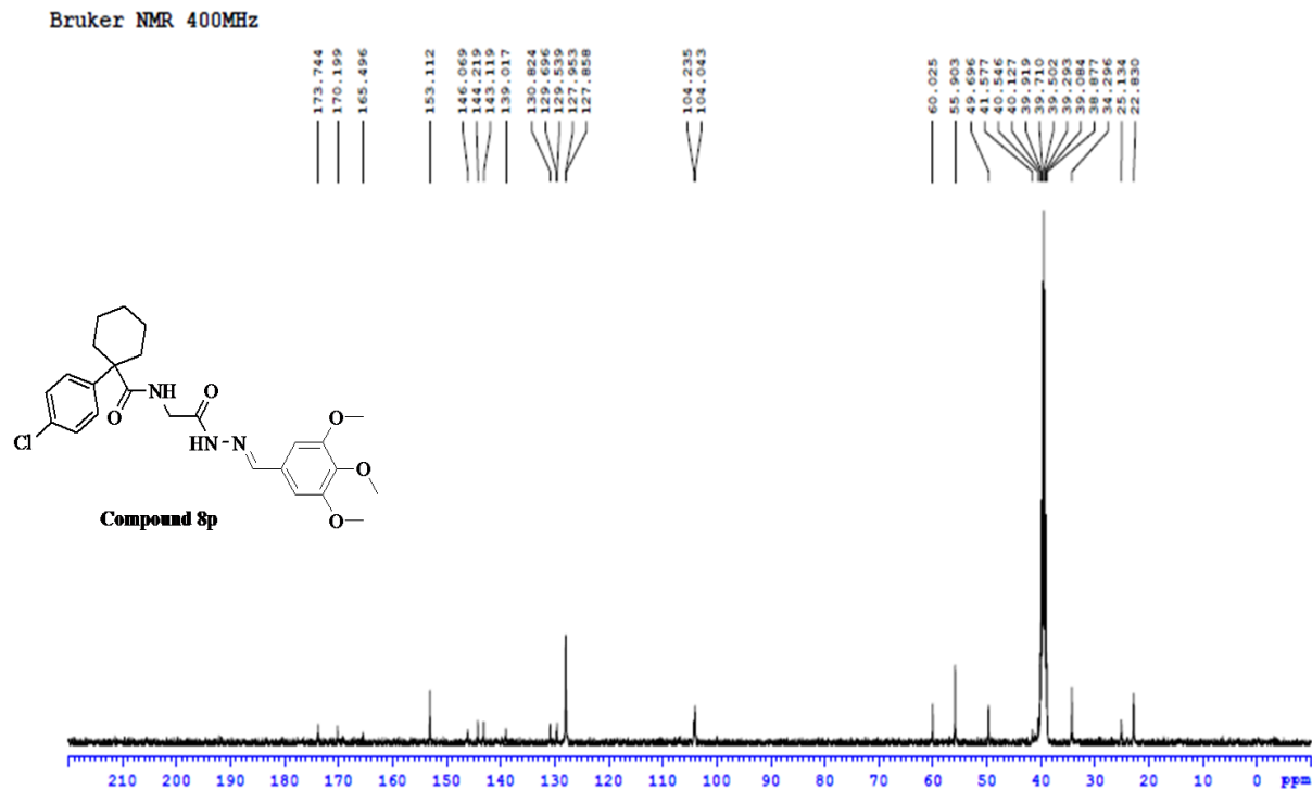
Figure S78: ^{13}\text{C} NMR spectrum of compound 8p
