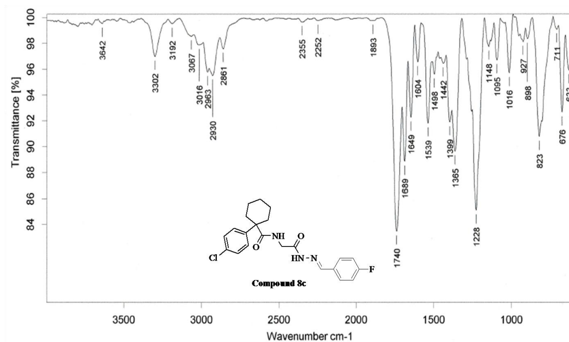
Figure S27: FT-IR spectrum of compound 8c
