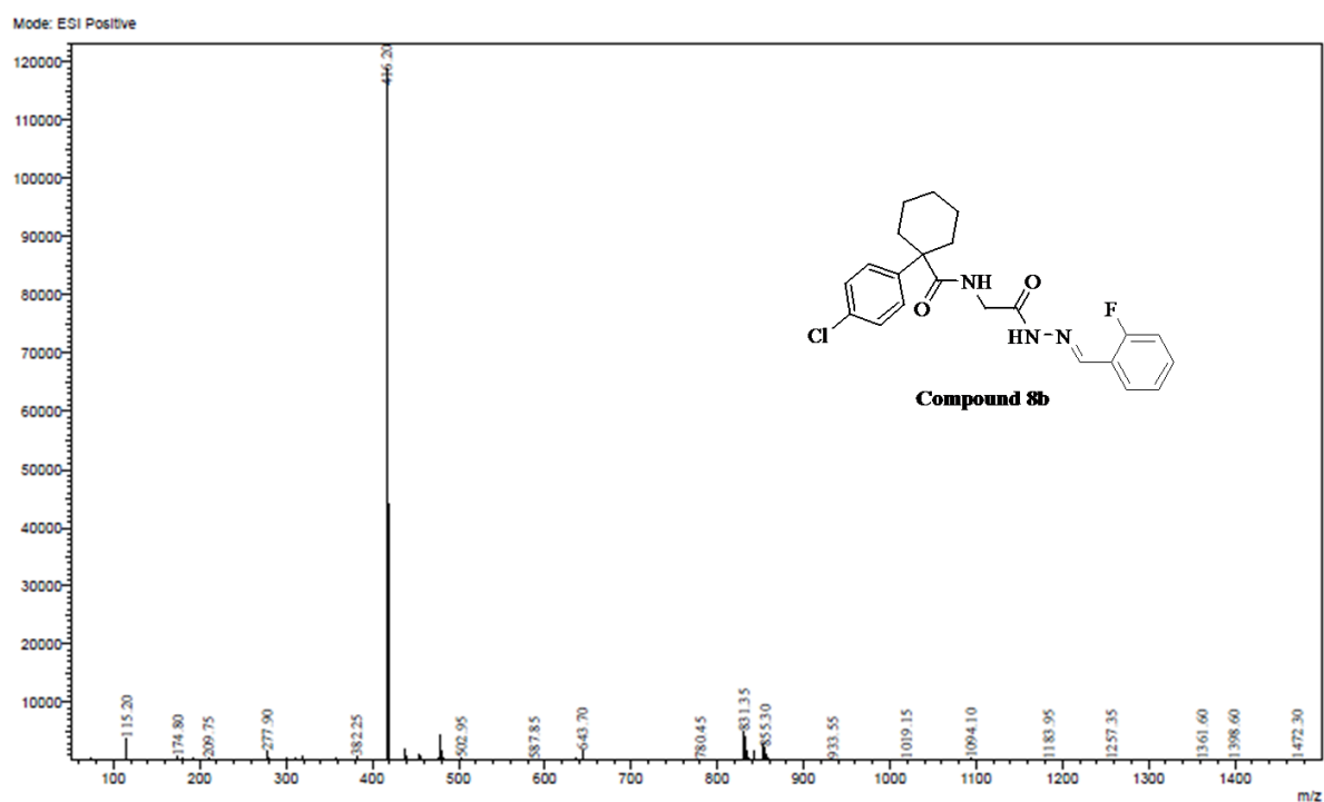
Figure S24: ESI-MS spectrum of compound 8b
