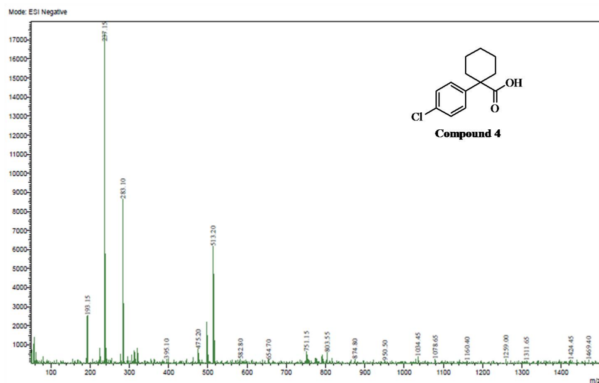
Figure S8: ESI-MS spectrum of compound 4
