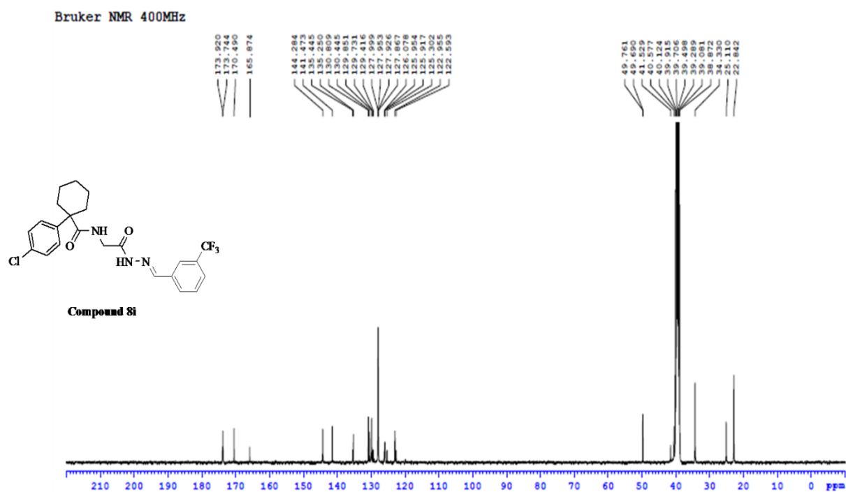
Figure S50: ^{13}\text{C} NMR spectrum of compound 8i
