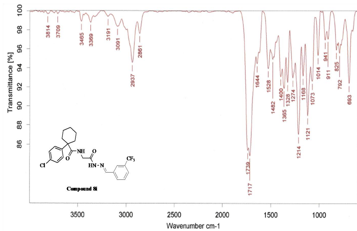
Figure S51: FT-IR spectrum of compound 8i
