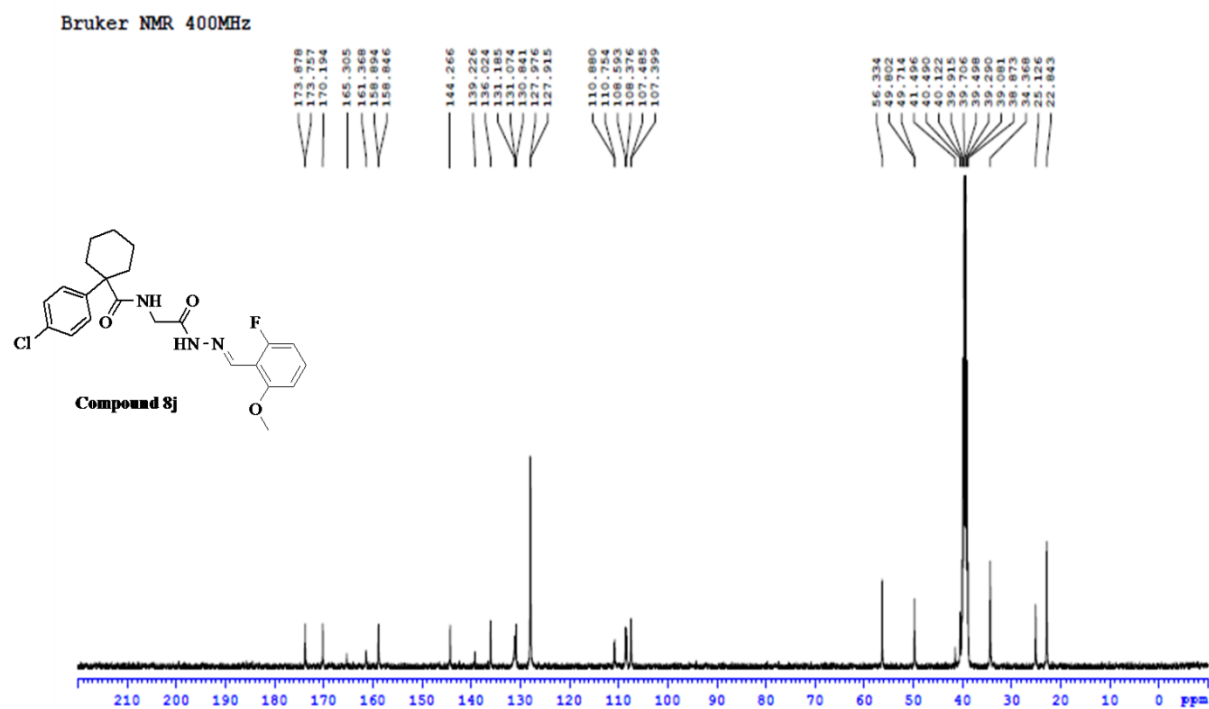
Figure S54: ^{13}\text{C} NMR spectrum of compound 8j
