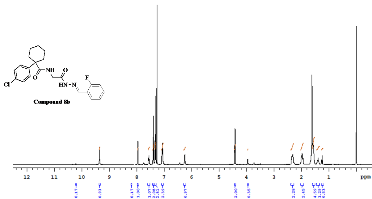
Figure S21: ^1\text{H} NMR spectrum of compound 8b
