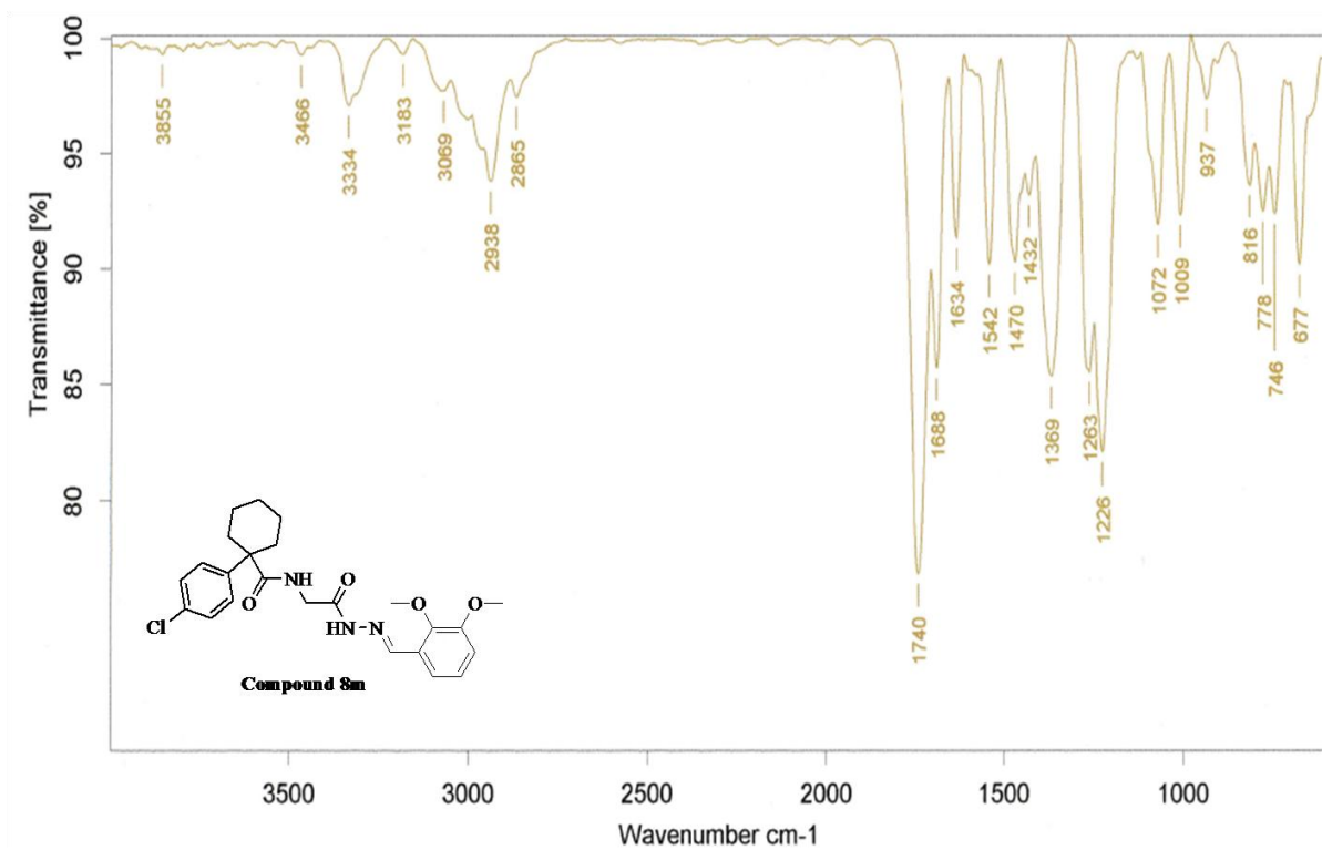
Figure S67: FT-IR spectrum of compound 8m
