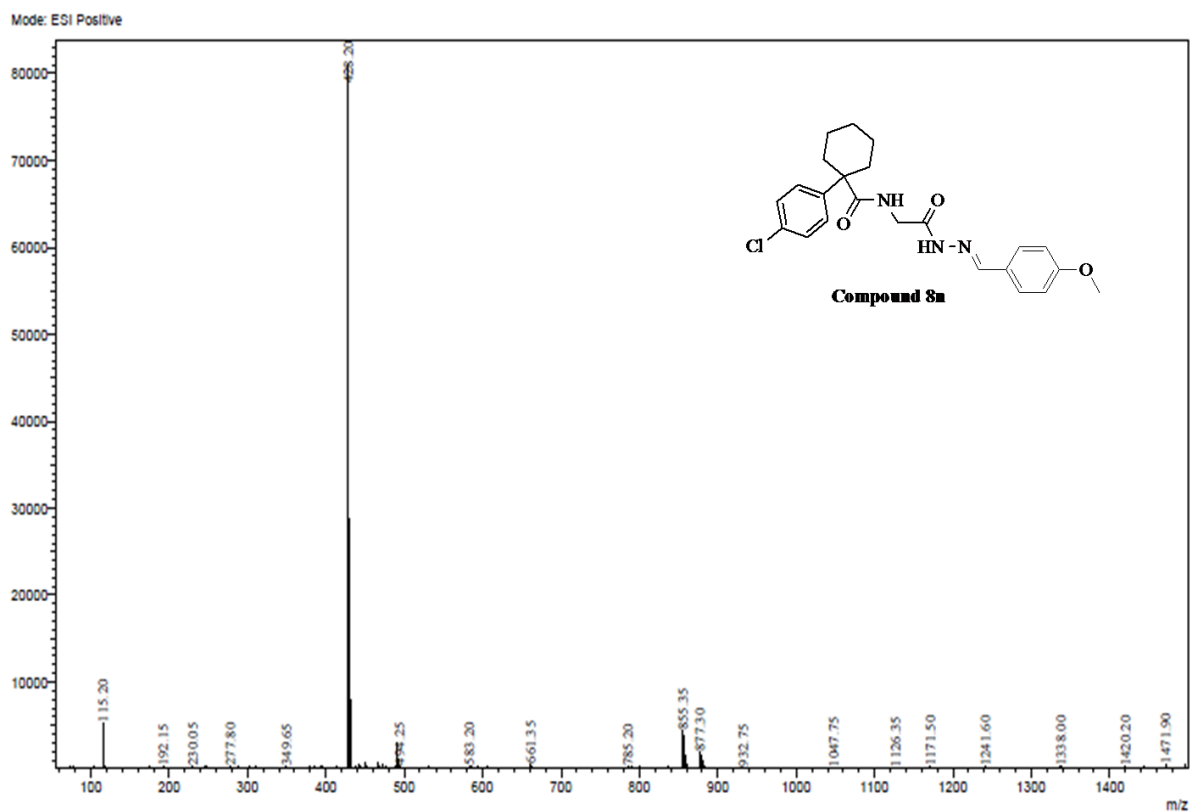
Figure S72: ESI-MS spectrum of compound 8n
