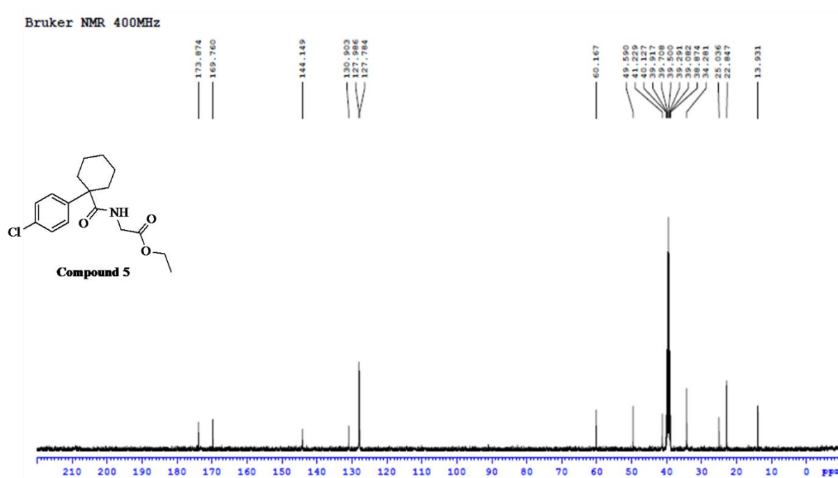
Figure S10: 13 C NMR spectrum of compound 5
