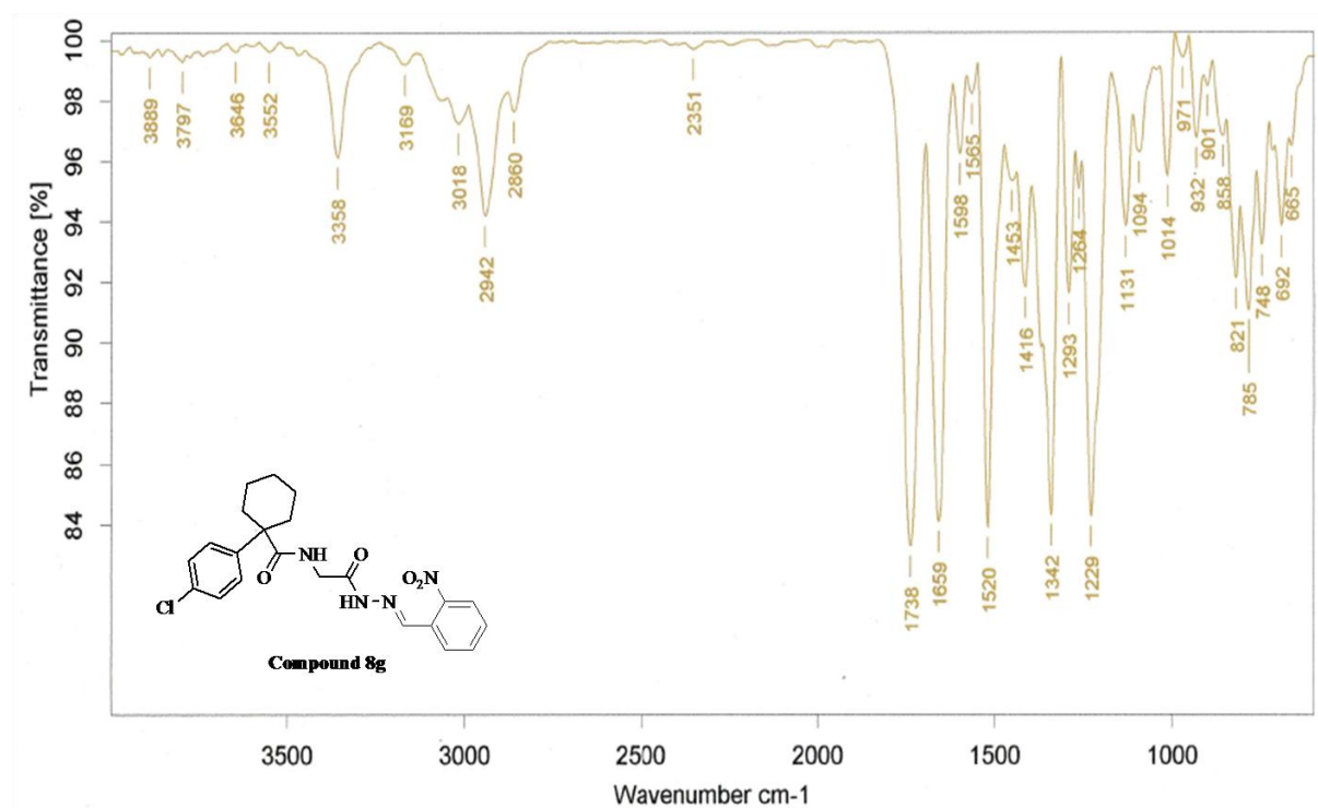
Figure S43: FT-IR spectrum of compound 8g
