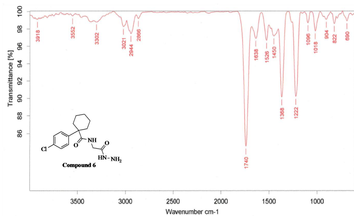
Figure S15: FT-IR spectrum of compound 6
