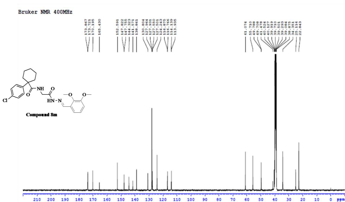
Figure S66: 13 C NMR spectrum of compound 8m
