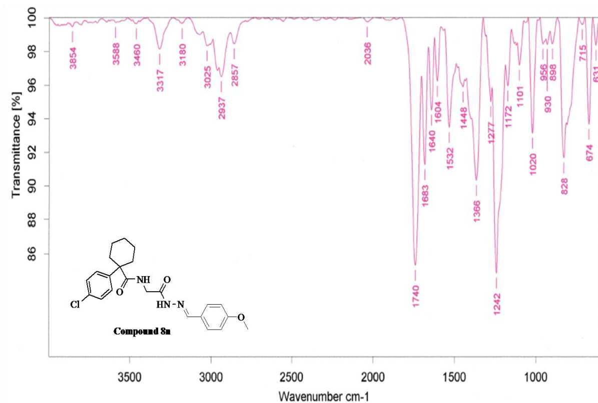
Figure S71: FT-IR spectrum of compound 8n
