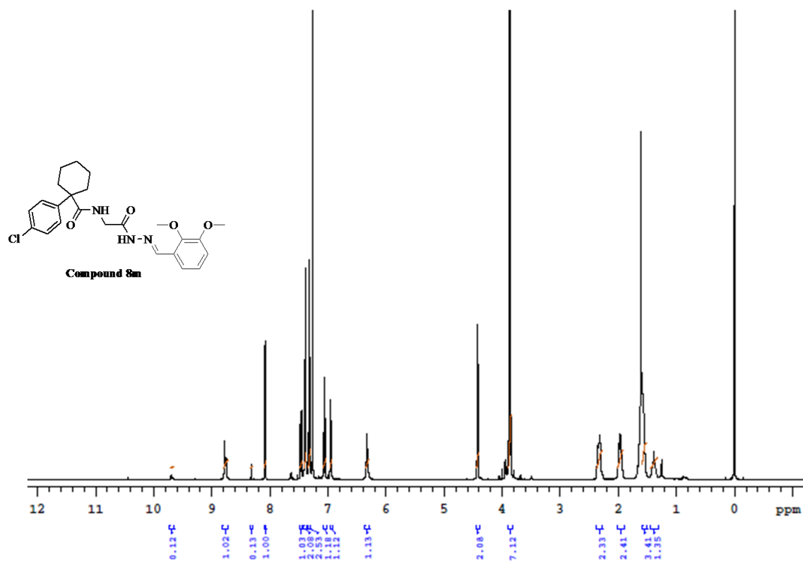
Figure S65: 1 H NMR spectrum of compound 8m
