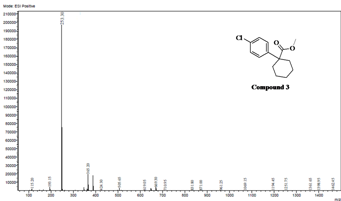
Figure S4: ESI-MS spectrum of compound 3
