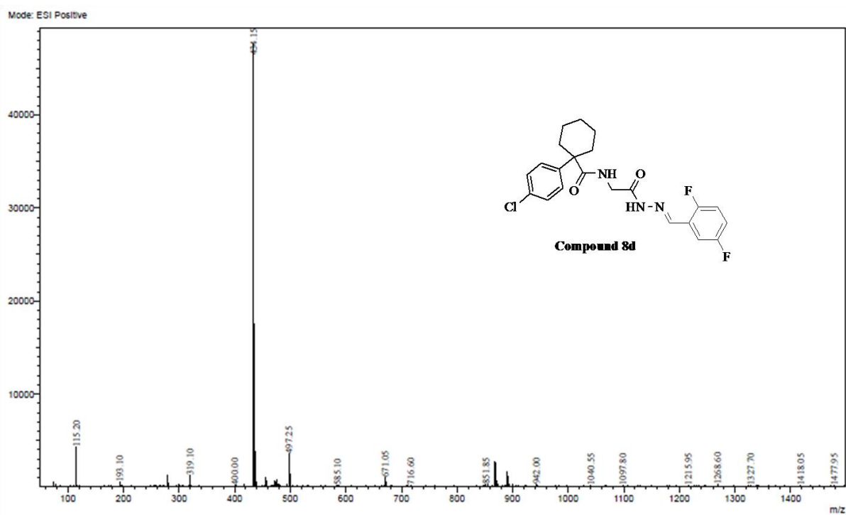
Figure S32: ESI-MS spectrum of compound 8d
