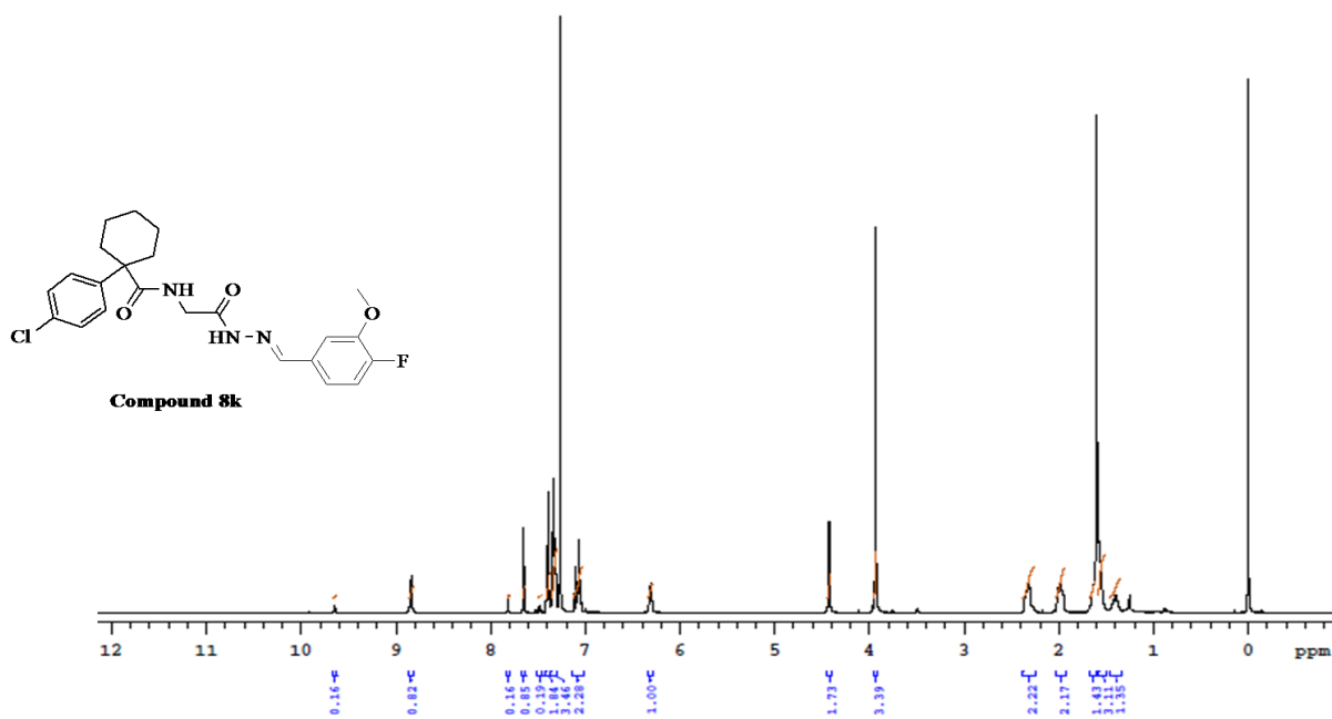
Figure S57: ^1\text{H} NMR spectrum of compound 8k
