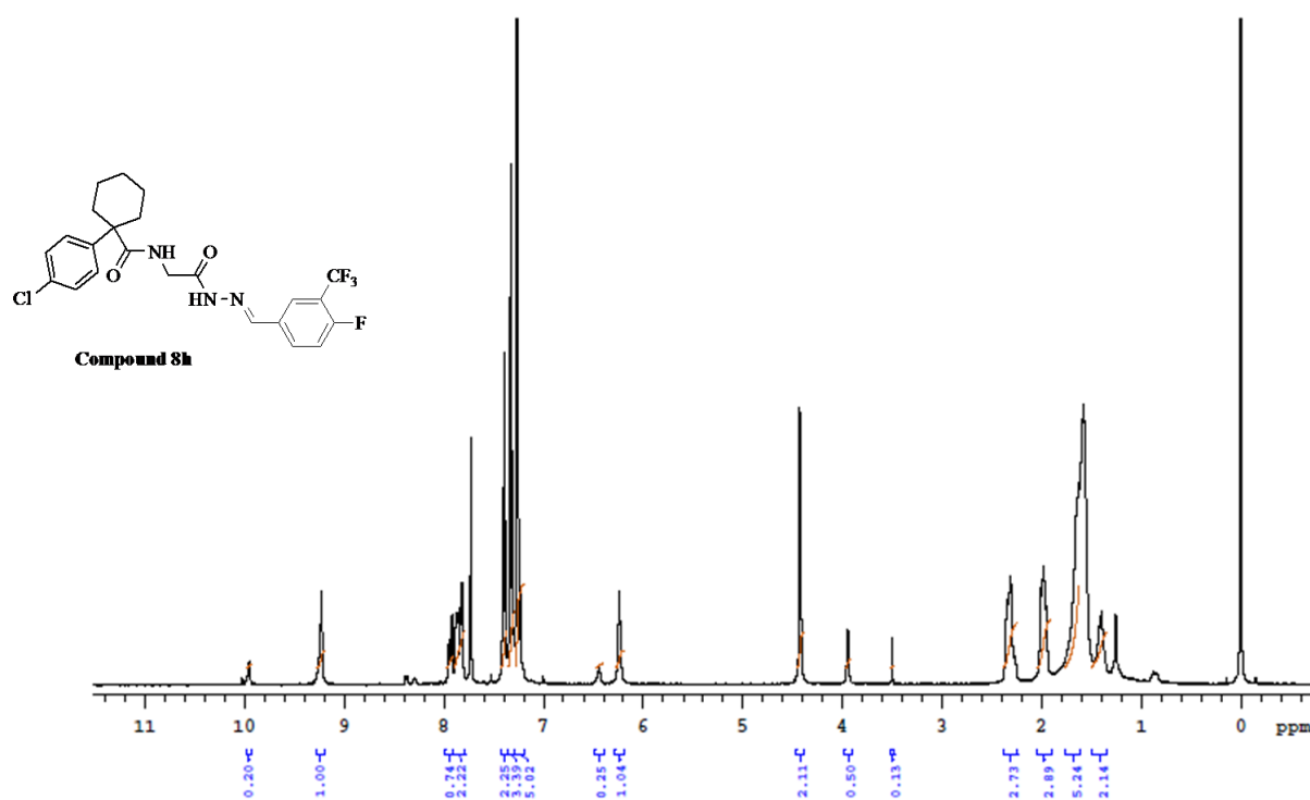
Figure S45: ^1\text{H} NMR spectrum of compound 8h
