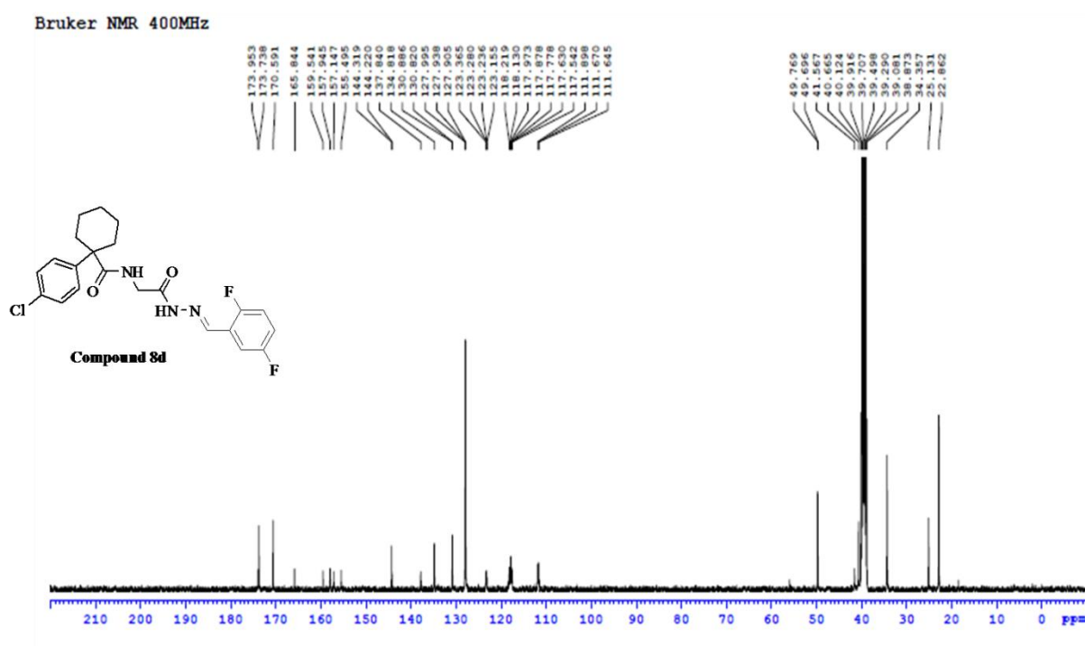
Figure S30: ^{13}\text{C} NMR spectrum of compound 8d
