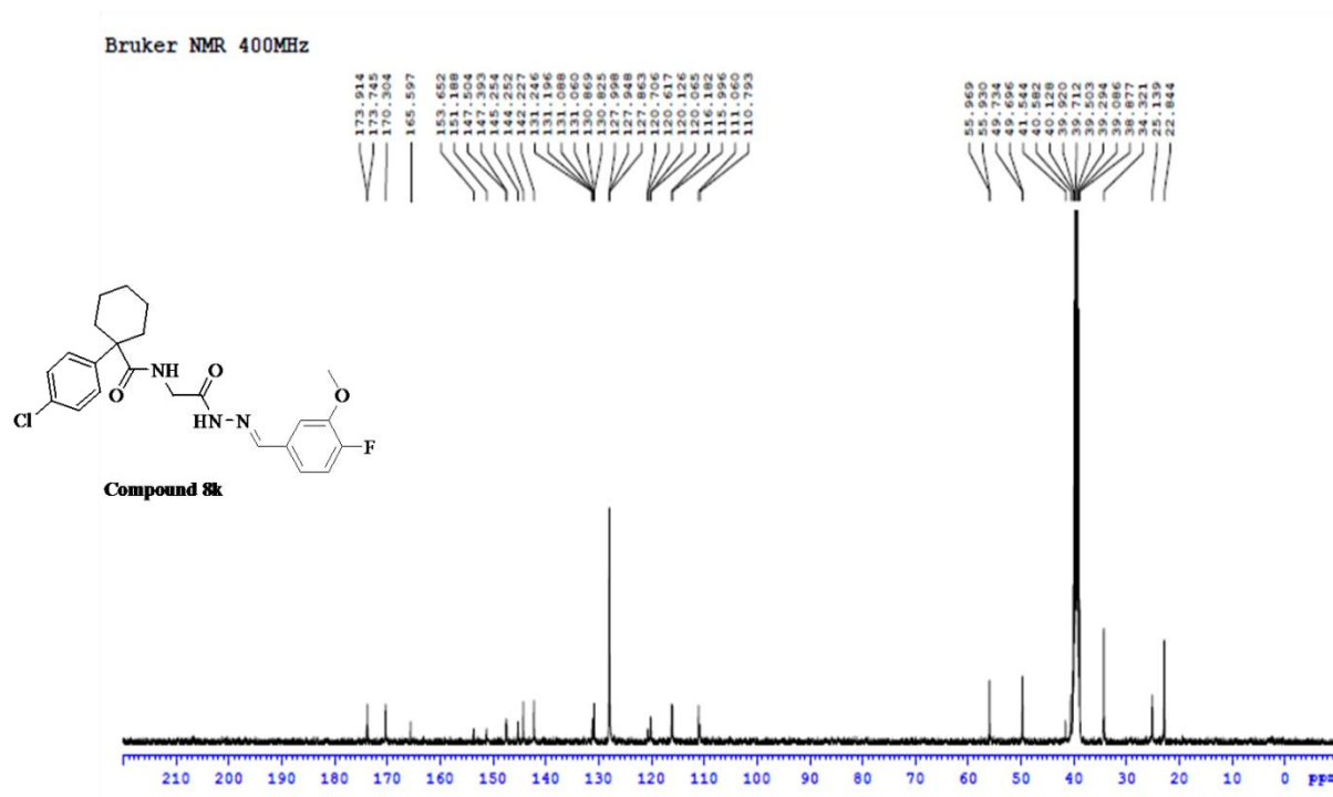
Figure S58: ^{13}\text{C} NMR spectrum of compound 8k
