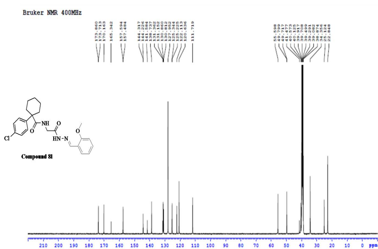
Figure S62: ^{13}\text{C} NMR spectrum of compound 8I
