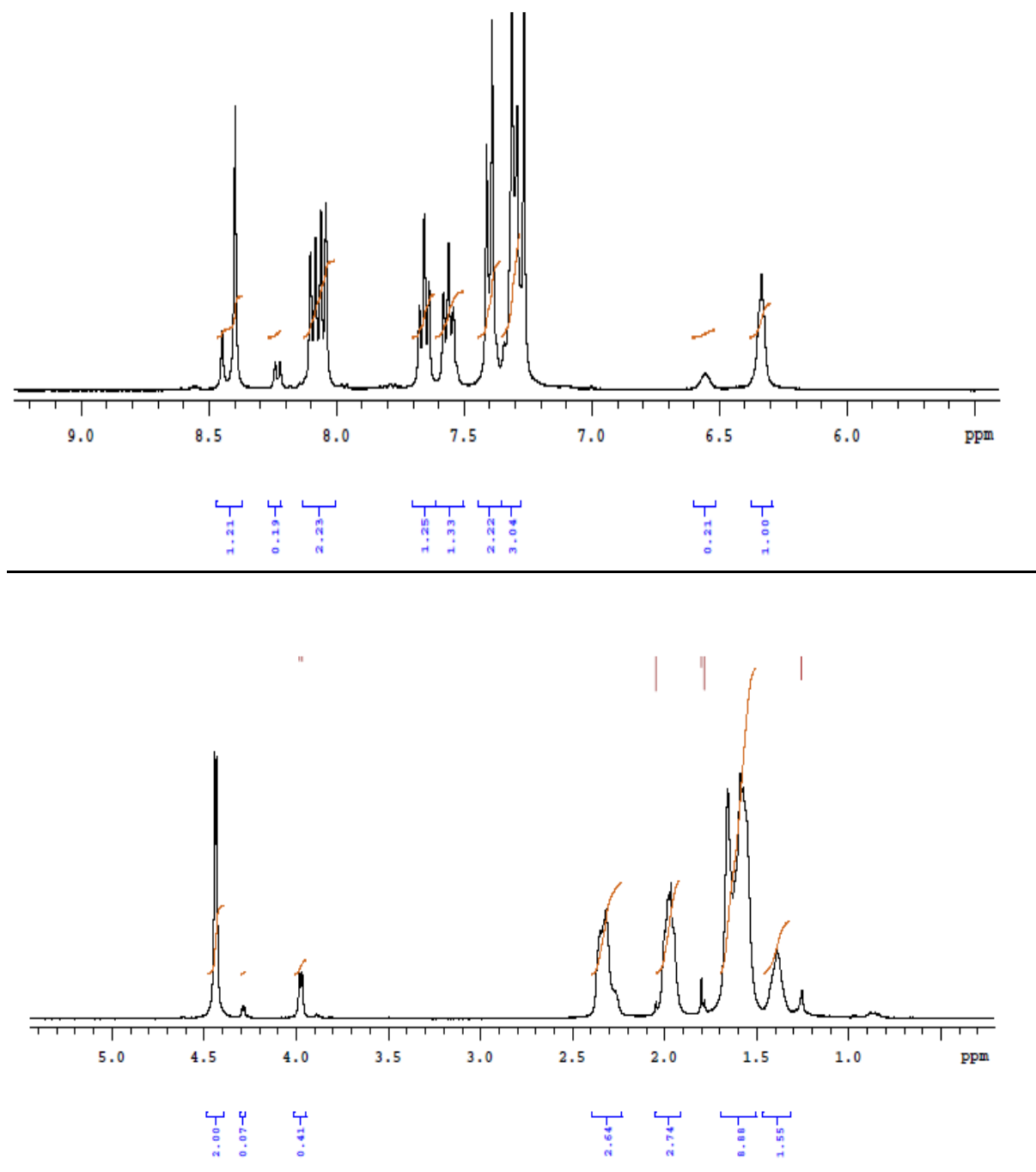
Figure S41: ^1\text{H} NMR spectrum of compound 8g
