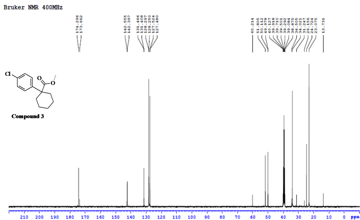
Figure S2: 13 C NMR spectrum of compound 3
