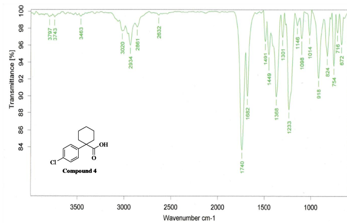
Figure S7: FT-IR spectrum of compound 4
