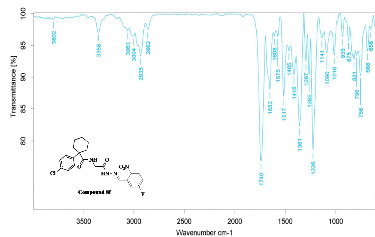
Figure S39: FT-IR spectrum of compound 8f
